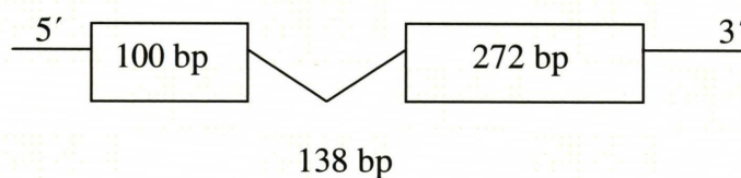
Figure 3.1: Genomic organization of the AtPNP-B encoding gene from Arabidopsis thaliana . (a) DNA sequence of AtPNP-B with the intron region indicated in red. (b) Schematic representation of the AtPNP-B gene.
