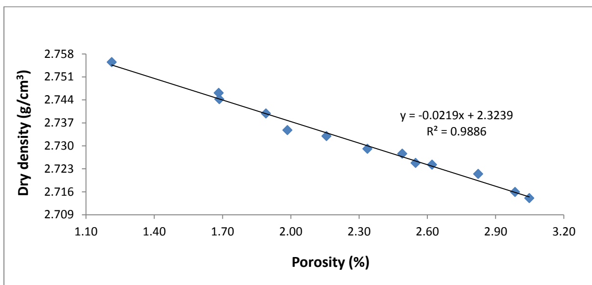
Figure C20 Dry density - porosity relationship for the Middleton Formation.
