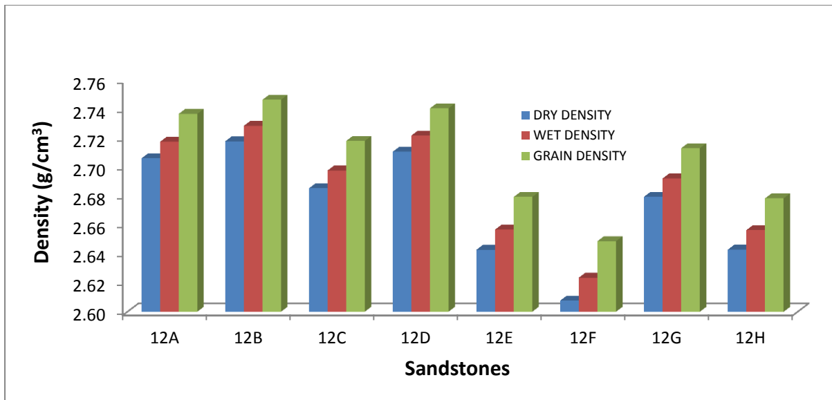
Figure C27 Bar chart of dry, wet and grain densities for the Elandsberg Member.
