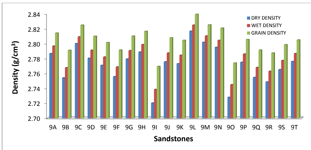
Figure C21 Bar chart of dry, wet and grain densities for the Oudeberg Member.
