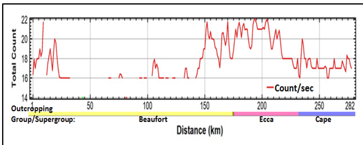
Figure 6.6 Profile for total gamma radiation count rate along Line B - B'.
