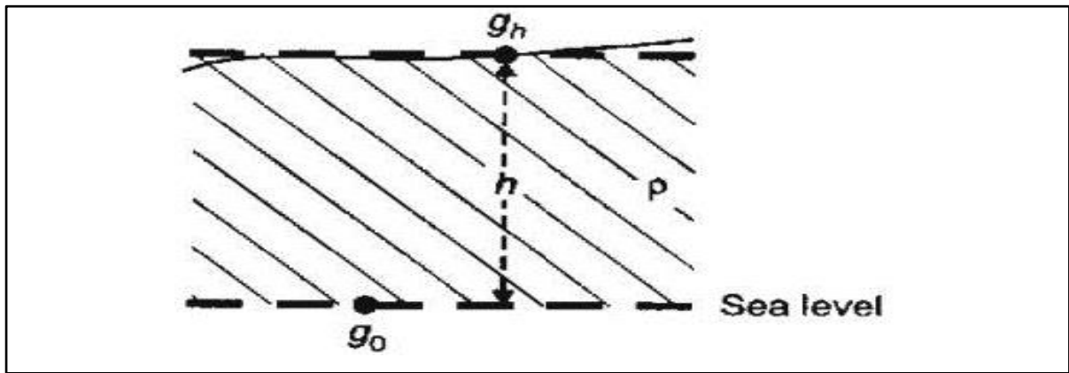
Figure C4 Schematic representation of Bouguer correction (Reeves, 2005).
