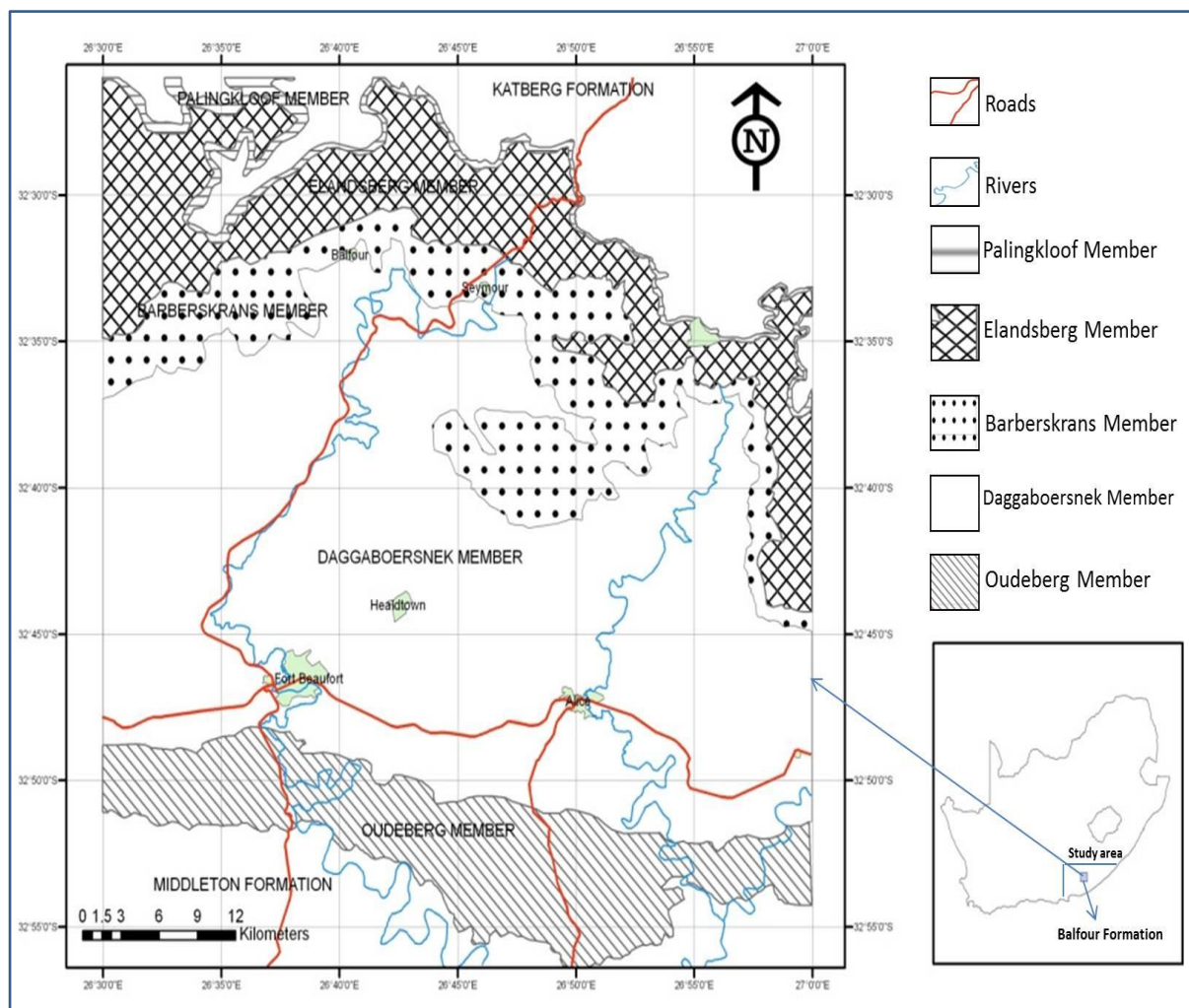
Figure 4.23 Map showing the distribution of sediments of the Oudeberg, Daggaboersnek, Barberskrans, Elandsberg, and Palingkloof Members of the Balfour Formation (Modified by author from Katemaunzanga and Gunter, 2009).
