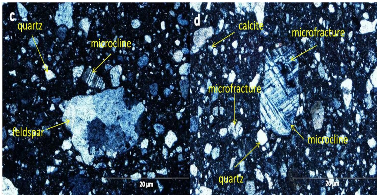
Figure 4.37 (c) Fine- to medium- grained clast population with angular - sub-rounded plagioclase, microcline and quartz. (d) Microfractures at some contact between the mineral grains.
