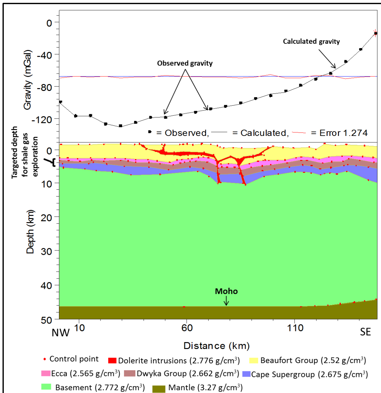
Figure 8.10 Gravity modelling of profile G – G'. VE = 1.09, Initial and final RMS errors are 61.843 and 1.274, respectively.
