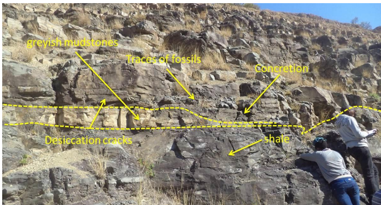
Figure 4.29 Photograph of the Palingkloof Member, near Queenstown showing greyish mudstones with subordinate shale as well as dessication cracks, concretions and traces of fossils (Elevation: 483 m; Longitude E 26° 46' 54.4"; Latitude S 32° 28' 56").
