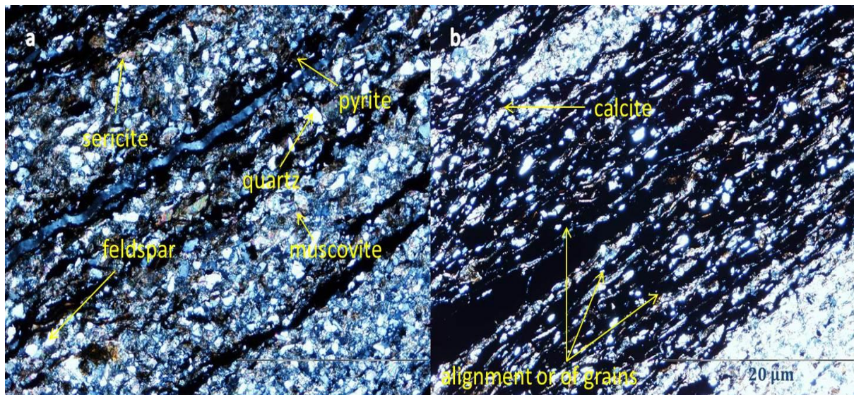
Figure 4.38 Photomicrographs of shales from Prince Albert Formation along the Eccia Pass. (a) Detrital grains of micas (occasionally deformed), quartz, feldspar, sericite (golden colour) and pyrite. (b) Alignment or orientation of grains, recrystallized euhedral calcite (yellowish colour).
