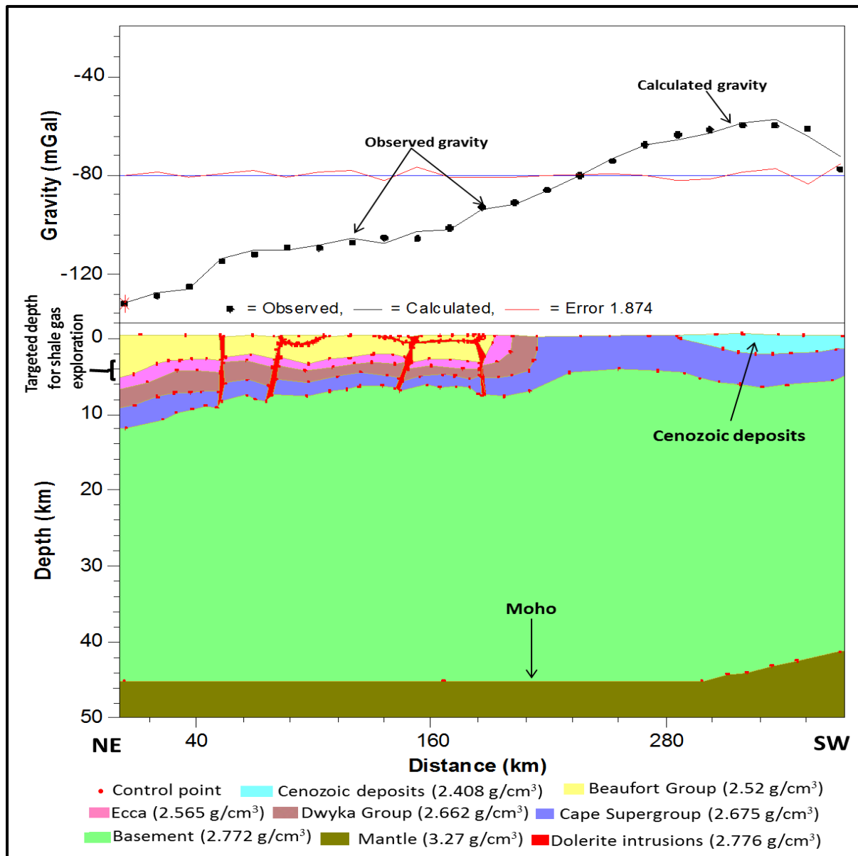
Figure 8.6 Gravity modelling of profile C - C'. VE = 1.82, Initial and final RMS errors are 82.623 and 1.874, respectively. Note: When the black curve (calculated gravity) matches with the black dots (observed gravity), it indicates a perfect fit with minimum error.
