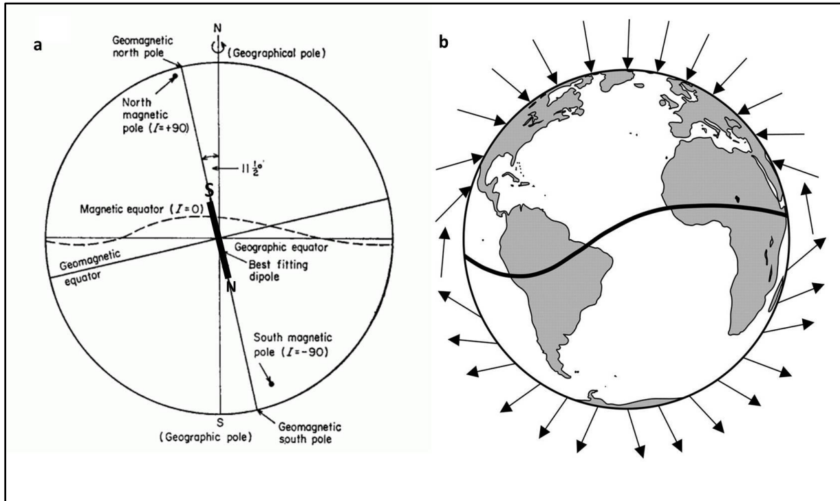
Figure 5.1 The field due to an inclined geocentric dipole and the field lines (Reeves, 2005). Note that the geomagnetic South pole is a magnetic North pole and the geomagnetic North pole is a magnetic south pole.
