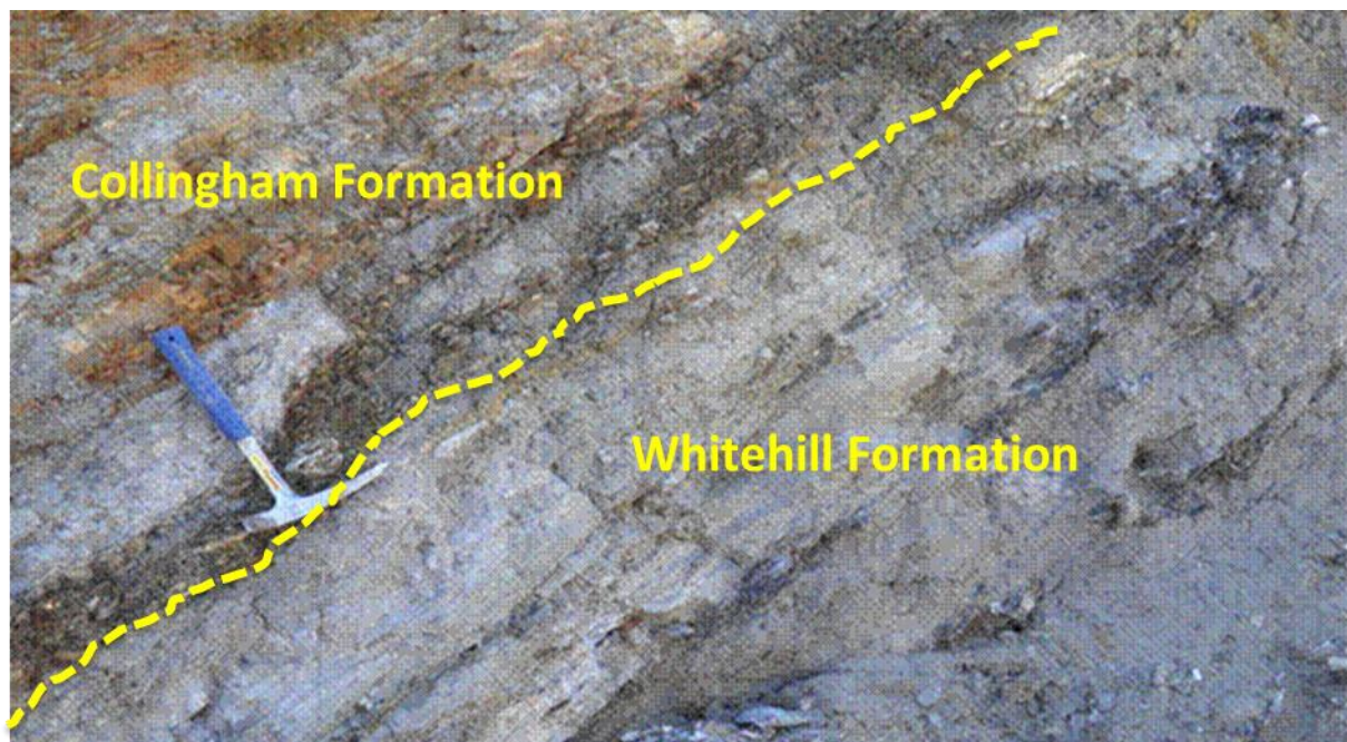
Figure 4.12 Photograph showing conformable contact between the Whitehill Formation and the Collingham Formation along the Eccle Pass.
