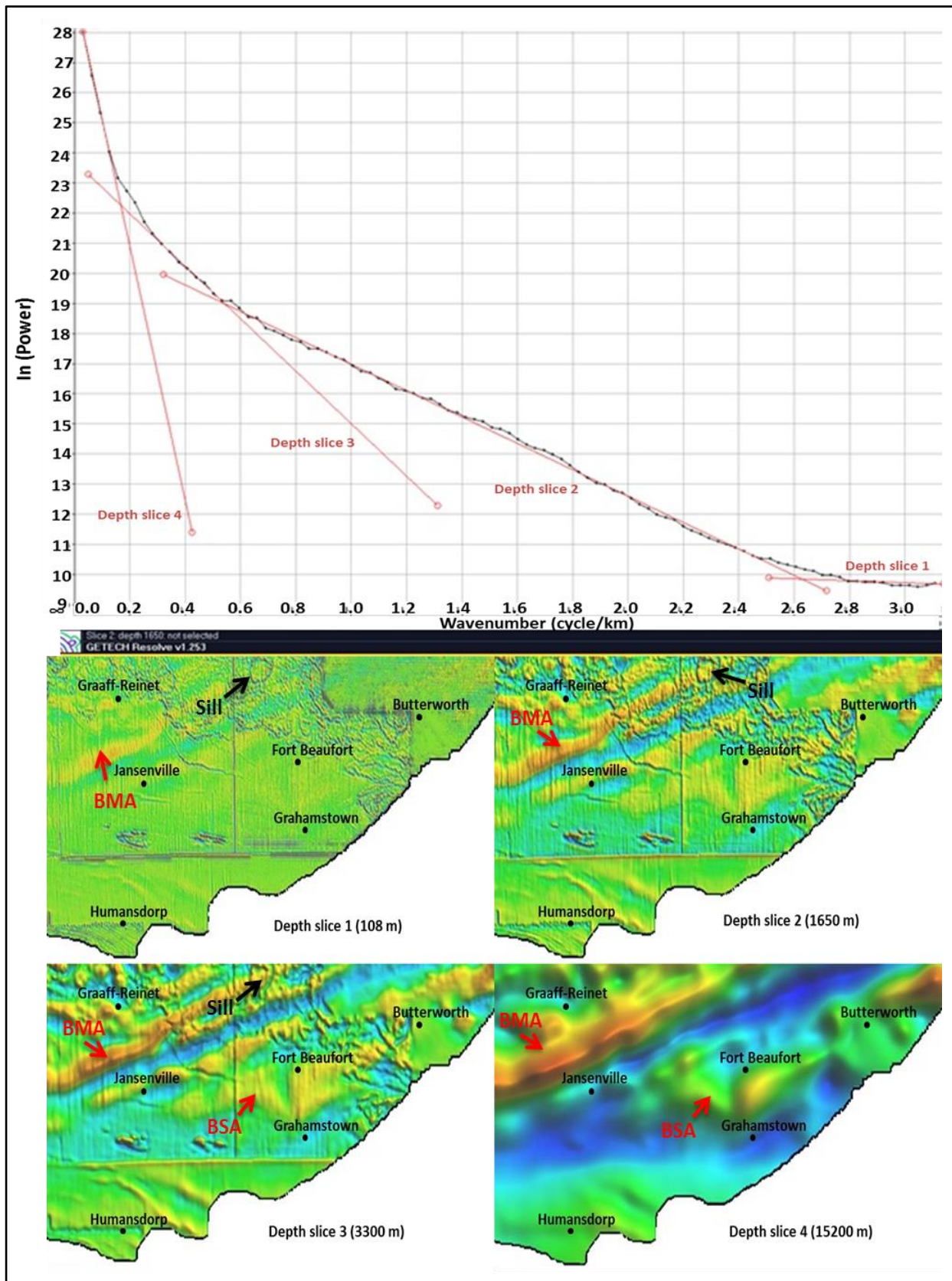
Figure 5.10 Depth slice showing changes in anomaly features with depth. Note: BMA is the Beattie Magnetic anomaly and BSA is the bean shape anomaly.
