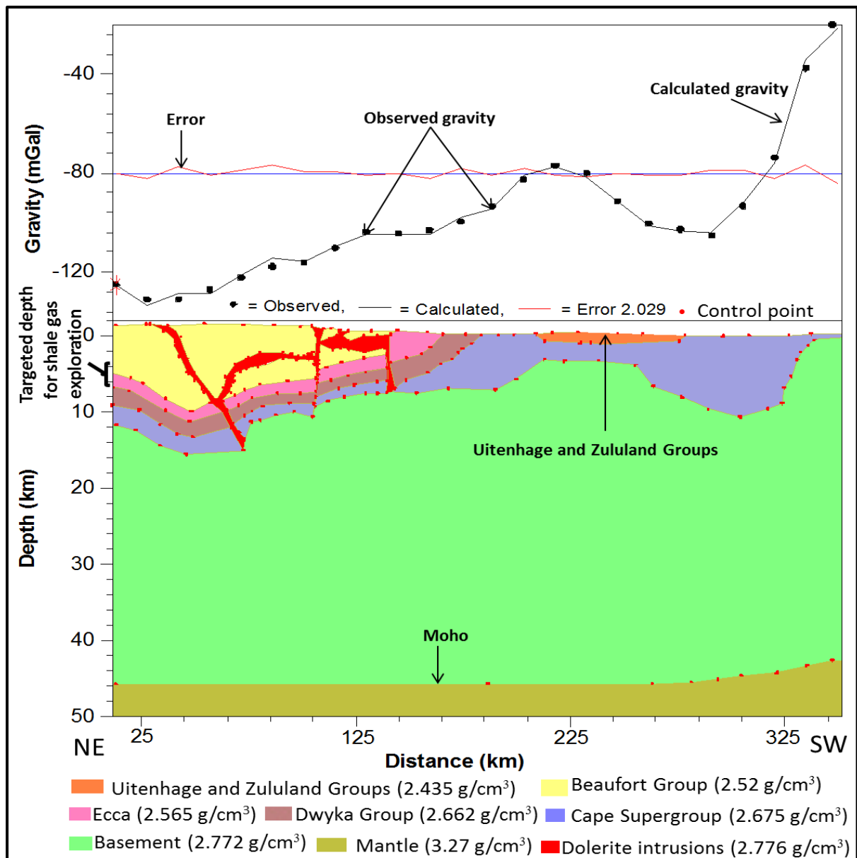
Figure 8.5 Gravity modelling of profile B – B'. VE = 1.98, Initial and final RMS errors are 61.705 and 2.029, respectively. Note: When the black curve (calculated gravity) matches with the black dots (observed gravity), it indicates a perfect fit with minimum error.
