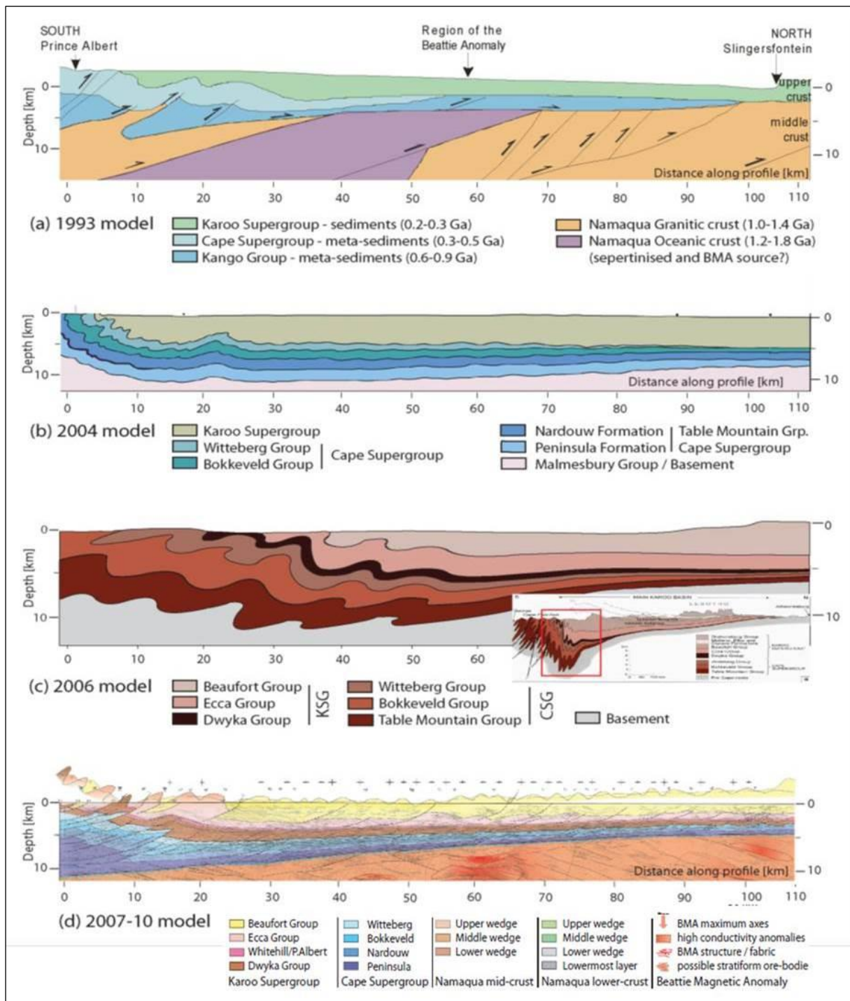
Figure 2.6 Comparing models of the Cape and Karoo Basins in the upper crust (< 15 km). (a) Hällich et al. (1993) model: Ophiolite wedge/serpentinised palaeoceanic crust as the possible source of BMA. (b) Chevallier et al. (2004) model: Karoo Supergroup undifferentiated. (c) Johnson, et al. (2006) model: Close-up from the regional model. (d) 2007- 2010 model: these models show intense folding, deepening and thickening of the Karoo Supergroup before the Cape Fold Belt which was interpreted as a fore-deep basin (Taken directly from Lindeque et al. , 2011).
