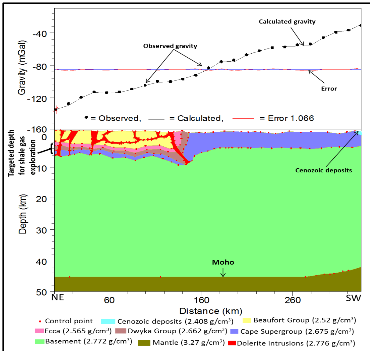
Figure 8.14 Gravity modelling of profile K - K'. VE = 1.97, Initial and final RMS errors are 58.466 and 1.066, respectively. Note: The modelled dolerite sills and dykes were originally set in horizontal and vertical positions, respectively and allowed to vary or change during the modelling process in order to have the best fit model.
