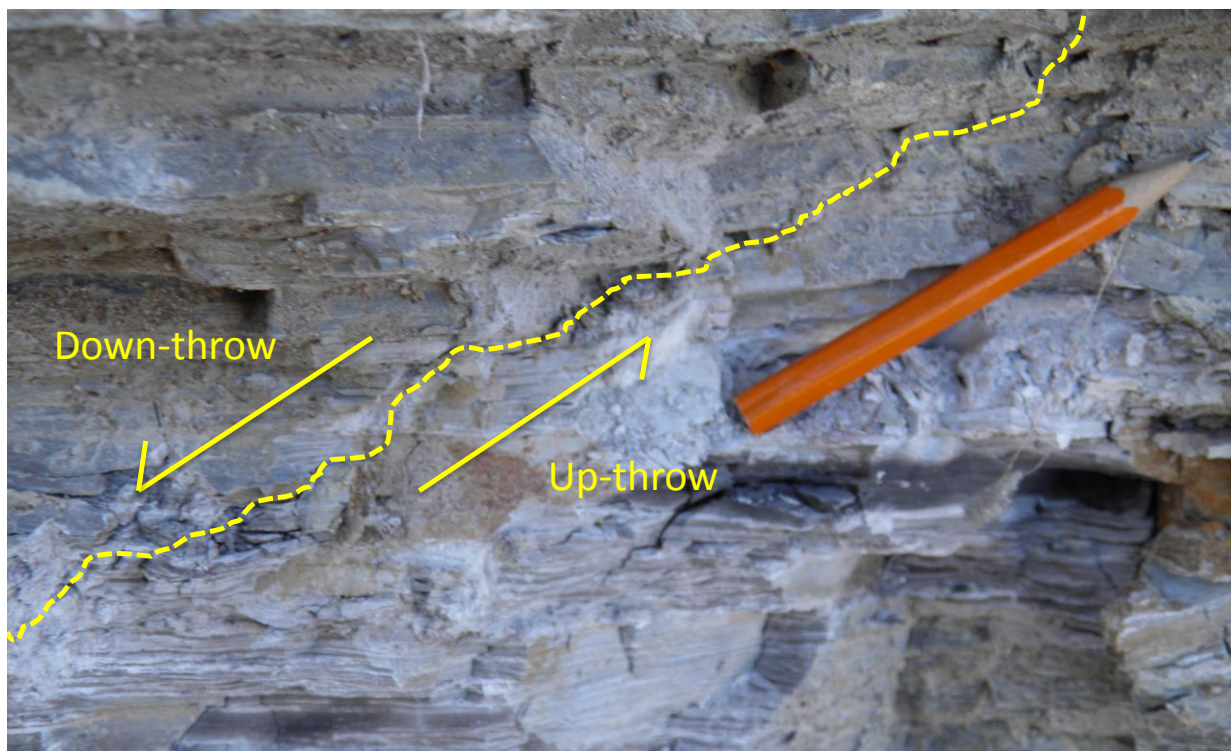
Figure 4.11 Photograph showing a normal fault cutting through the Whitehill Formation, thus dividing it into two layers which lie side by side.
