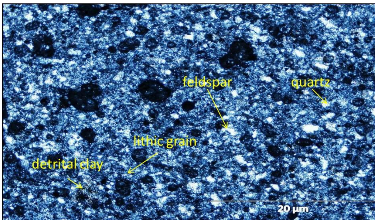
Figure 4.46 Photomicrographs of sandstones from Katberg Formation showing feldspar, quartz, detrital clay and lithic grains.
