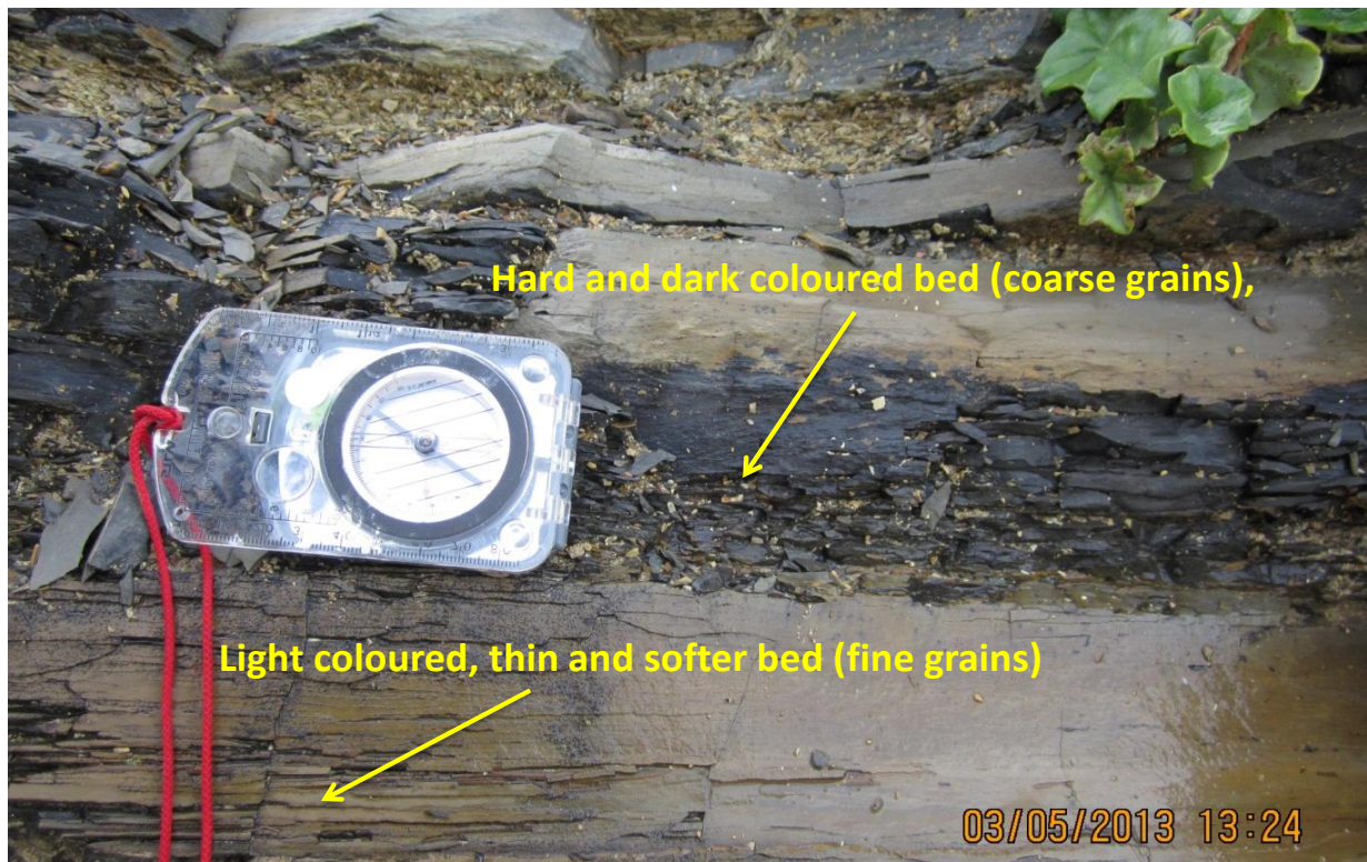
Figure 4.14 Well developed horizontal rhythmite of claystone (soft and light beds) interbedded with the mudstones (hard and dark coloured beds) of the Collingham Formation (Elevation: 471 m; Longitude E 26° 37' 35.7"; Latitude S 33° 12' 56.0"). The claystone easily crumbles than the mudstones. Lamination structures can be seen in the finer mudstones. Micro-ripple lamination appeared in the relative coarser and thicker mudstone layers, which is a typical sedimentary structure for turbidite sediments.
