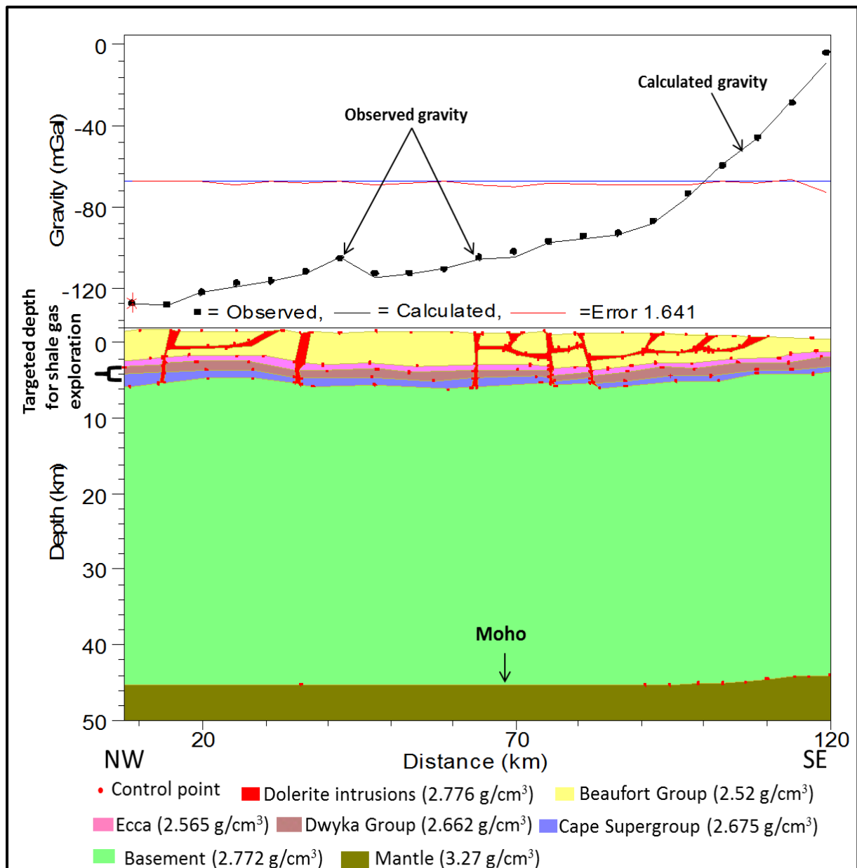
Figure 8.11 Gravity modelling of profile H - H'. VE = 2.19, Initial and final RMS errors are 61.675 and 1.641, respectively. Note: The modelled dolerite sills and dykes were originally set in horizontal and vertical positions, respectively and allowed to vary or change during the modelling process in order to have the best fit model.
