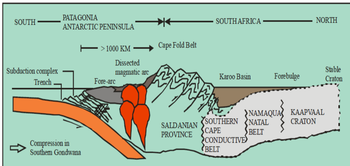
Figure 2.3 The generalized foreland basin model of the Karoo basin during the Triassic period, showing the location of the foredeep and forebulge parts of the basin in relation to the Cape Fold Belt, and the inferred position of the arc and subduction zone (Turner, 1999).
