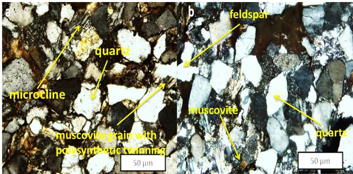
Figure 4.41 Photomicrographs of sandstones from Fort Brown Formation along Eccla Pass. (a) Sub-angular feldspar, microcline, quartz and elongated muscovite grain with polysynthetic twinning. (b) Sub-angular polycrystalline quartz grains and mostly exhibit undulatory extinction.
