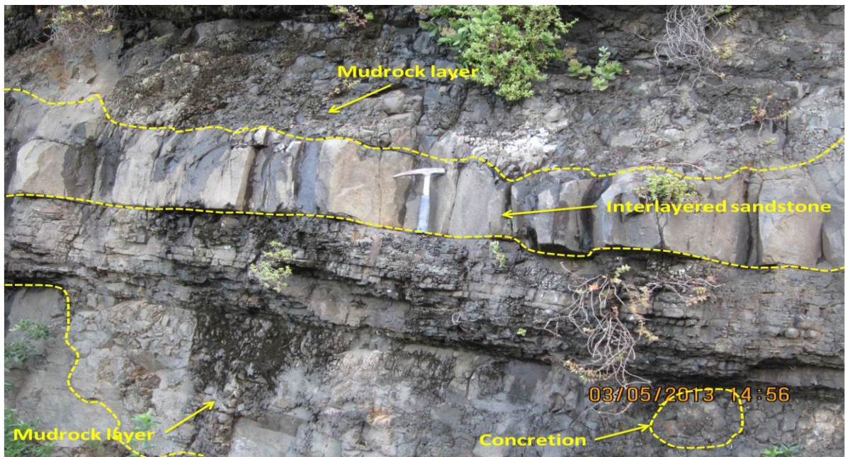
Figure 4.21 Photograph of the Koonap Formation near Fort Beaufort showing sandstone interbedded with mudrock. The sandstones show fining-upward sequence (Elevation: 241 m; Longitude E 26° 39' 04.9"; Latitude S 33° 03' 24.4").
