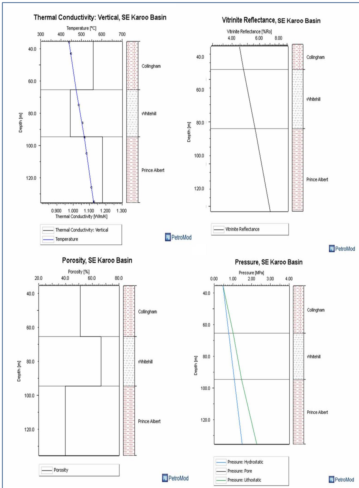
Figure 8.30 Depth plots of the southeastern Karoo Basin. Note: The hydrostatic pressure coincides with the pore pressure.
