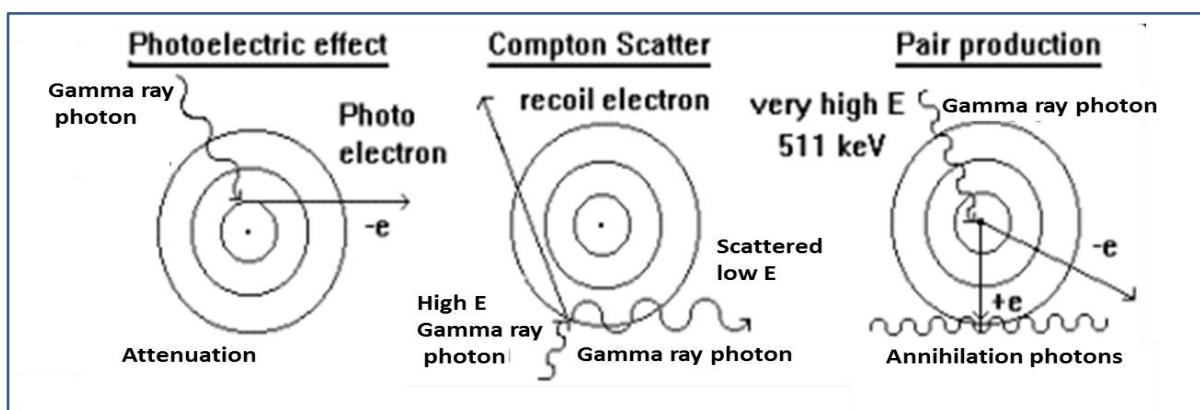
Figure 6.2 Interaction of gamma rays with matter (Killeen, 1979).
