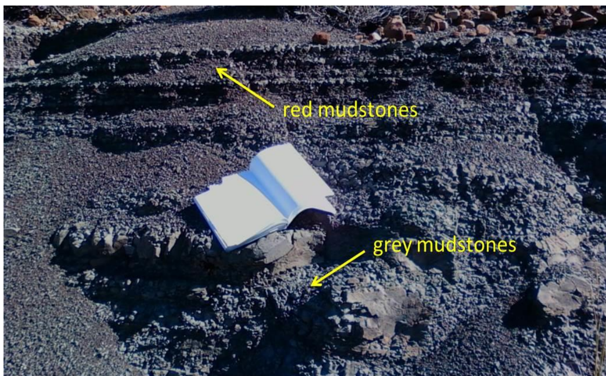
Figure 4.30 Red shales and mudstones at the base of the Palingkloof Member (where the Permo-Triassic boundary is discernable) along the R61 road between Cradock and Tarkastad towns.
