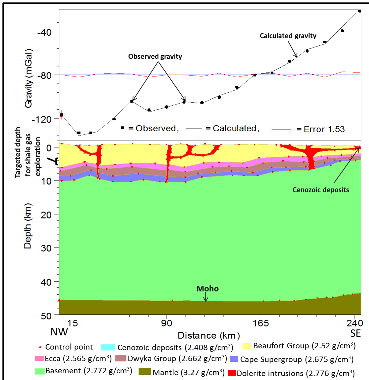
Figure 8.9 Gravity modelling of profile F - F'. VE = 1.89, Initial and final RMS errors are 48.268 and 1.53, respectively. The modelled dolerite sills and dykes were originally set in horizontal and vertical positions, respectively and allowed to vary or change during the modelling process in order to have the best fit model.
