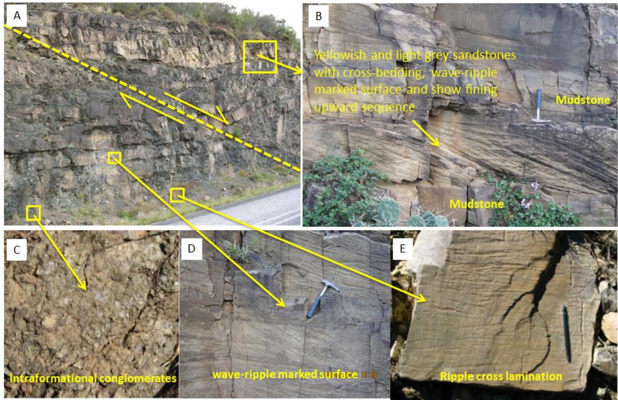
Figure 4.24 Photograph of the Oudeberg Member, north of Fort Beaufort. (A) Faulting that results in duplication of strata. (B) Fining upward sequence indicating deposition in grading upwards braided rivers. (C) intraformational conglomerates. (D) Wave-ripple marked surface. (E) Ripple cross lamination (Elevation: 833 m; Longitude E 26° 53' 34.2"; Latitude S 32° 53' 38.7").
