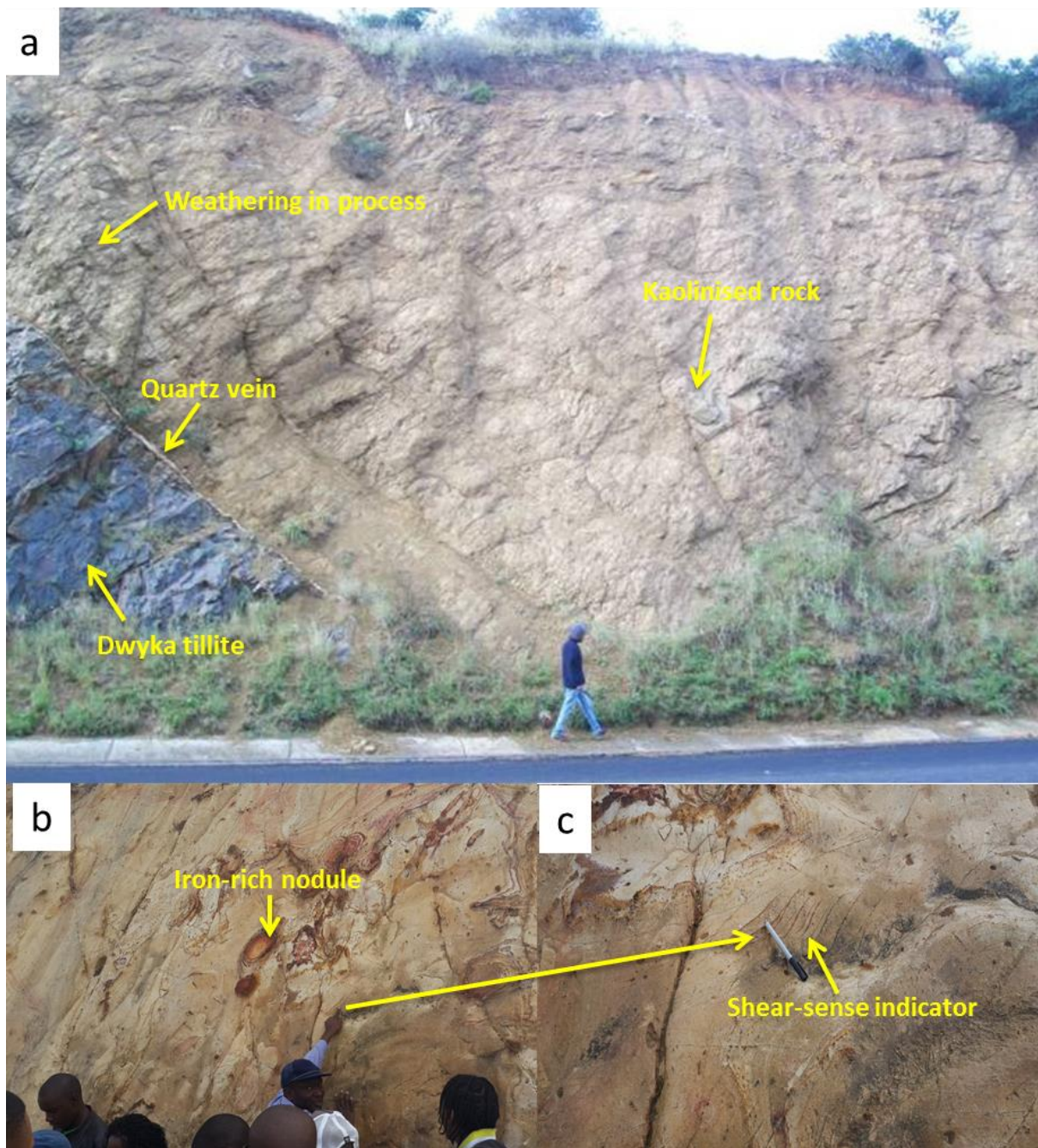
Figure 4.4 Road cut exposure of the kaolin deposit sourced from the Dwyka tillite showing iron-rich nodules, shear-sense indicators and quartz veins.
