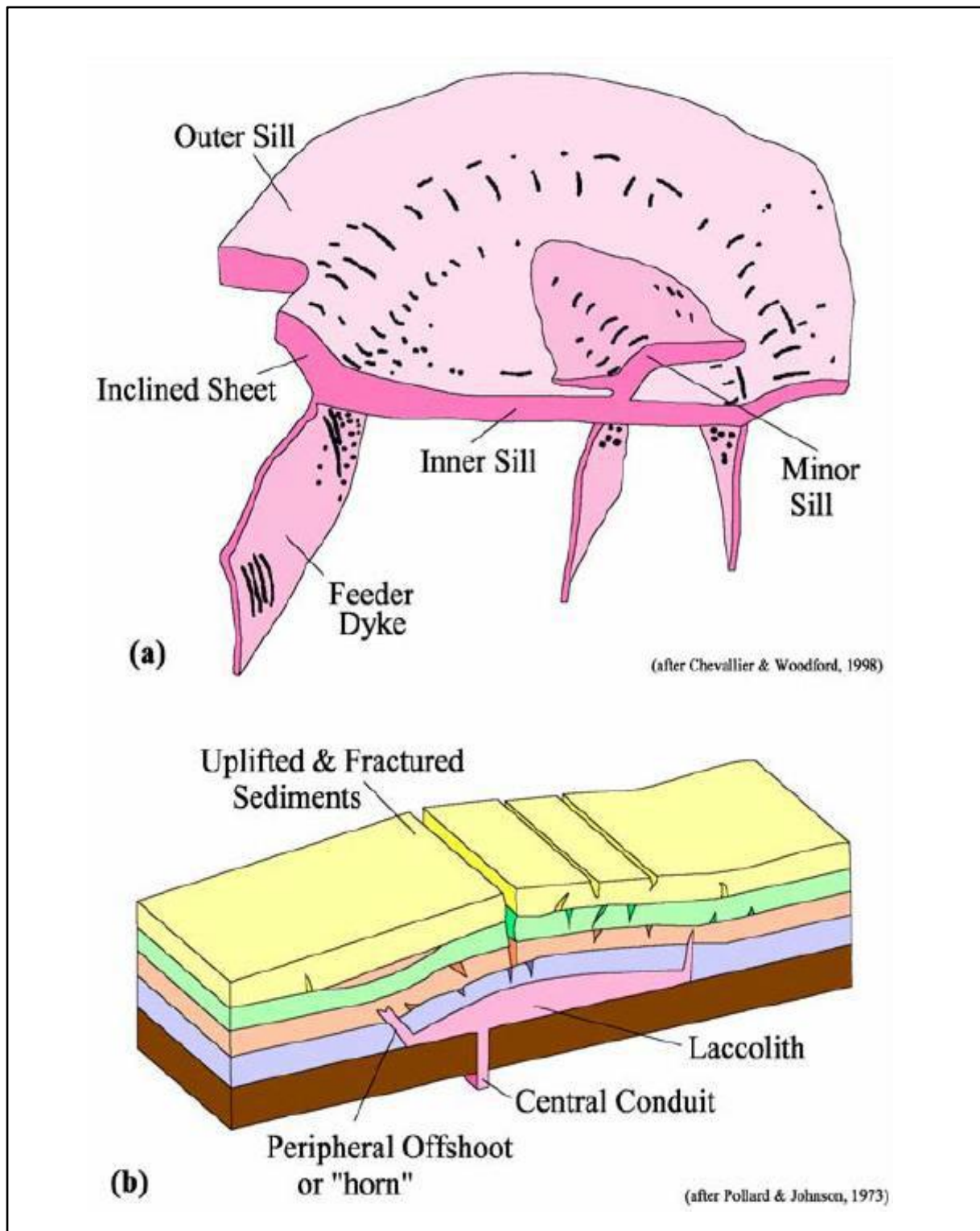
Figure 2.10 Dolerite sill/ring emplacement models; (a) Ring dyke model; (b) Laccolith model (Woodford and Chevallier, 2002).
