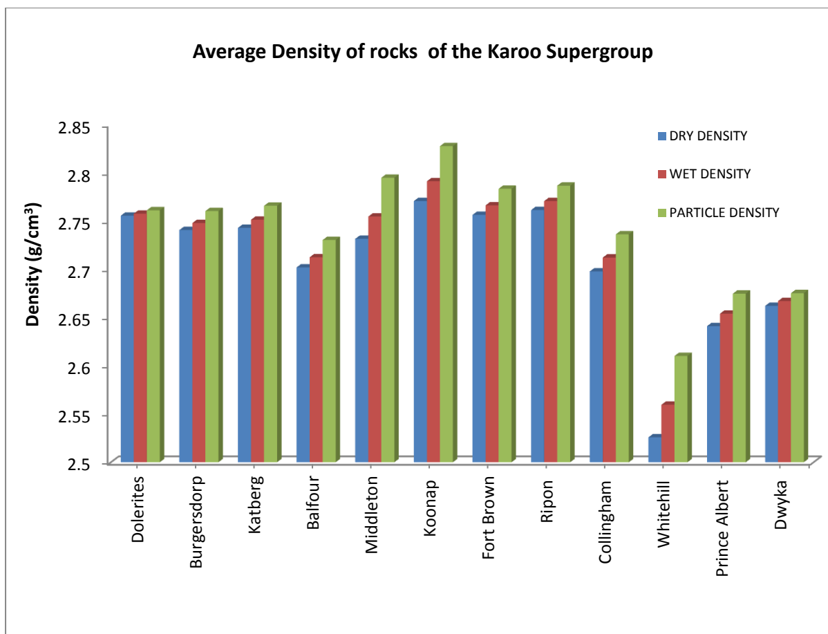
Figure 7.2 Bar chart of average densities of rock samples from the Karoo Supergroup and the dolerite intrusions.
