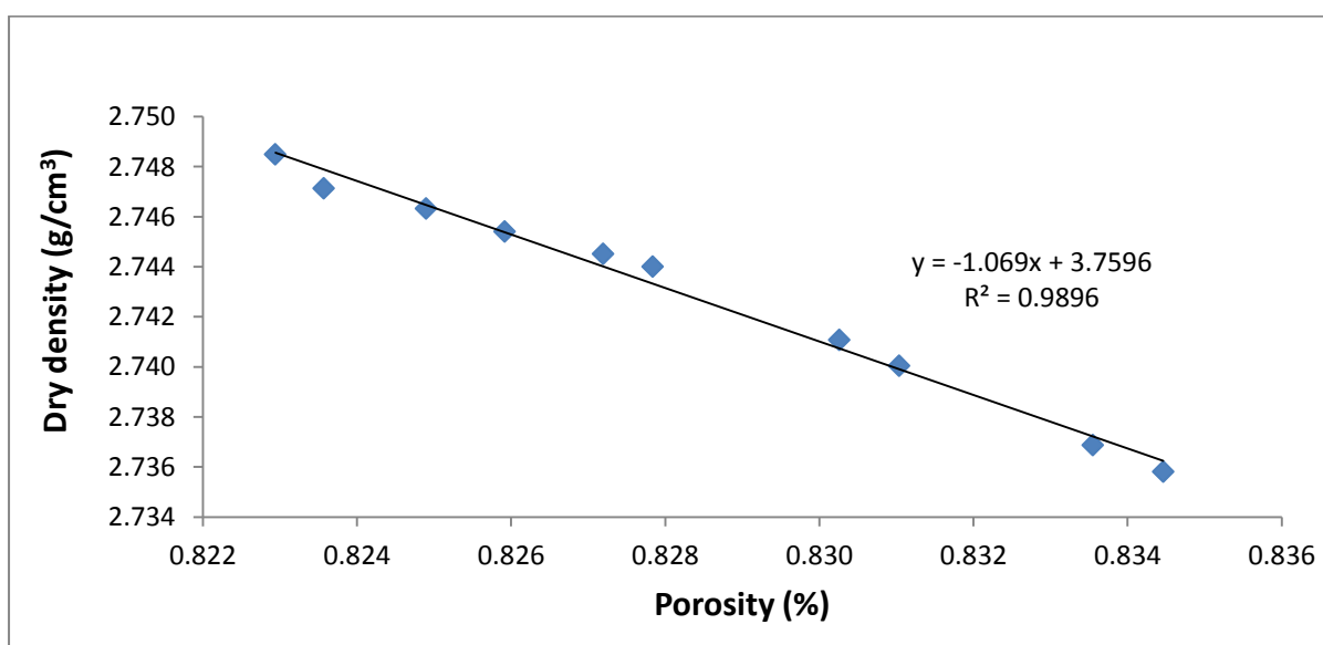
Figure C32 Plot of dry density against porosity for sandstones from the Katberg Formation.
