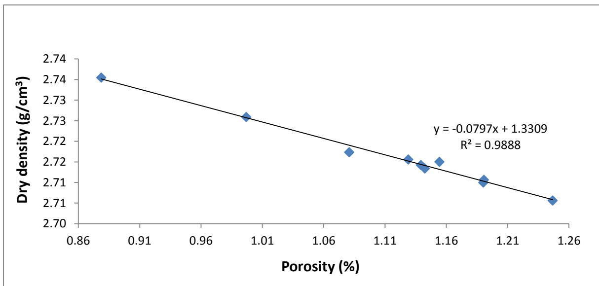
Figure C30 The plot of dry density versus porosity for sandstones from the Palingkloof Member showing linear relationship. The regression line which correlate the dry density with porosity indicate a high negative correlation with a coefficient value ( R = 0.9944 ) which is close to +1, thus implying that the variables (dry density and porosity) are closely related.
