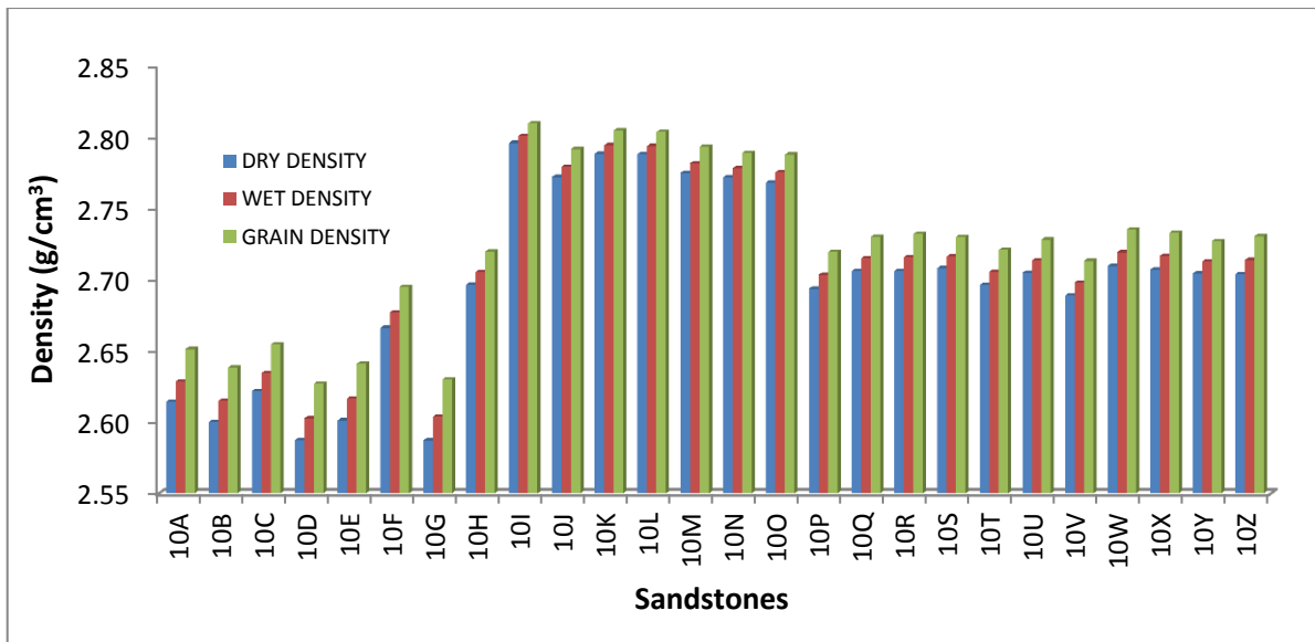
Figure C23 Bar chart of dry, wet and grain densities for the Daggaboersnek Member.
