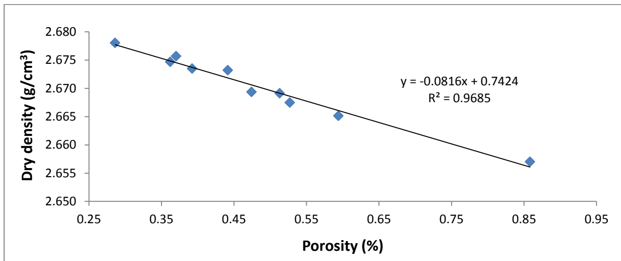
Figure C6 Dry density - porosity relationship for the Dwyka diamictite.
