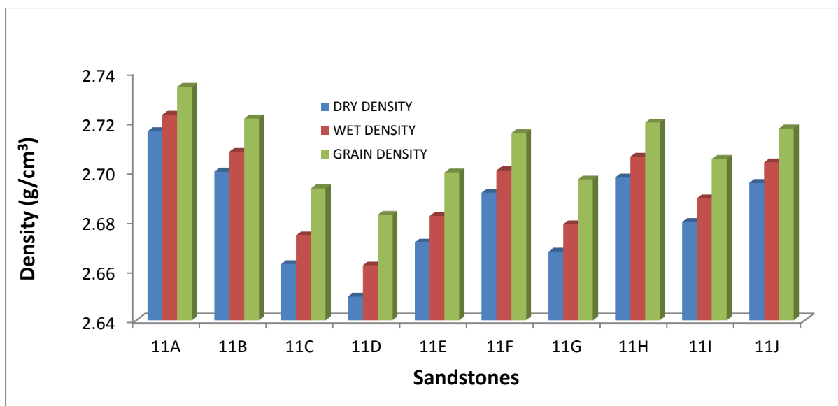
Figure C25 Bar chart of dry, wet and grain densities for the Barberskrans Member.
