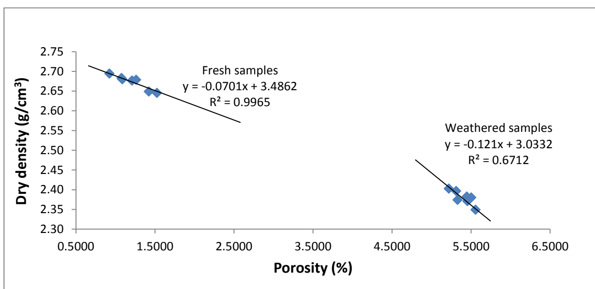
Figure C10 Dry density - porosity relationship for shale of the Whitehill Formation.
