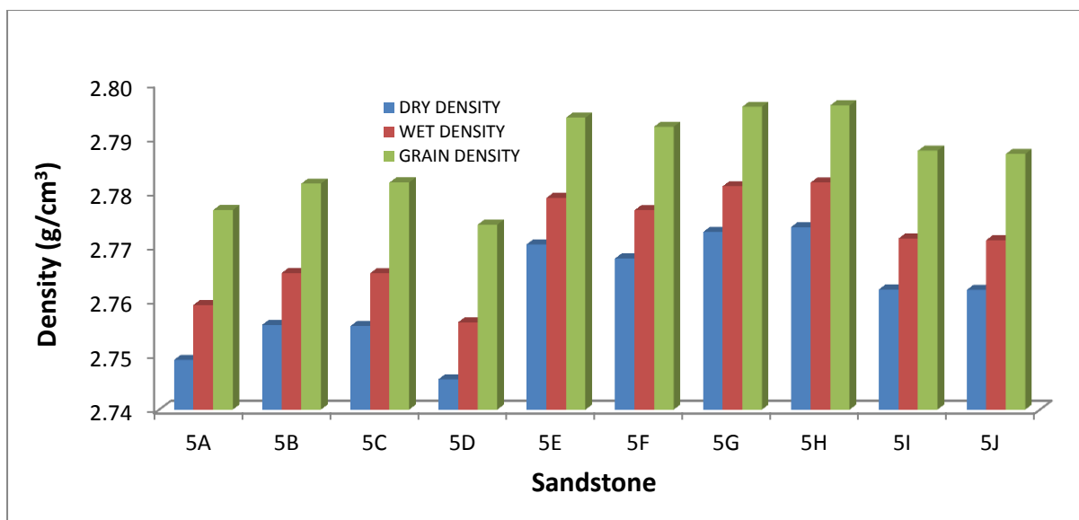
Figure C13 Bar chart of dry, wet and grain densities for sandstones from the Ripon Formation.
