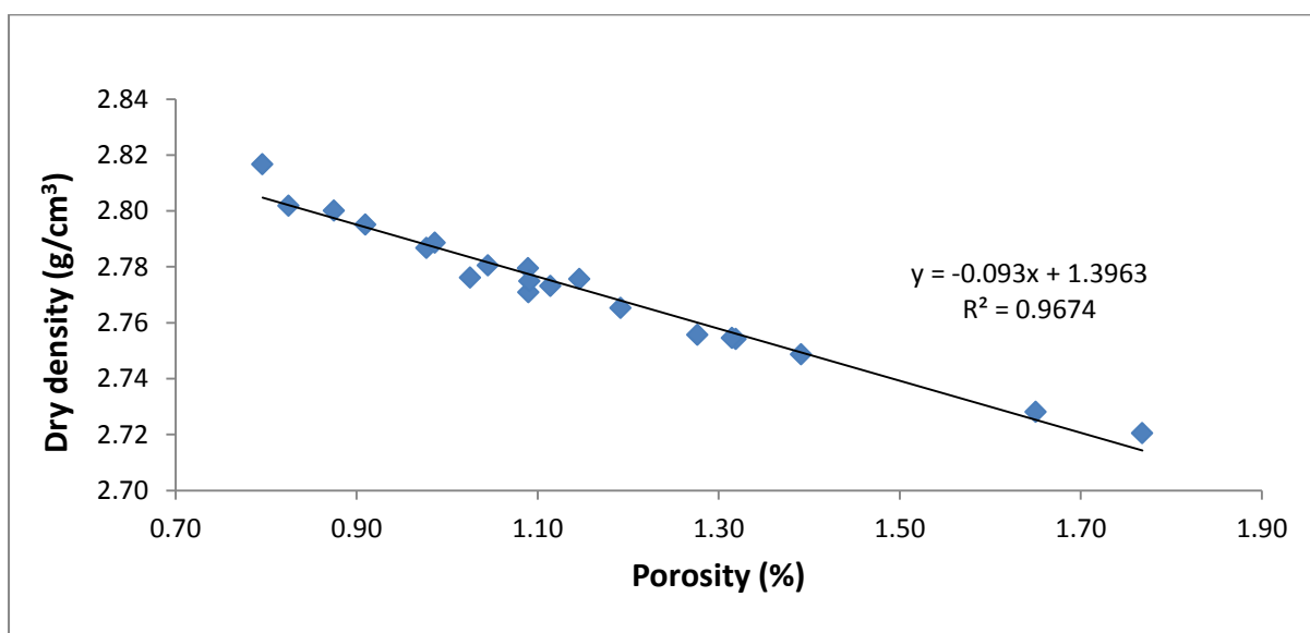
Figure C22 Dry density - porosity relationship for sandstones from the Oudeberg Member.
