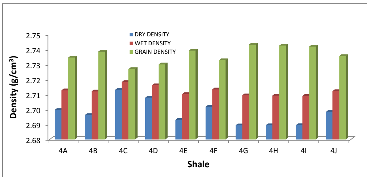
Figure C11 Bar chart of dry, wet and grain densities for shale from Collingham Formation.
