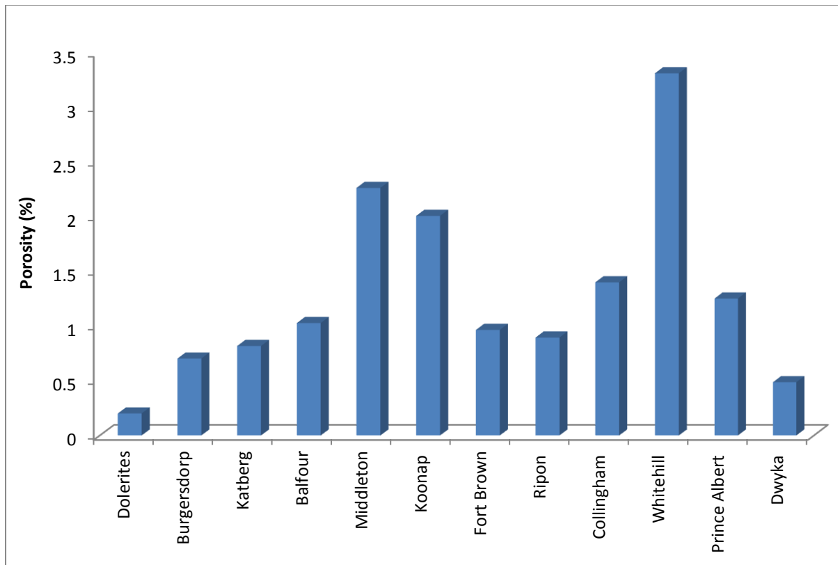
Figure 7.3 Bar chart of average porosity of rock samples from the Karoo Supergroup and the dolerite intrusions.
