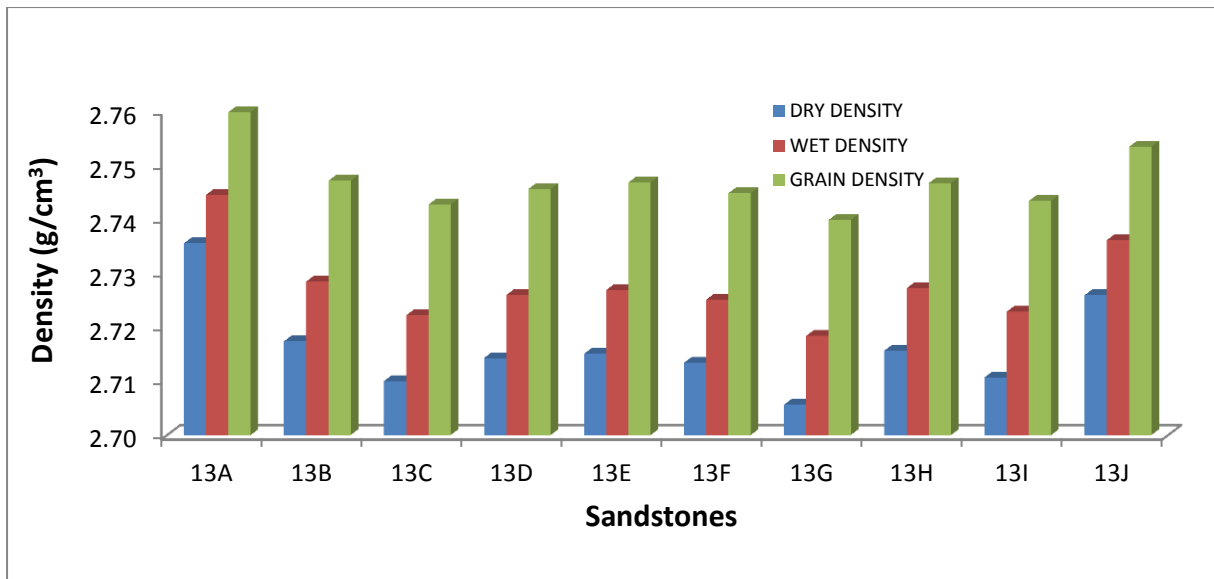
Figure C29 Bar chart of dry, wet and grain densities for the Palingkloof Member.
