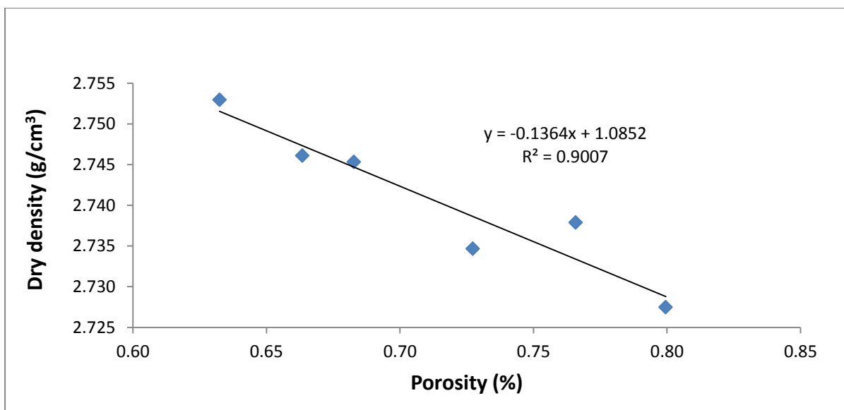
Figure C34 shows the plot of dry density versus porosity for mudstones from the Burgersdorp Formation. The coefficient of determination ( R^2 ) value is 0.9007, thus the correlation coefficient (R) is 0.9491 which is close to +1, signifying that the variables (dry density and porosity) are closely related. This negative correlation implies that the lower the density, the higher the porosity and vice versa.
