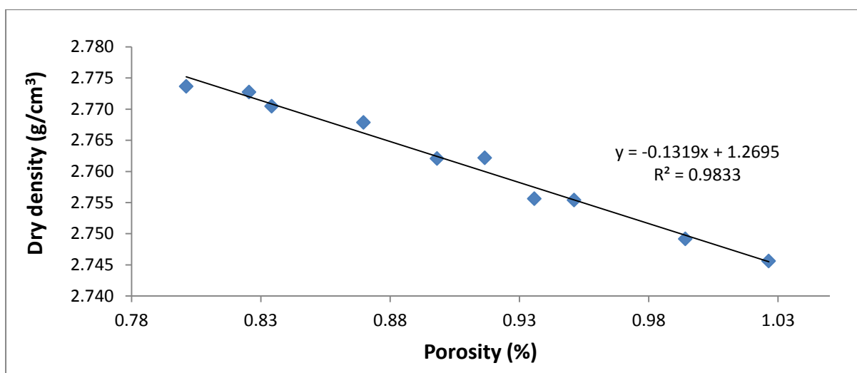
Figure C14 Dry density - porosity relationship for sandstones from the Ripon Formation.
