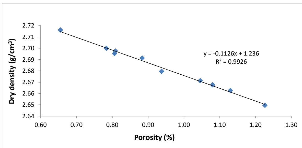
Figure C26 Dry density - porosity relationship for sandstone from the Barberskrans Member.
