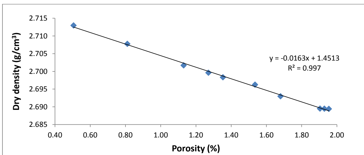
Figure C12 Dry density - porosity relationship for shale of the Collingham Formation.
