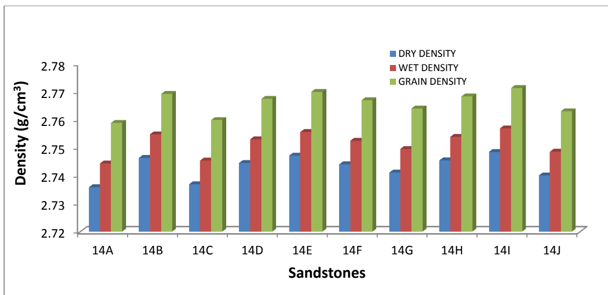
Figure C31 Bar chart of dry, wet and grain densities for the Katberg Formation.
