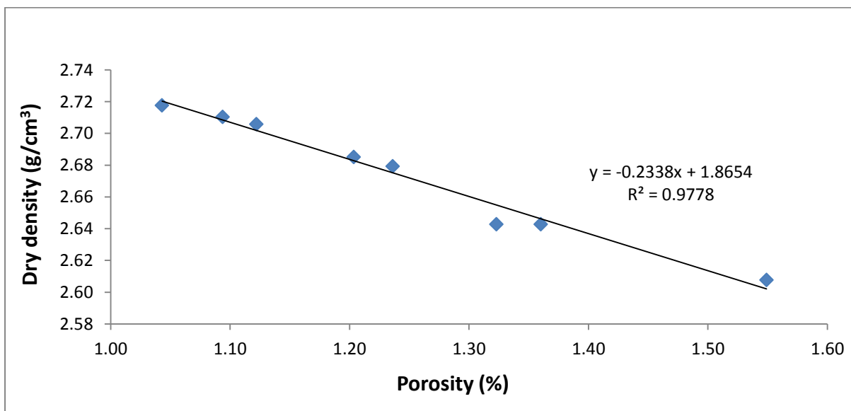
Figure C28 Plot of dry density - porosity of sandstones from the Elandsberg Member.
