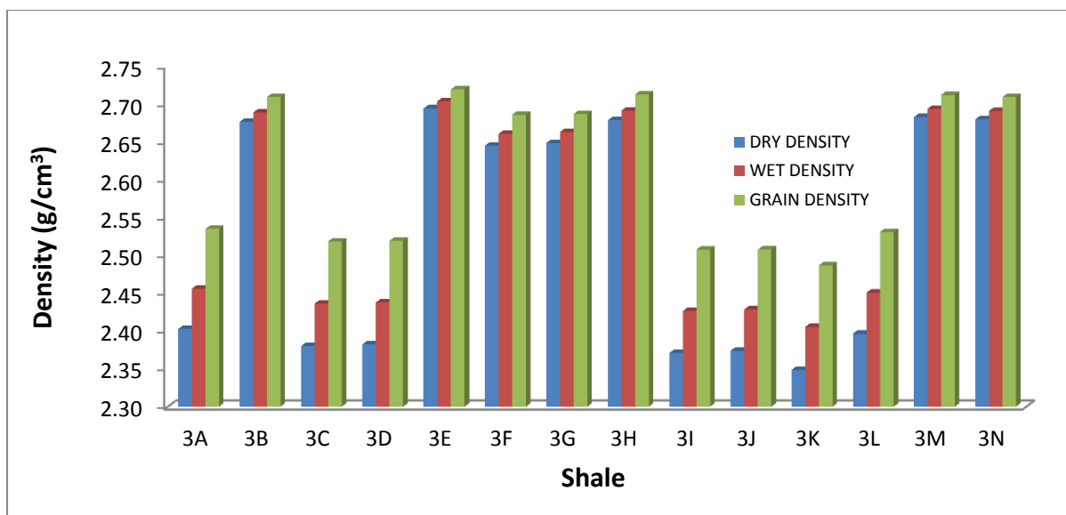
Figure C9 Bar chart of dry, wet and grain densities for shale from Whitehill Formation.
