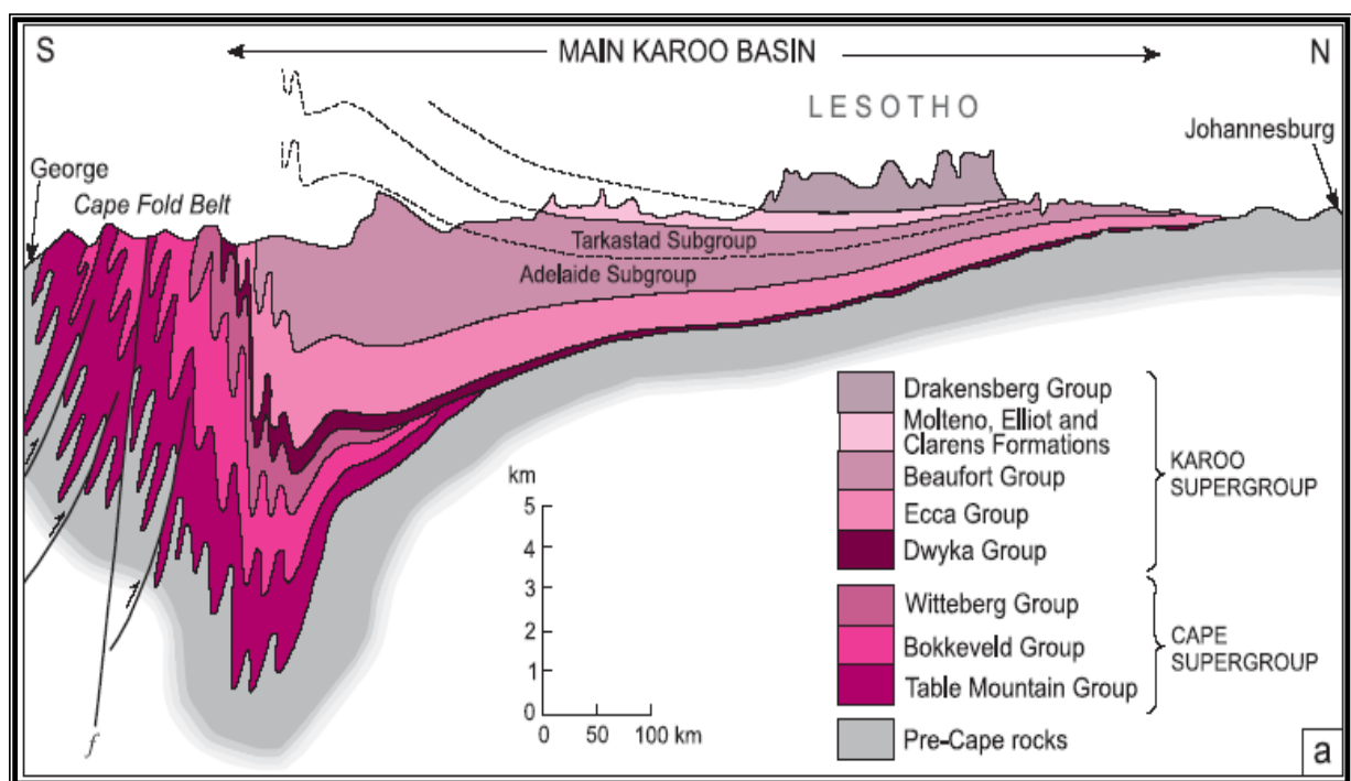
Figure 2.4 Section view of Karoo Supergroup, showing the thinning effect and also the tectonic settings (Johnson et al. , 1997).
