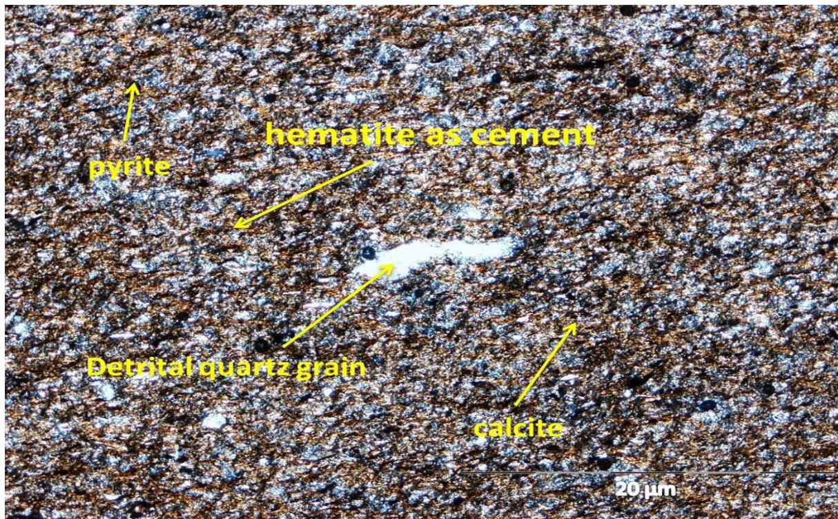
Figure 4.39 Photomicrographs of shales from Whitehill Formation along the Eccia Pass showing calcite (yellowish), pyrite (dark colours), hematite as cement and detrital quartz grain.
