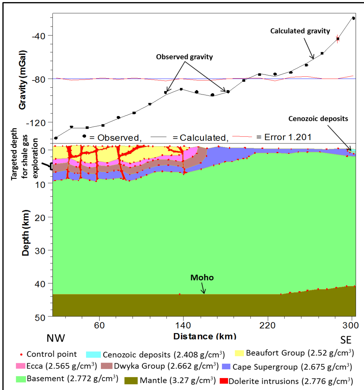
Figure 8.8 Gravity modelling of profile E - E'. VE = 1.53, Initial and final RMS errors are 65.381 and 1.201 respectively.
