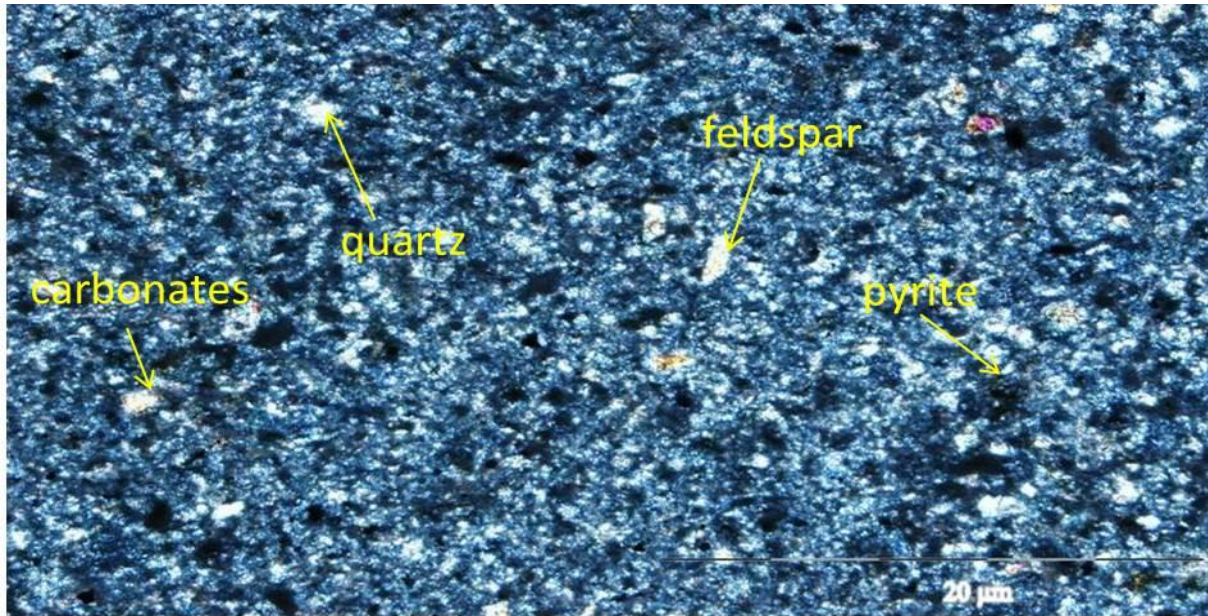
Figure 4.47 Photomicrographs of sandstones from Burgersdorp Formation showing quartz, feldspar, pyrite and carbonates.
