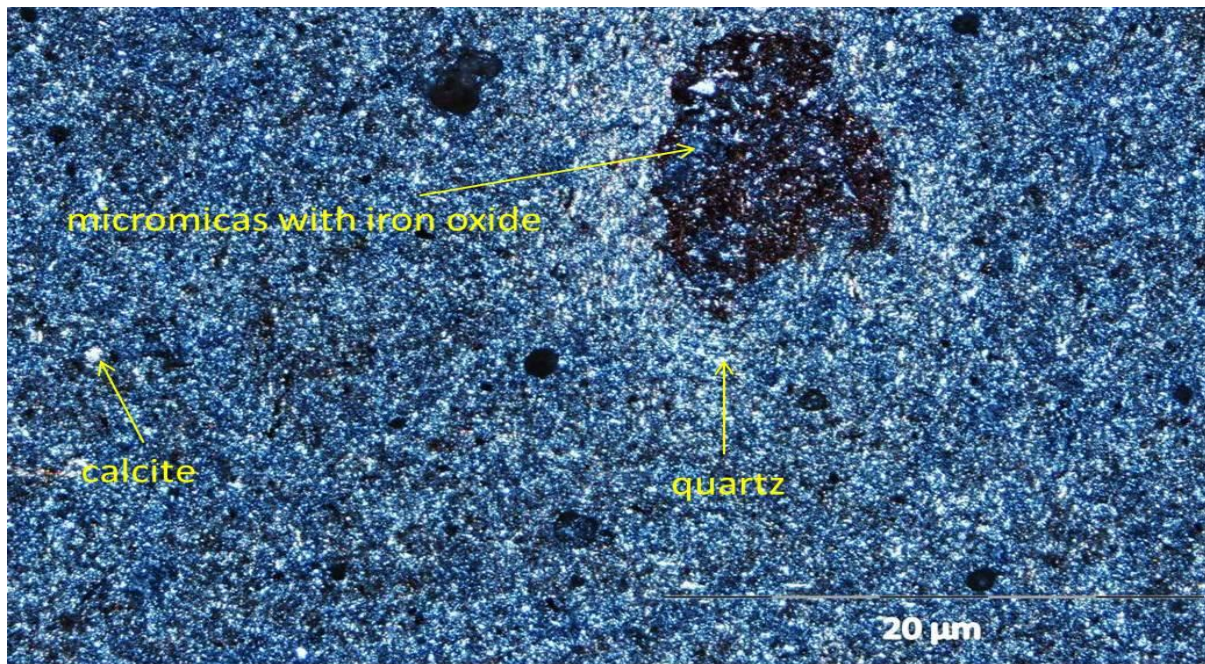
Figure 4.44 Photomicrographs of mudstones from Middleton Formation around Fort Beaufort showing quartz, calcite and micromicas with iron oxide.
