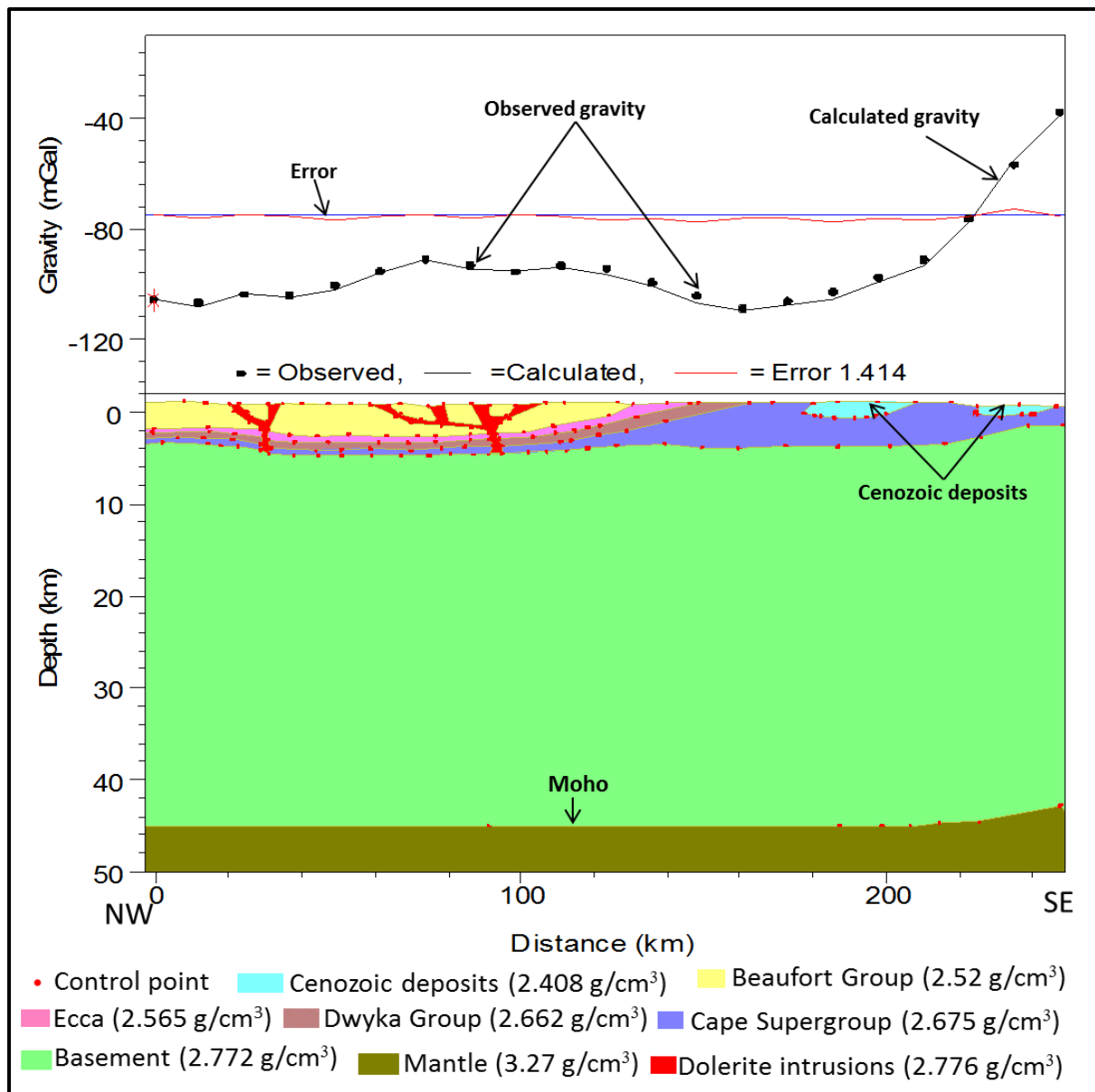
Figure 8.13 Gravity modelling of profile J - J'. VE = 0.93, Initial and final RMS errors are 48.483 and 1.414, respectively. Note: When the black curve (calculated gravity) matches with the black dots (observed gravity), it indicates a perfect fit with minimum error.
