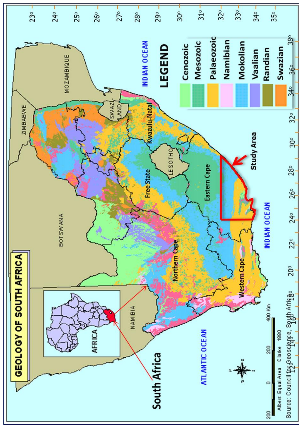
Figure 1.1 Geological map showing location of the study area (Modified after Council for Geoscience, 1995).
