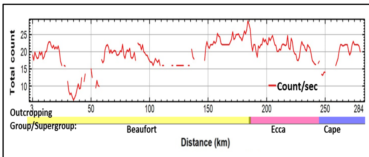
Figure 6.8 Profile for total gamma radiation count rate along Line K - K'.
