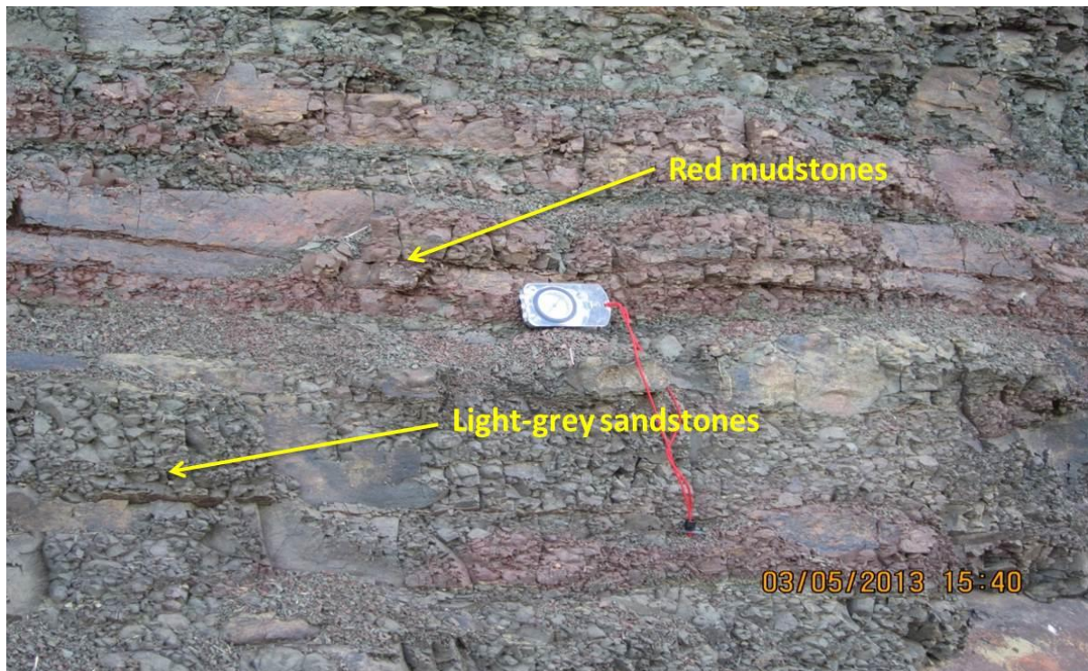
Figure 4.22 Photograph the Middleton Formation around Fort Beaufort showing red mudstones interbedded with light-grey sandstones that show fining-upward sequence believed to be deposited in low-energy systems (Elevation: 463 m; Longitude E 26° 37' 58.7"; Latitude S 33° 51' 26").
