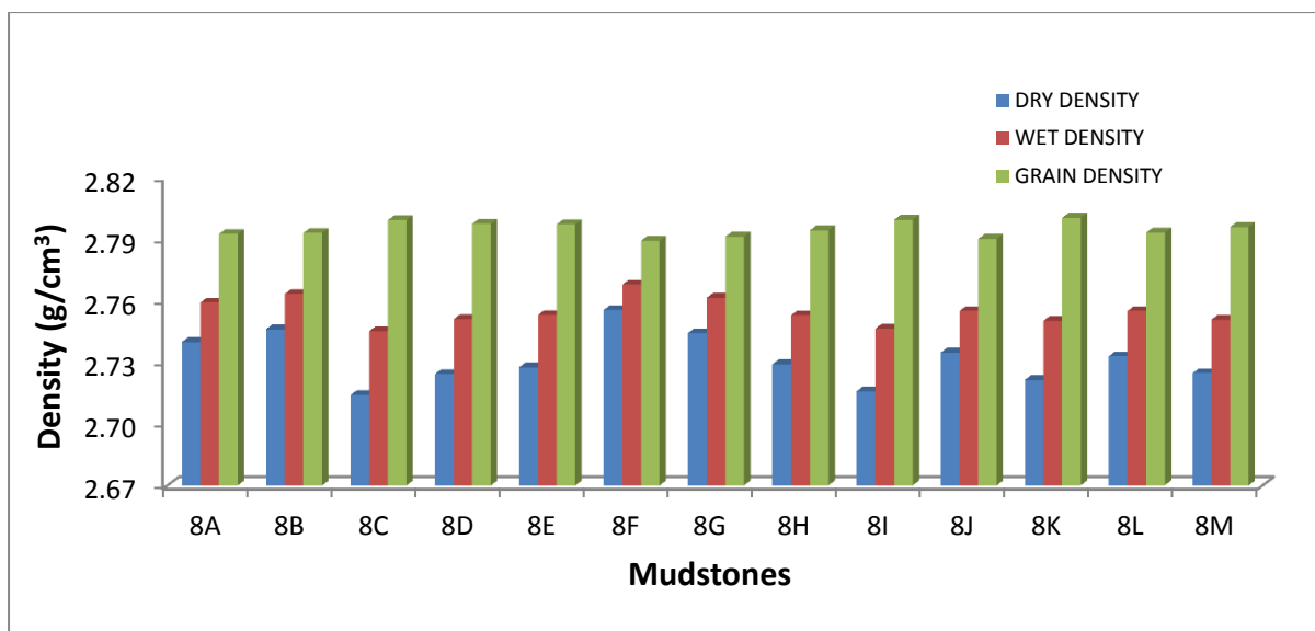
Figure C19 Bar chart of dry, wet and grain densities for the Middleton Formation.
