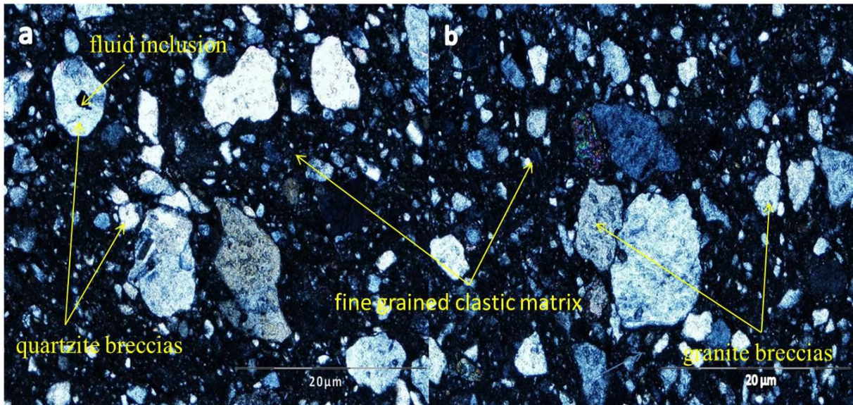
Figure 4.37 Photomicrographs of Dwyka diamictites along the Eccia Pass. (a) Irregular fluid inclusion around sub-angular quartz grains in quartzite clast. (b) Sub-round-angular granite and minor quartzite components in the breccias (fine grained clastic matrix which are rich in clay minerals).
