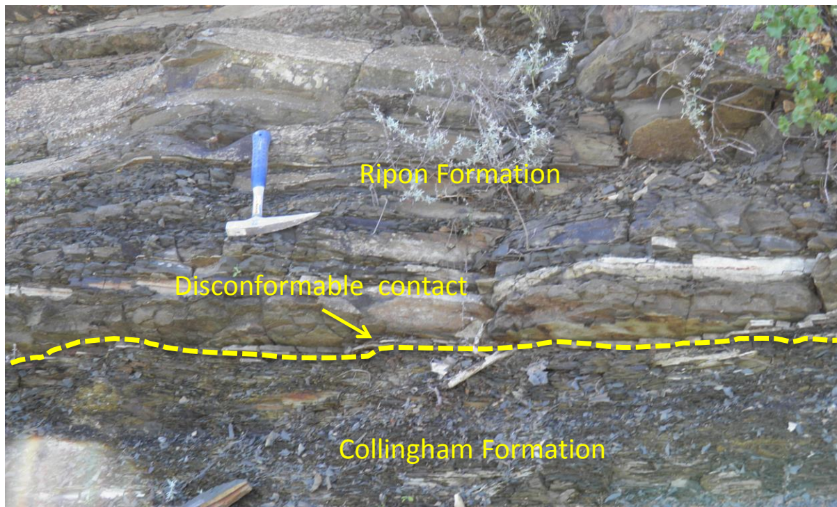
Figure 4.15 Disconformable contact between the Collingham Formation at the bottom and the Ripon Formation at the top. The top beds are slightly inclined compared to the bottom beds, indicating a disconformity or lower angle of unconformity.
