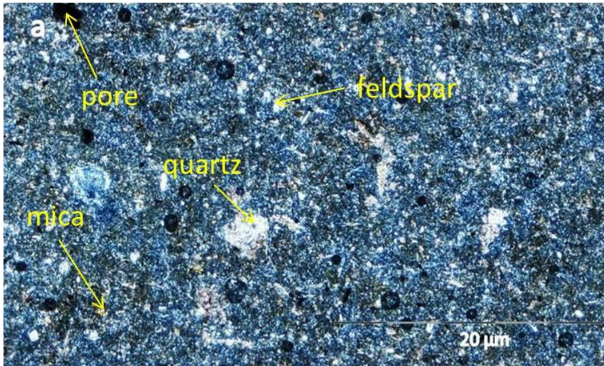
Figure 4.43 Photomicrographs of sandstones from Koonap Formation near Fort Beaufort showing feldspar, quartz, mica and pores.
