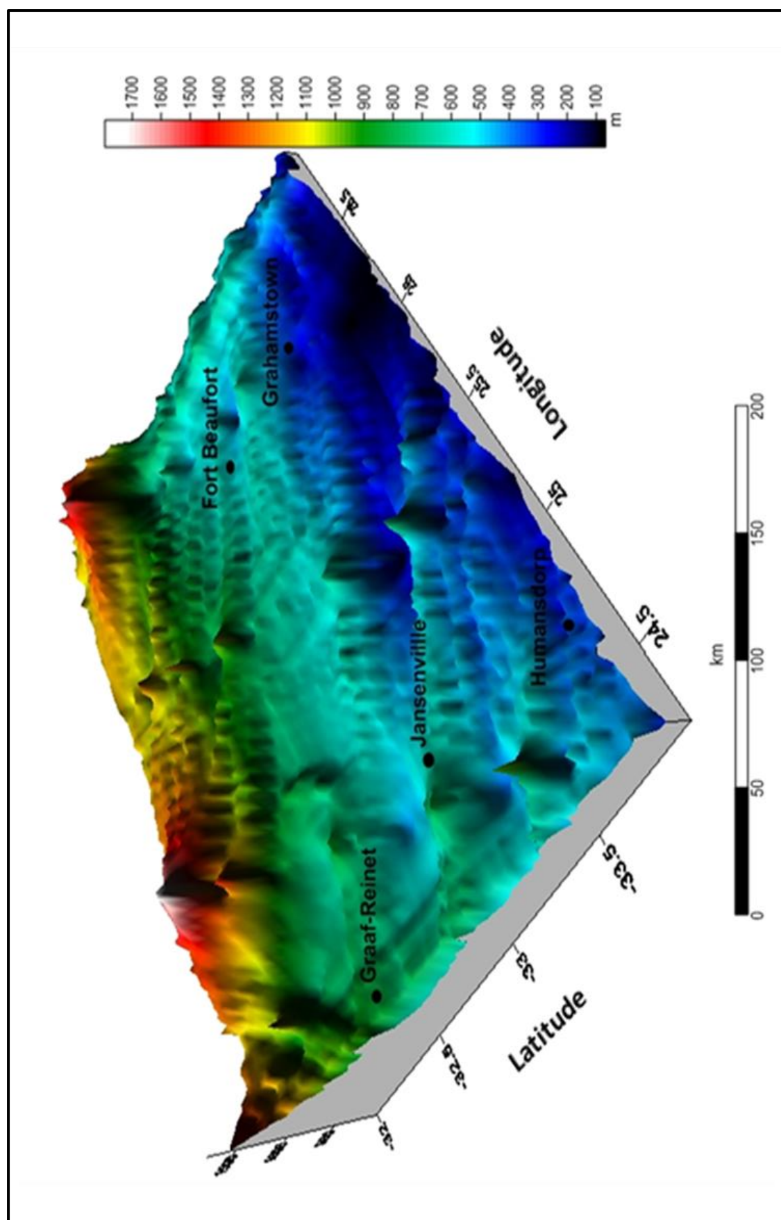
Figure 8.2 3D view of the current elevation map (Data extracted from Google Earth and displayed using Surfer-10)
