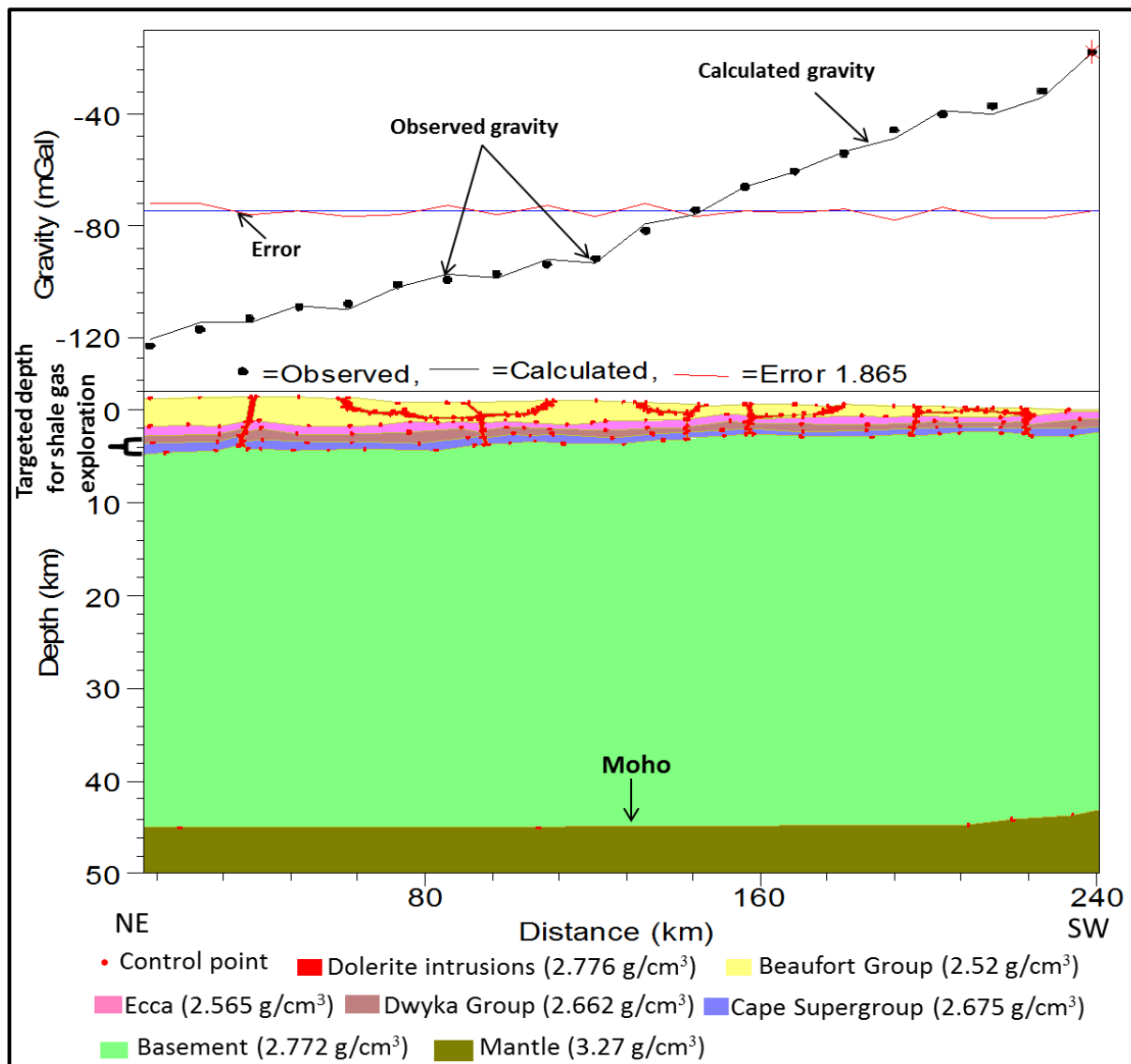
Figure 8.17 Gravity modelling of profile N – N'. Vertical exaggeration = 3.11, Initial and final RMS errors are 84.381 and 1.865, respectively. Note: The modelled dolerite sills and dykes were originally set in horizontal and vertical positions, respectively and allowed to vary or change during the modelling process in order to have the best fit model. When the black curve (calculated gravity) joins/matches with the black dots (observed gravity), it indicates a perfect fit with minimum error.
