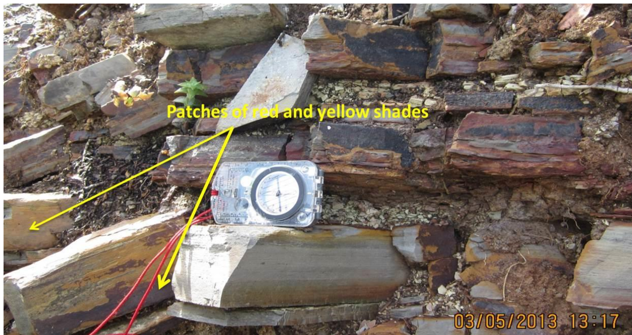
Figure 4.10 Weathered thinly laminated shale of the Whitehill Formation with patches of red and yellow shades and generally rich in iron sulphides (pyrite). (Elevation: 499 m; Longitude E 26° 37' 38.3"; Latitude S 33° 12' 58.4").
