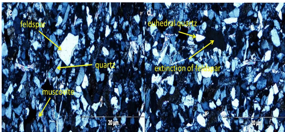
Figure 4.42 (c) Feldspar, quartz and mica as framework grains. (d) Extinction of feldspar (black) with euhedral quartz, poorly sorted with angular to sub-round grains.
