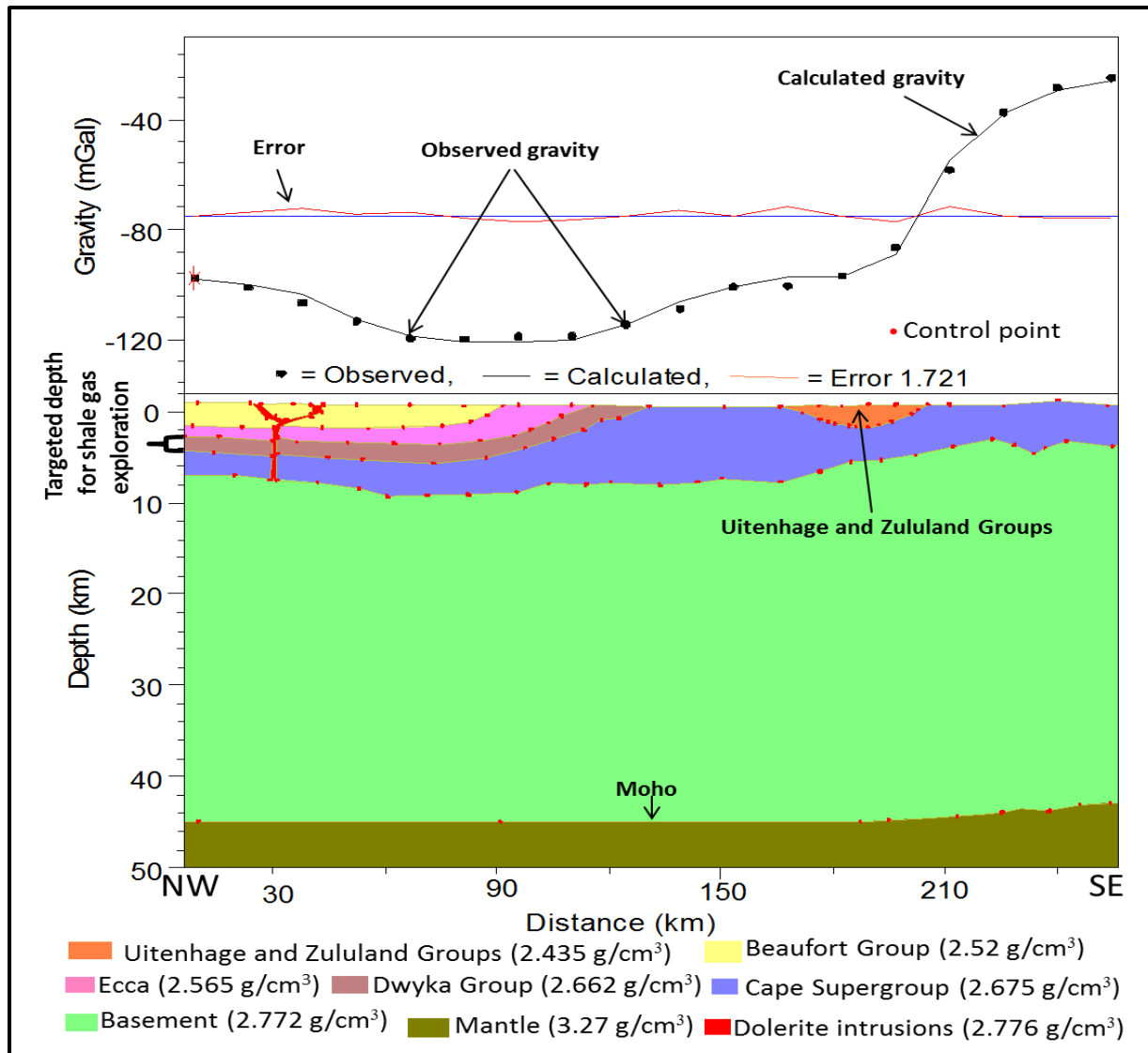
Figure 8.12 Gravity modelling of profile I – I'. VE = 0.80, Initial and final RMS errors are 64.389 and 1.721, respectively.
