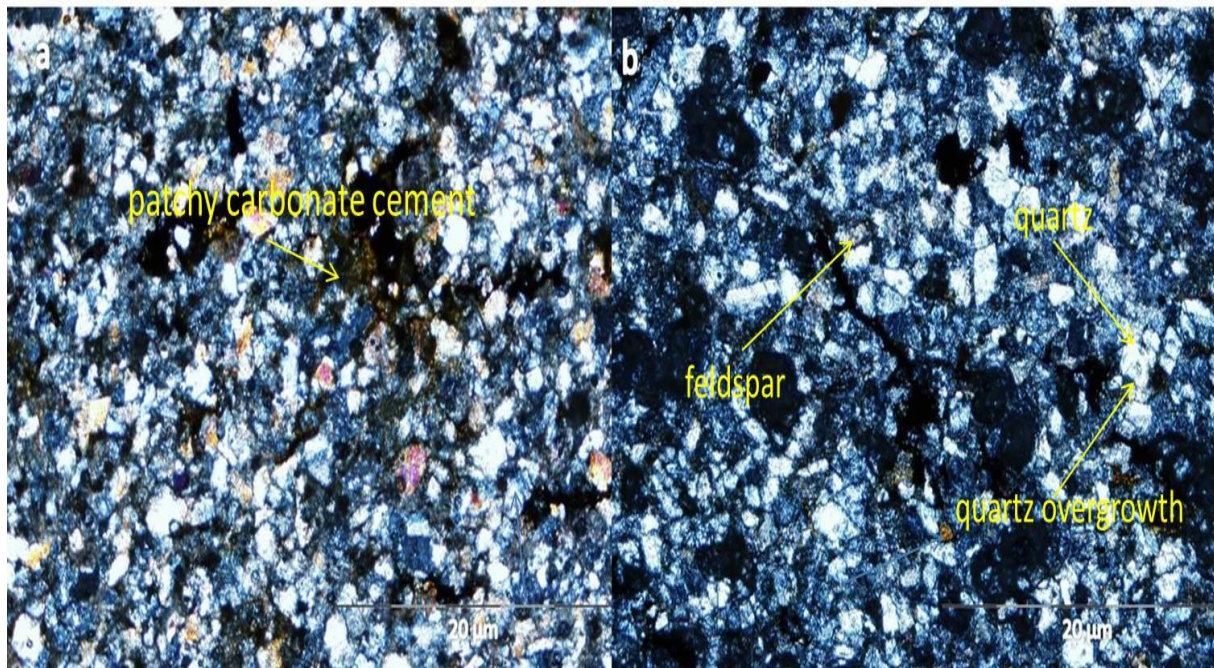
Figure 4.45 Photomicrographs of sandstones from Balfour Formation. (a) fine matrix, poorly sorted and sub-round grains with patchy carbonate cement occurring in the interstitial spaces. (b) Monocrystalline quartz, feldspars and other rock fragments with quartz overgrowths. Note: No significant difference is seen in the sandstones of all the members that make up the Balfour Formation, thus only one section is presented here.
