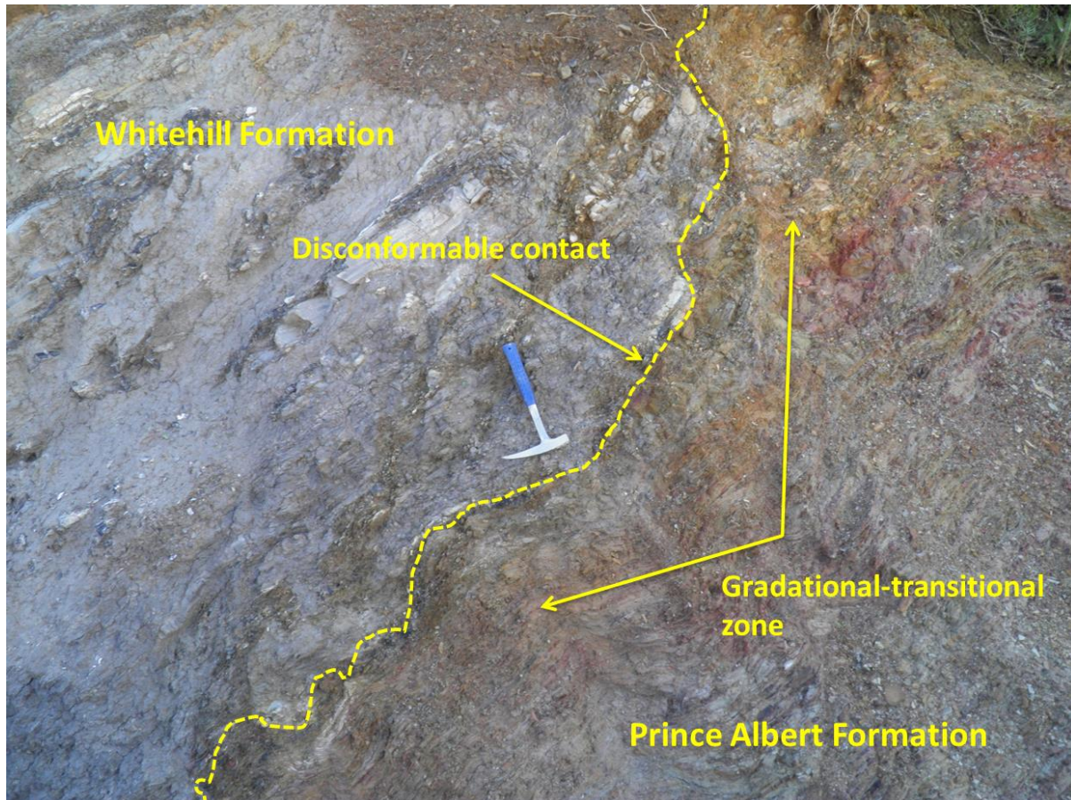
Figure 4.8 Photograph showing gradational-transitional zone and disconformable contact between the Prince Albert Formation and the Whitehill Formation along the Eccca Pass.
