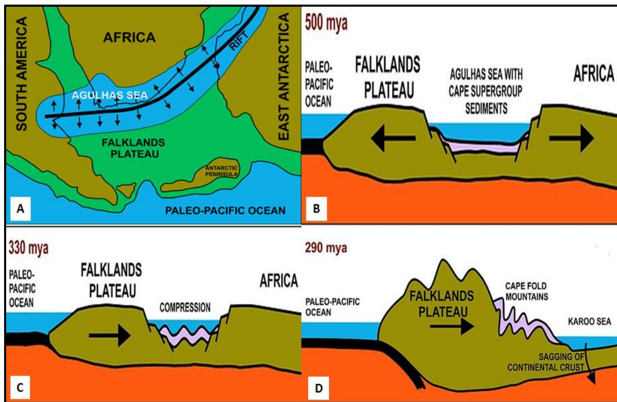
Figure 8.26 Events that led to the development of the Karoo basin (Karoo Period of sediment deposition) in Southern Africa. (A) Southern Gondwana during the Cambrian-Ordovician Periods. The olive-green colour depicts today's continents into which the supercontinent finally broke up. (B) The geology about 500 Ma, with the sediments that would later form the Cape Supergroup settling in the Agulhas Sea. (C) The drifting of the Falkland Plateau northwards once again to close the Agulhas Sea. This drifting caused the Cape Supergroup to be deformed and resulted in a series of folds. (D) The subduction of the paleo-Pacific Oceanic plate beneath the Falkland Plateau, during the Early Permian period, resulted in a massive range of mountains. These mountains were later eroded into the Karoo Sea, forming, especially, the Beaufort Group of the Karoo Supergroup ( http://en.wikipedia.org/wiki/Karoo_Supergroup ). Note: In Figure 8.26 (B - D), the continental plates are represented by the olive-green structures, the paleo-Pacific - Oceanic plate is shown with the thick black layer on the left, while the orange and blue colour shows the upper mantle and the flooded areas or ocean, respectively.
