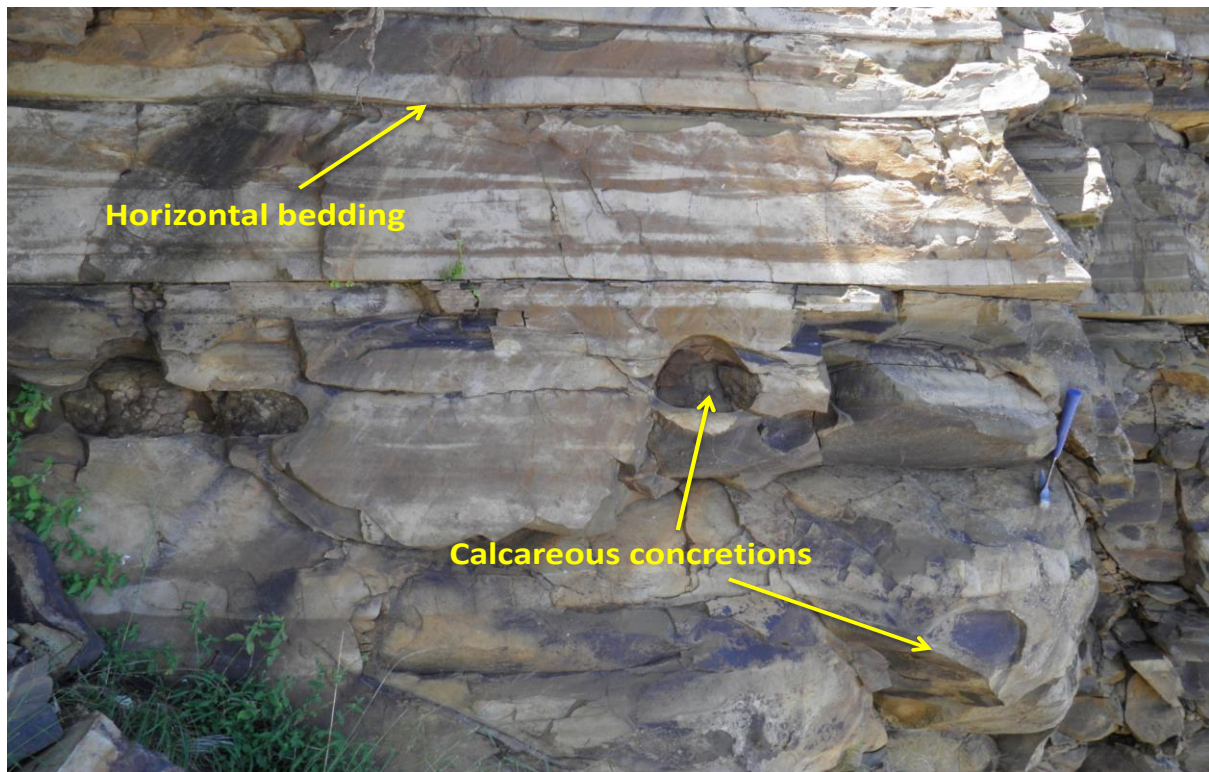
Figure 4.18 Well-developed horizontal bedding, lenticular bedding (upper middle), calcareous concretions, and joints on the greywacke in the basal unit of the Ripon Formation.
