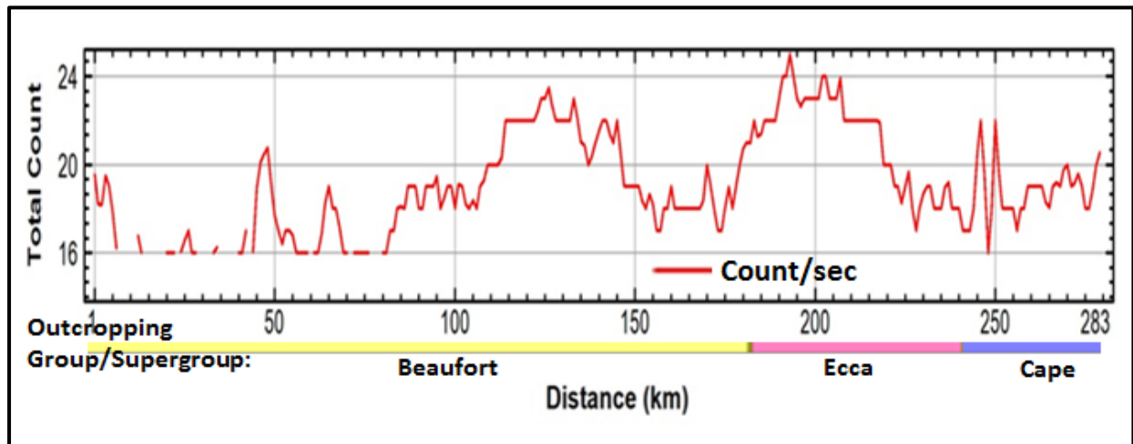
Figure 6.5 Profile for total gamma radiation count rate along Line A - A'.
