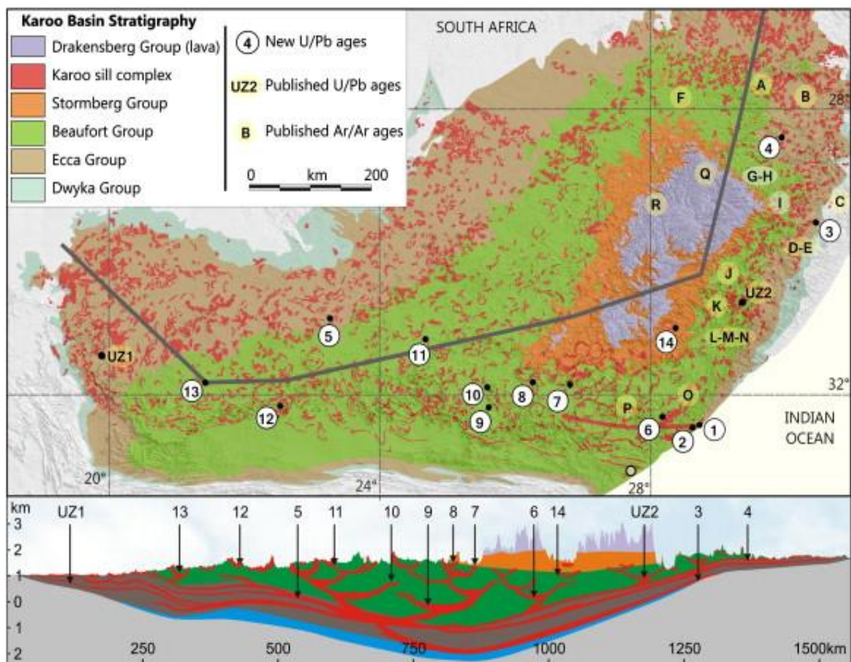
Figure 2.7 The geographical distribution/widespread of the dolerite intrusions throughout the Karoo Basin of South Africa ( http://karoospace.co.za/dolerite-karoos-fracking-game-changer ).
