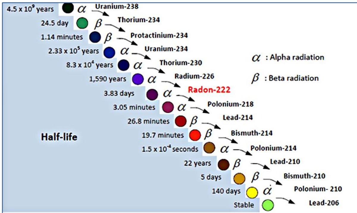
Figure 6.1 Half-life for the decay of uranium-238 to stable lead-206 (Stevenson et al., 2004).
