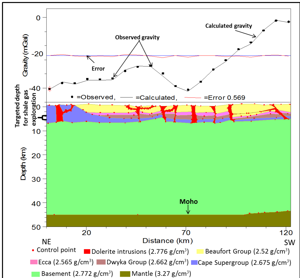
Figure 8.16 Gravity modelling of profile M – M'. Vertical exaggeration = 0.9, Initial and final RMS errors are 74.381 and 0.569, respectively. Note: When the black curve (calculated gravity) joins/matches with the black dots (observed gravity), it indicates a perfect fit with minimum error.
