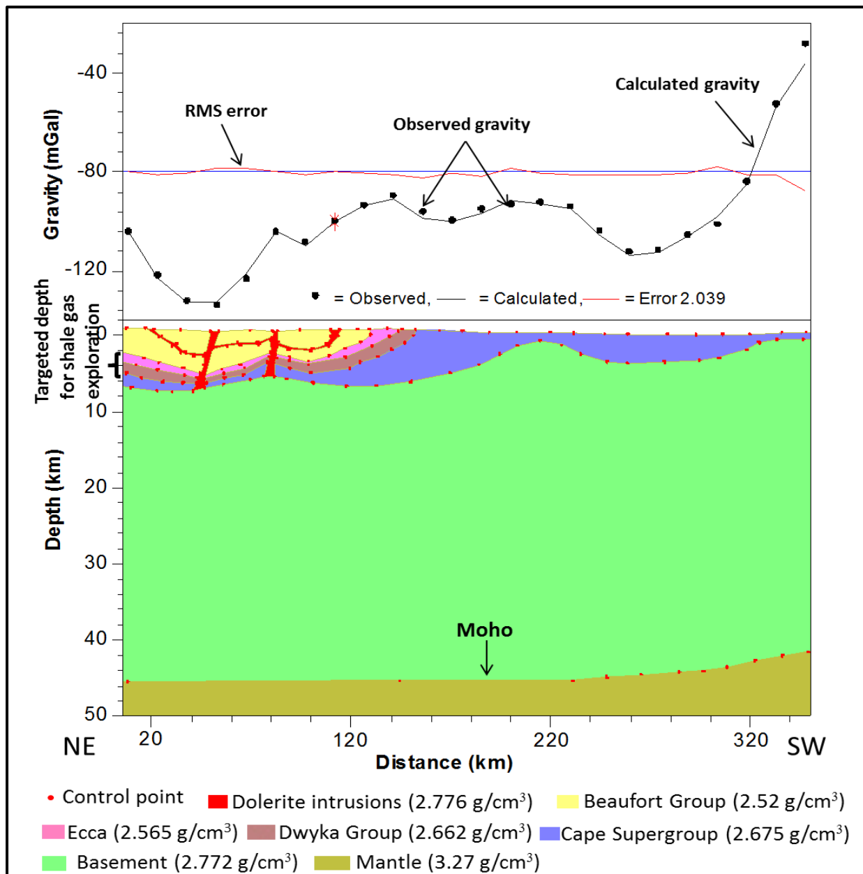
Figure 8.4 Gravity modelling of profile A - A'. Vertical exaggeration (VE) = 2.12, Initial and final RMS errors are 95.481 and 2.039, respectively.
