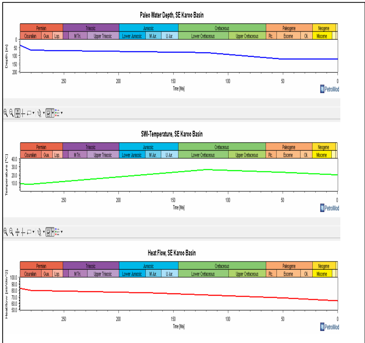
Figure 8.29 Boundary conditions plot of the southeastern Karoo Basin.
