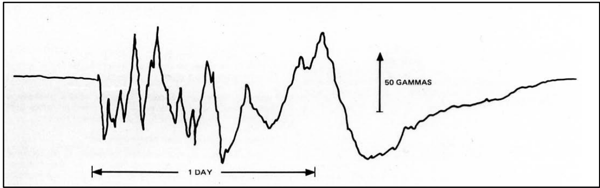
Figure B4 Magnetic storm associated with high solar activity (Reeves, 2005).
