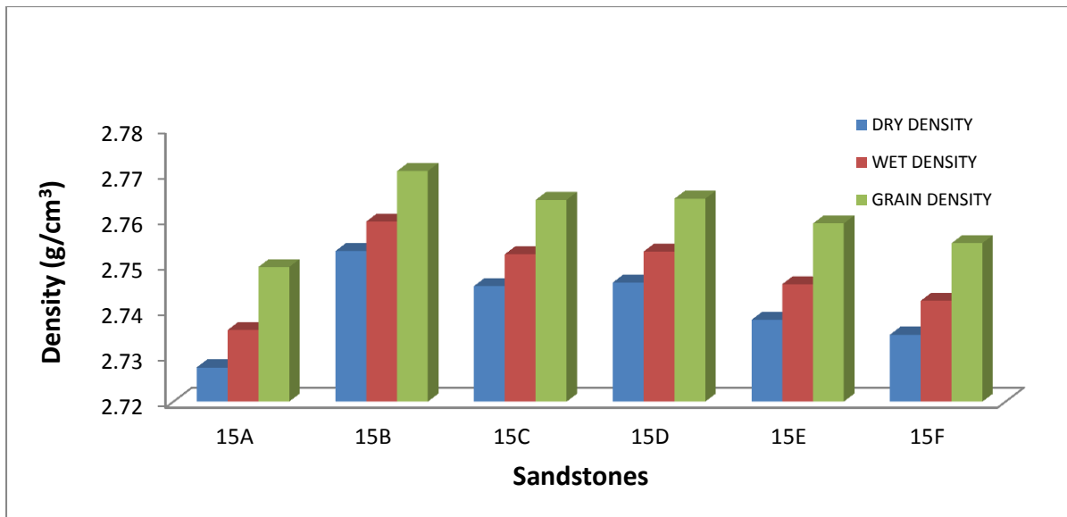
Figure C33 Bar chart of dry, wet and grain densities for the Burgersdorp Formation.
