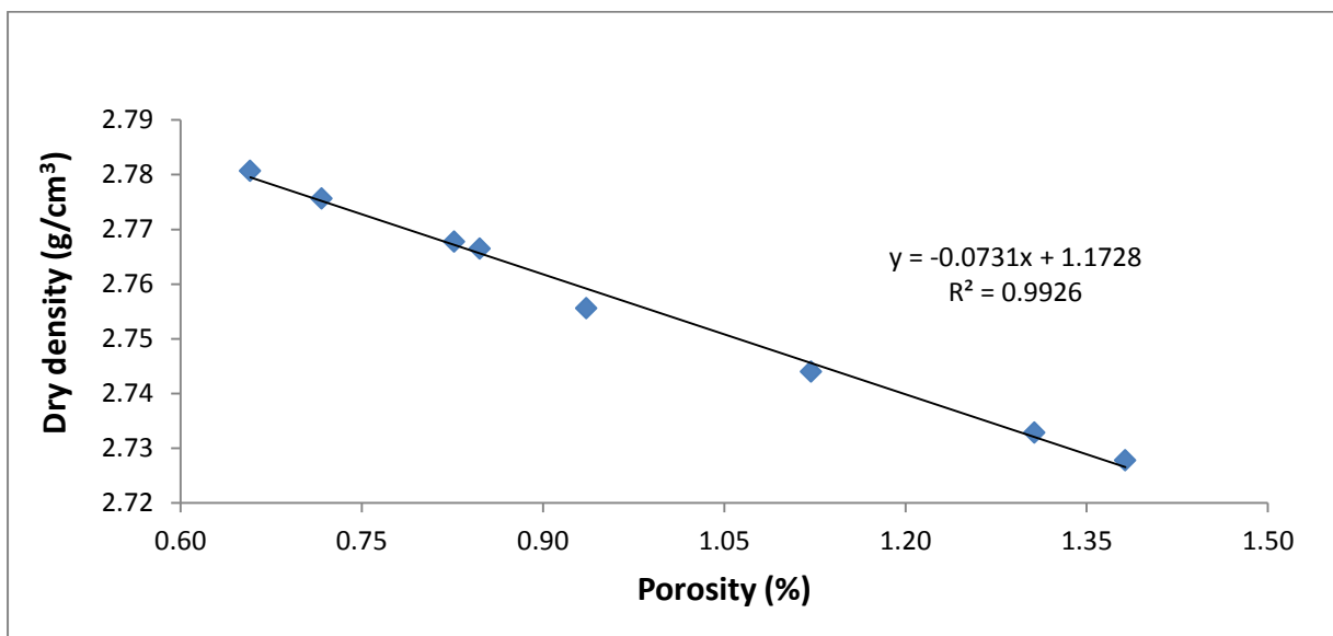
Figure C16 Dry density - porosity relationship for the Fort Brown Formation.
