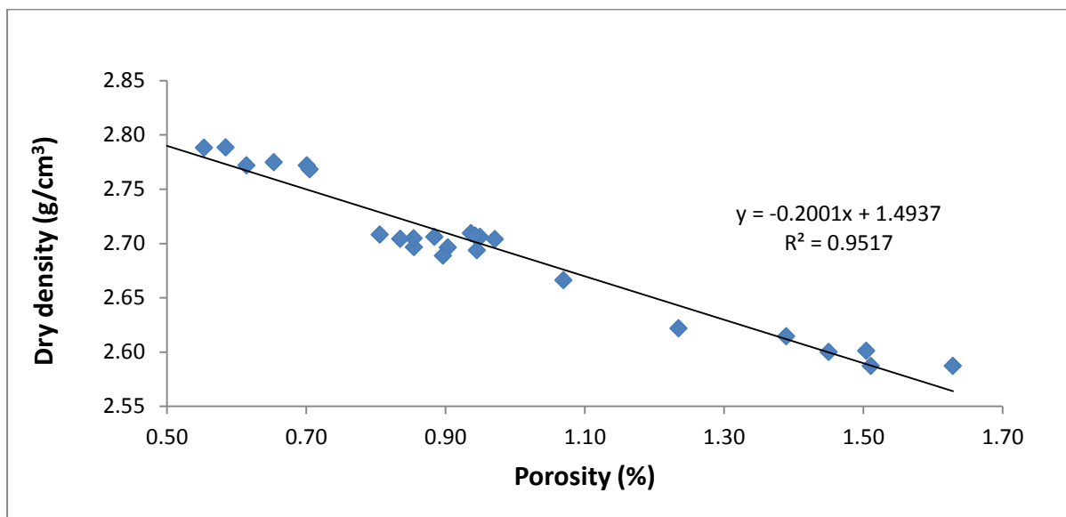
Figure C24 Dry density - porosity relationship for the Daggaboersnek Member.
