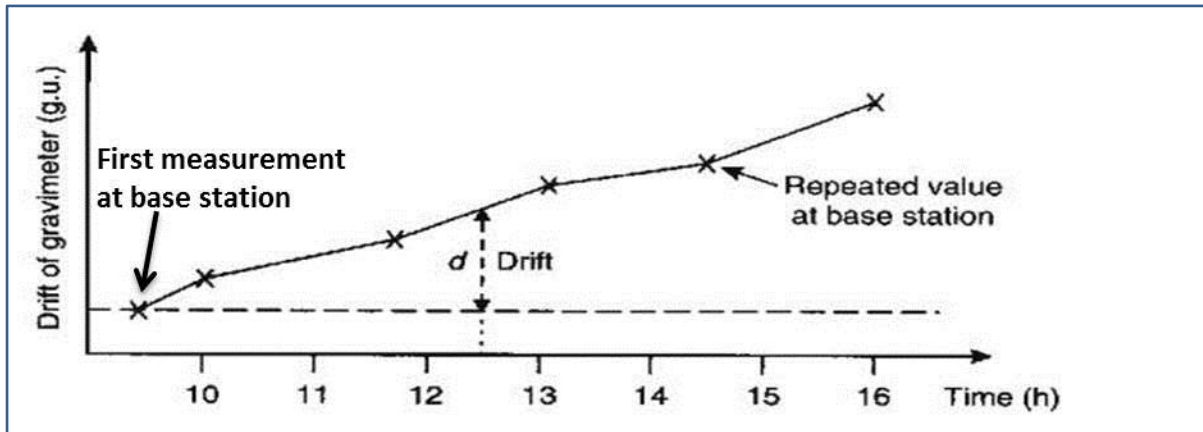
Figure C1 Graph of drift of gravimeter against time (Modified from Reeves, 2005).
