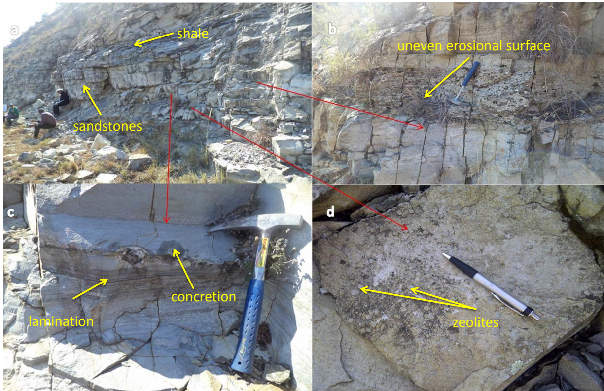
Figure 4.31 Photograph of the Katberg Formation, near Queenstown showing (a) Fine to medium grained, light grey sandstones with subordinate shale.(b) Uneven erosional surfaces. (c) Lamination and concretion (d) Zeolites.
