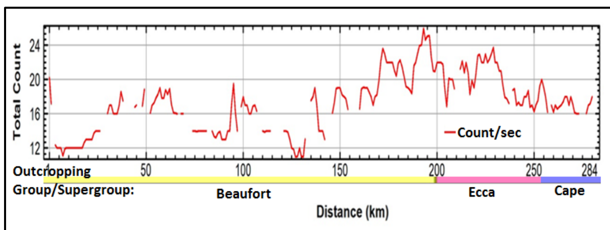
Figure 6.7 Profile for total gamma radiation count rate along Line C - C'.
