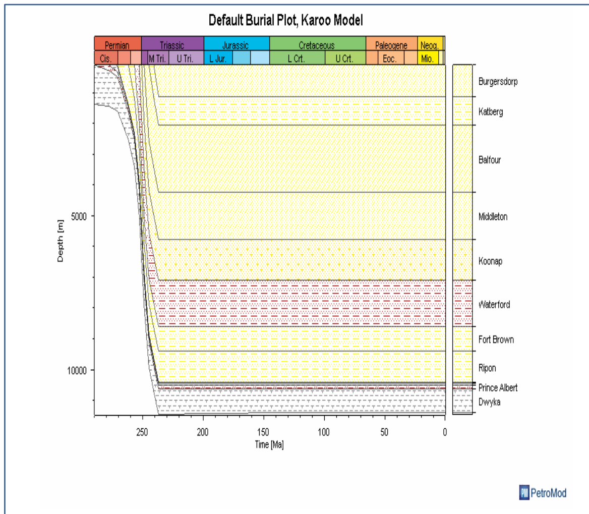
Figure 8.27 Burial history plot of the southeastern Karoo Basin.
