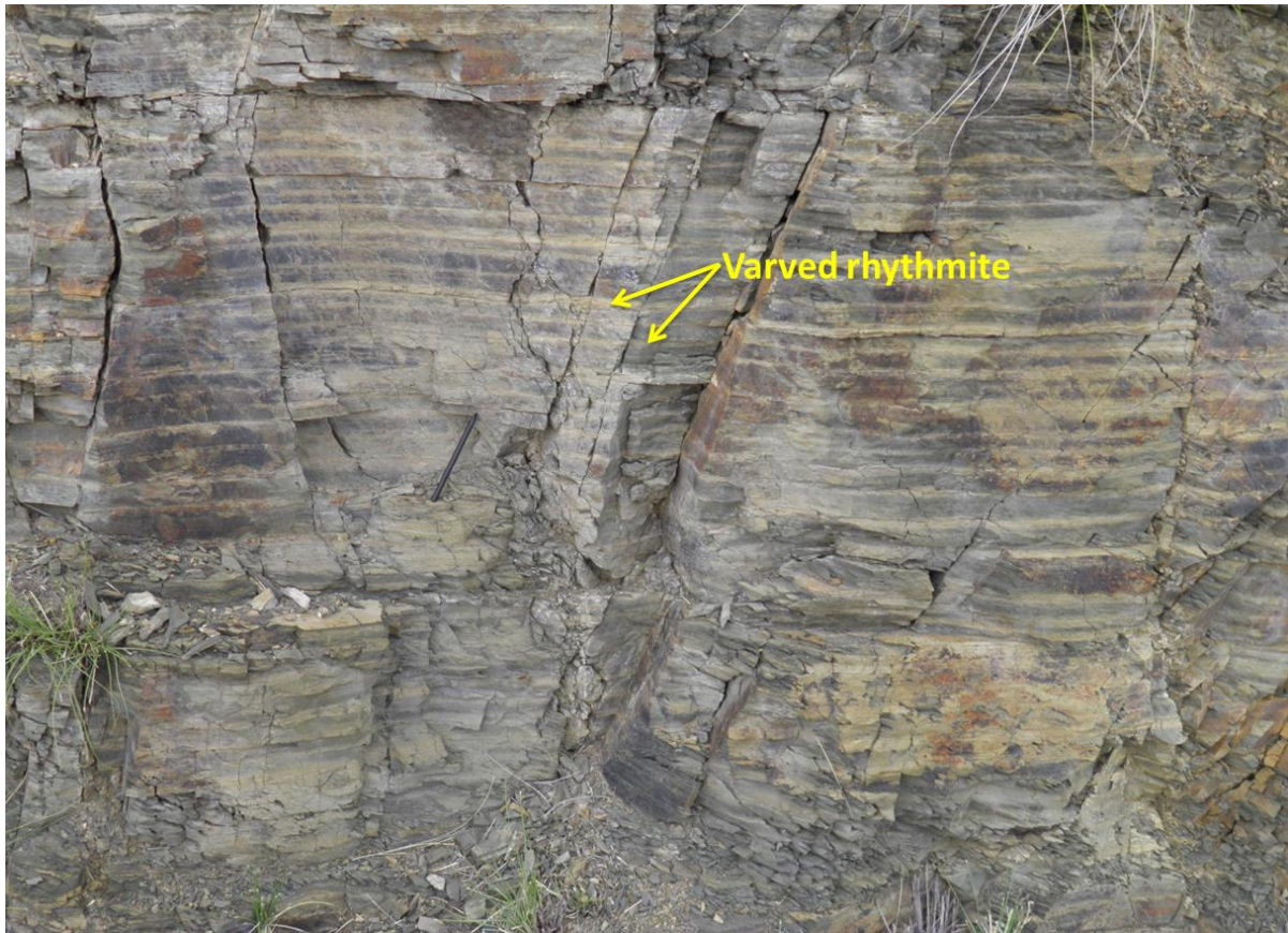
Figure 4.20 Varved rhythmite deposits of the Fort Brown Formation possibly of lacustrine origin. The photograph shows alternating light coloured mudstone and dark coloured mudstone, each with a centimetre thickness. The varves which are another kind of lamination can also be observed and the structures formed in a lacustrine environment with seasonal deposition of sediments. Whenever there was a high inflow of water, coarser sediments were also transported into the basin, whilst the finer sediments were deposited from suspension during periods when the water inflow was low.
