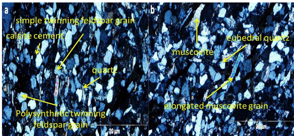
Figure 4.42 Photomicrographs of sandstones from Ripon Formation along Eccla Pass. (a) Calcite cement (dark colour), polysynthetic and simple twinning feldspar grains with zonation. (b) Concave and convex texture within the euhedral quartz grains and elongated muscovite grain with polysynthetic twinning.
