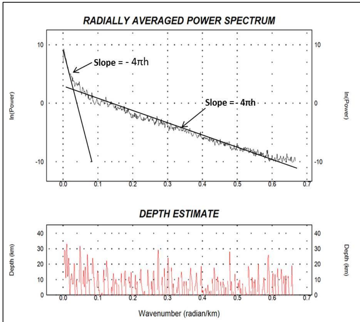
Figure 5.8 Radially averaged power spectrum of the aeromagnetic data of the study area.
