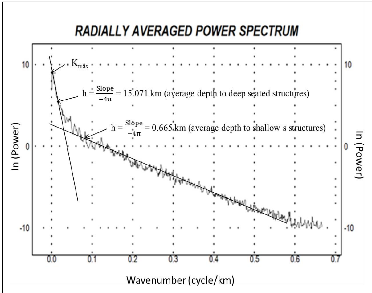
Figure 5.9 Depth estimate from the radially averaged power spectrum.
