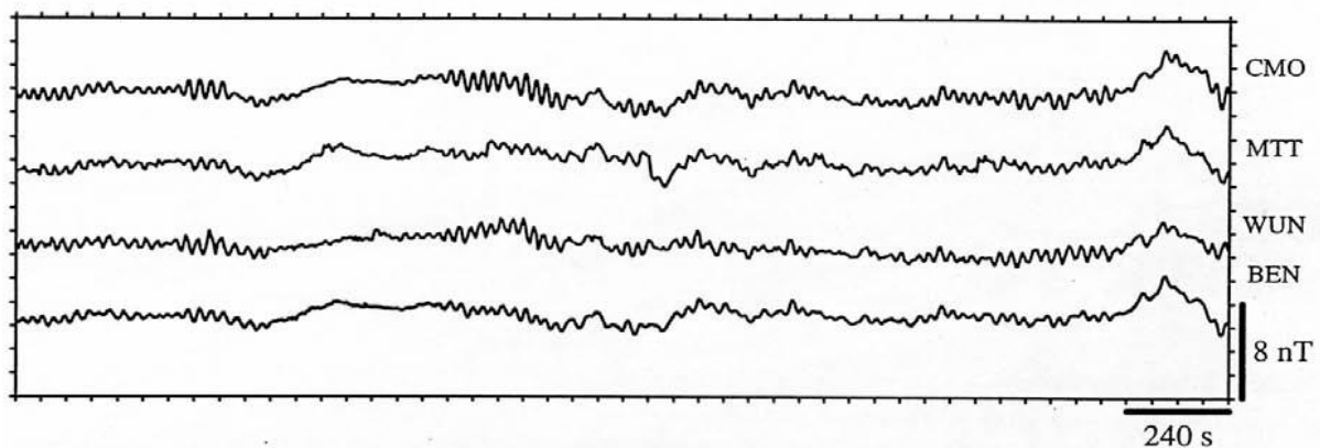
Figure B3 Micropulsations recorded at stations a few tens of kilometres apart (Reeves, 2005).
