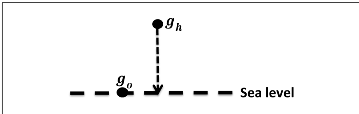
Figure C3 Schematic representation of free-air correction (Reeves, 2005).
