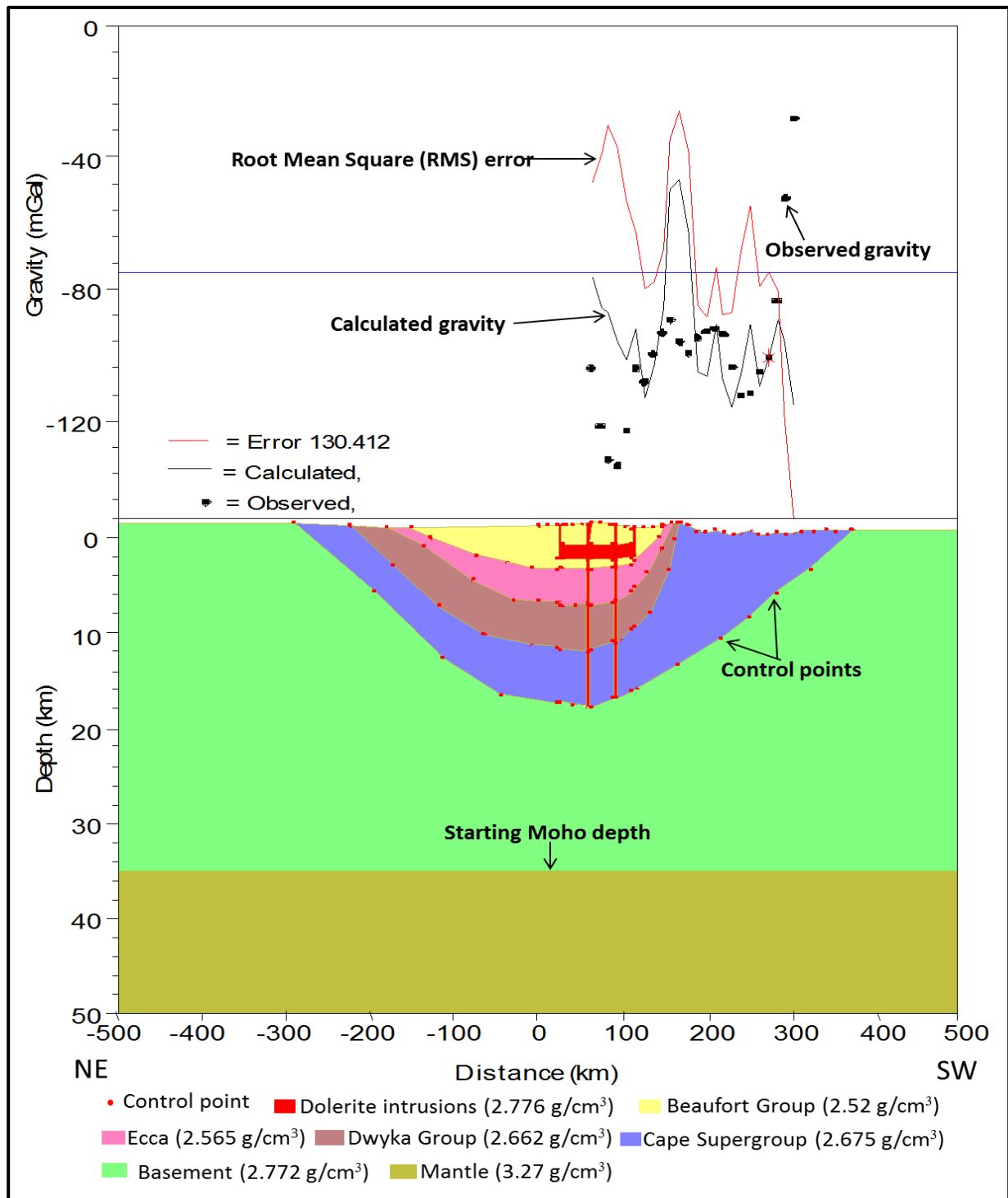
Figure 8.3 Starting model for profile A - A'. Vertical exaggeration (VE) = 5.75, Initial root mean square (RMS) error = 130.412 Note: When the black line/curve (calculated gravity) matches with the black dots (observed gravity), it indicates a perfect fit with minimum error. The modelled dolerite sills and dykes (presented in Figure 8.4 – 8.17) were originally set in horizontal and vertical positions, respectively and allowed to vary or change during the modelling process in order to have the best fit model.
