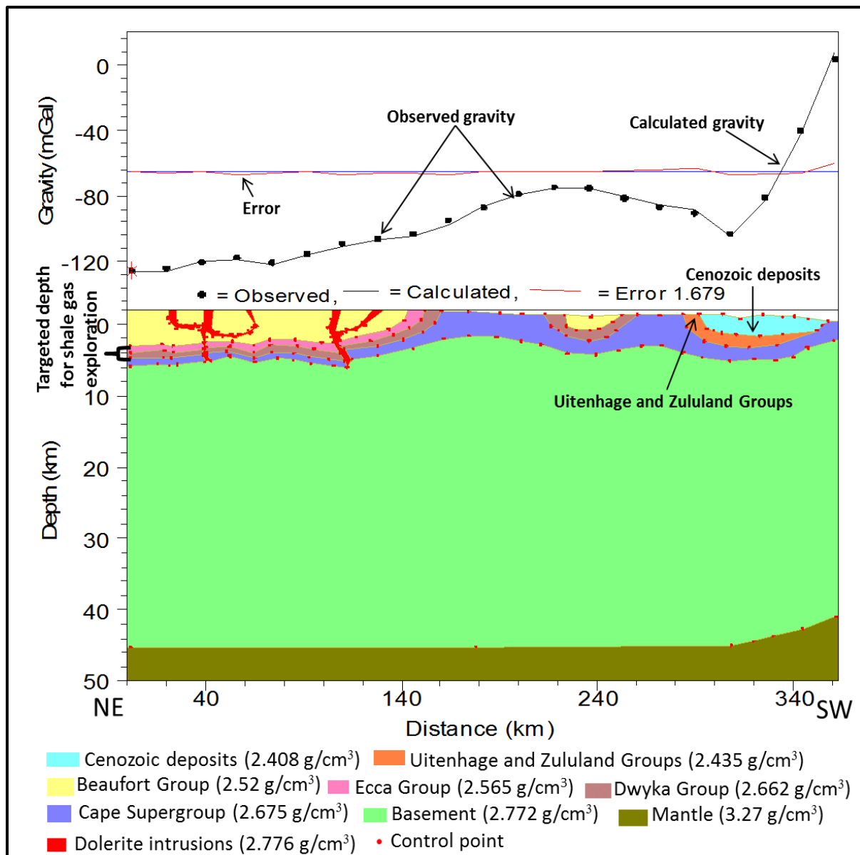
Figure 8.15 Gravity modelling of profile L – L'. VE = 2.27, Initial and final RMS errors are 148.036 and 1.679, respectively.
