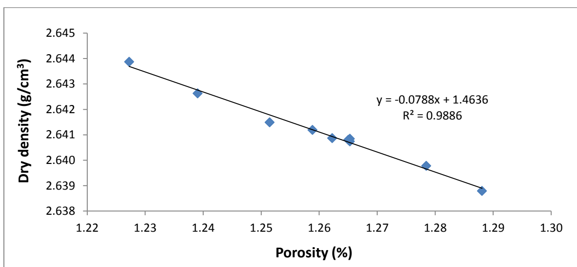
Figure C8 Dry density - porosity relationship for shale from the Prince Albert Formation.
