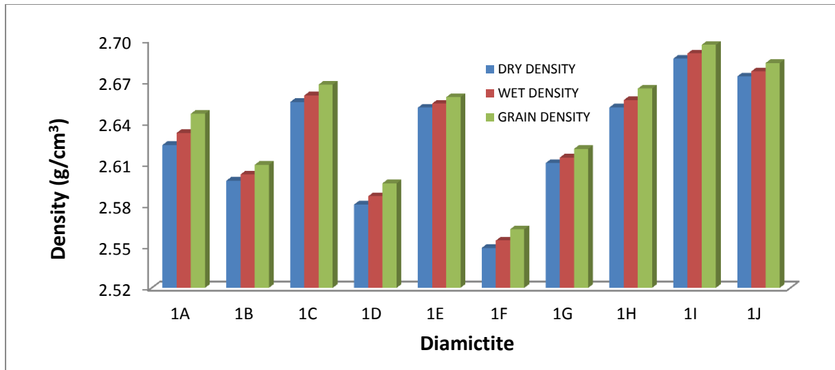
Figure C5 Bar chart of dry, wet and grain densities for the Dwyka diamictite.
