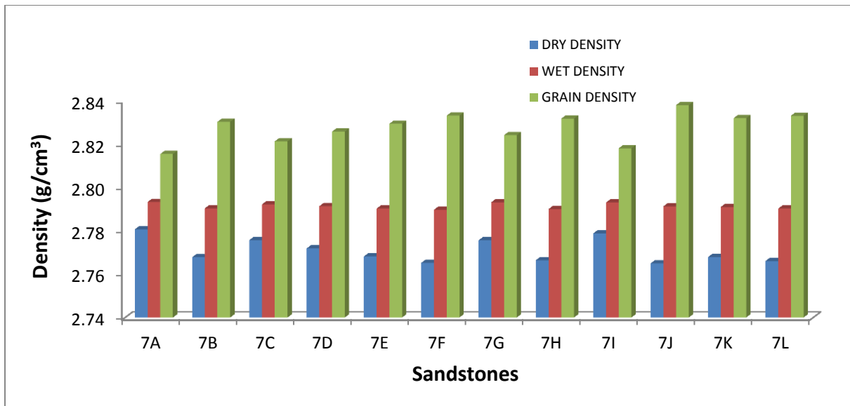
Figure C17 Bar chart of dry, wet and grain densities for the Koonap Formation.
