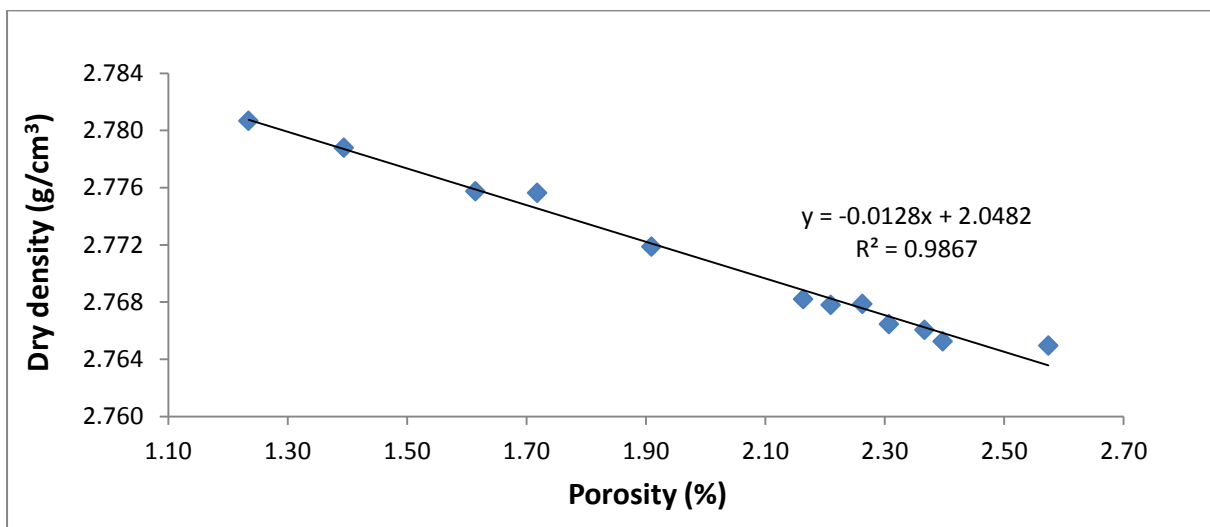
Figure C18 Dry density - porosity relationship for the Koonap Formation.
