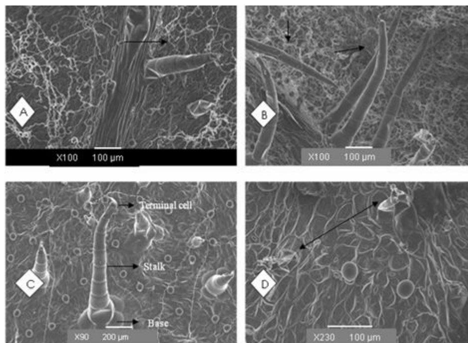
Figure 2. (A) Note the location of NGT on the midrib. (B) Distribution and arrangement of NGT and GTs on the midrib and leaf surfaces of A. arcuotoides . (C) Morphology of a NGT showing the terminal cell, the stalk and the base. (D) Glandular (GT) either collapsed naturally or during preparation for SEM.
