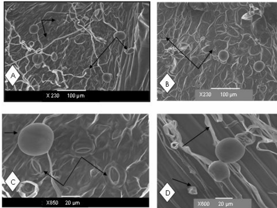
Figure 1. (A) Stomata and GTs distribution and their proximity on the abaxial and (B) Adaxial surfaces of A. arcuotoides . (C) Magnified view of the globular head of GT and stomata pores on the abaxial surface. (D) Crystal deposit and connection of GTs with fibre-ends of NGTs.
