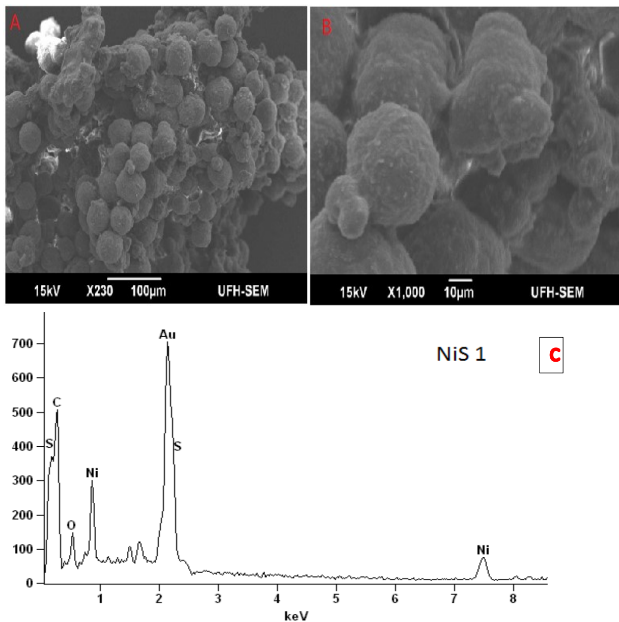
Figure 4.10: SEM micrograph of the NiS1 from \text{Ni}(\text{L}^4)_2 complex (A) low magnification, (B) high magnification and (C) EDX spectrum of the sample.
