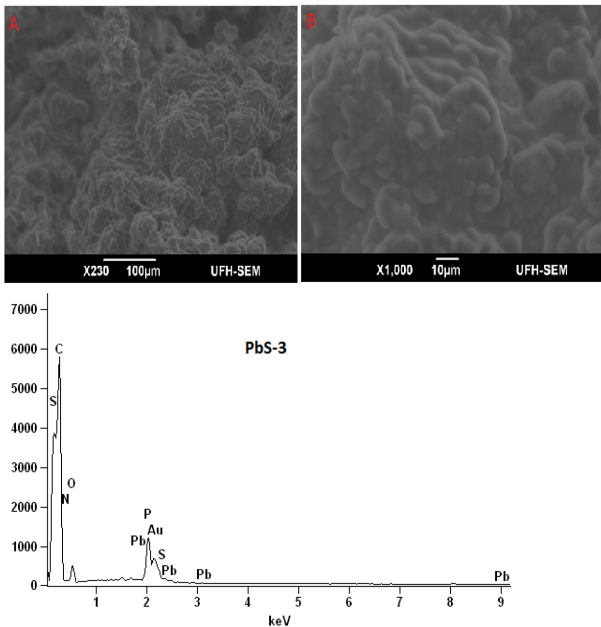
Figure 4.15: SEM micrograph of the PbS3 from \text{Pb}(\text{L}^5)_2 complex (A) low magnification, (B) high magnification and (C) EDX spectrum of the sample.
