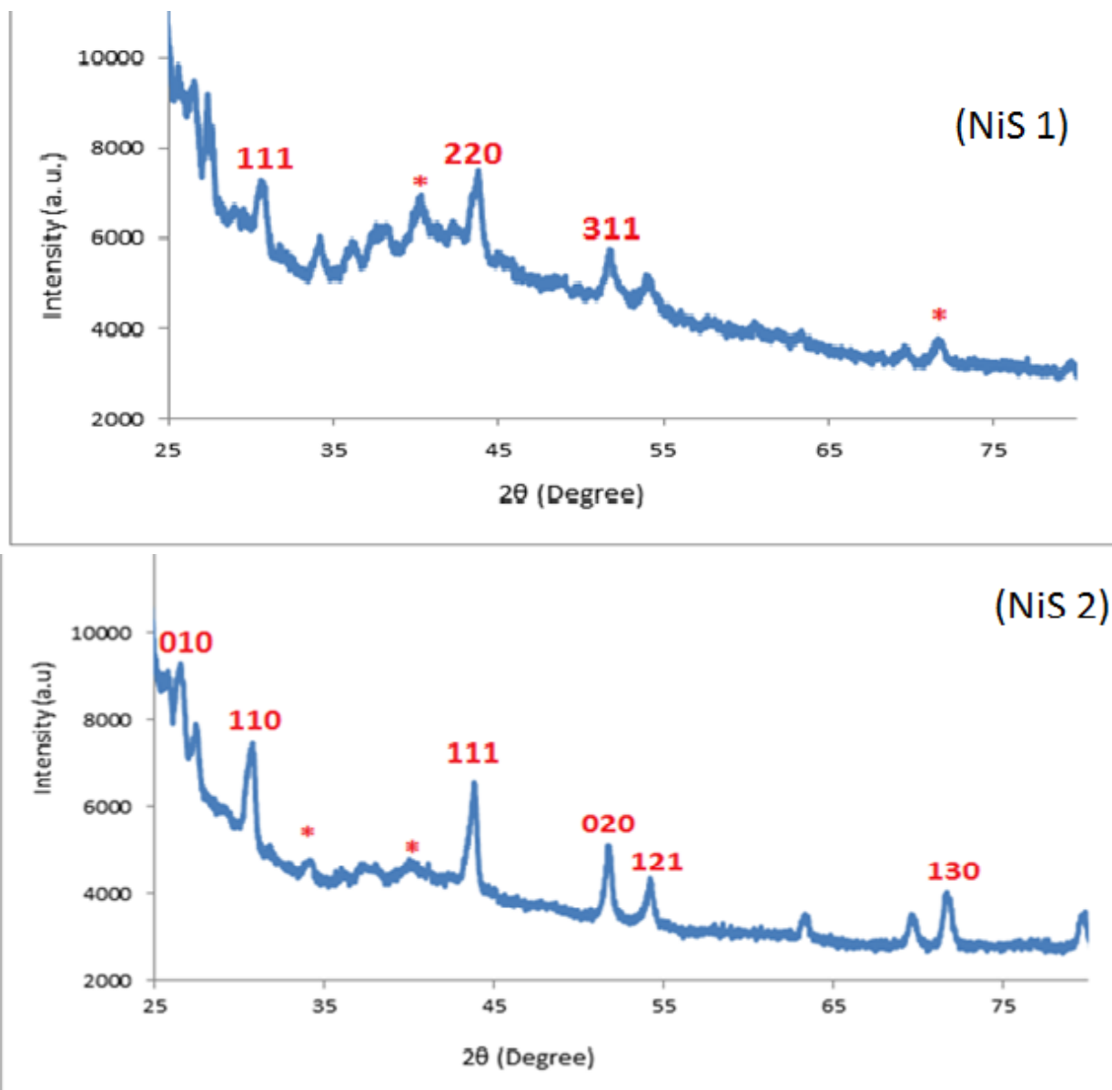
Figure 4.3: The XRD patterns of NiS1 and NiS2 nanoparticles synthesized from \text{Ni}(\text{L}^4)_2 and \text{Ni}(\text{L}^1)_2 complexes.
