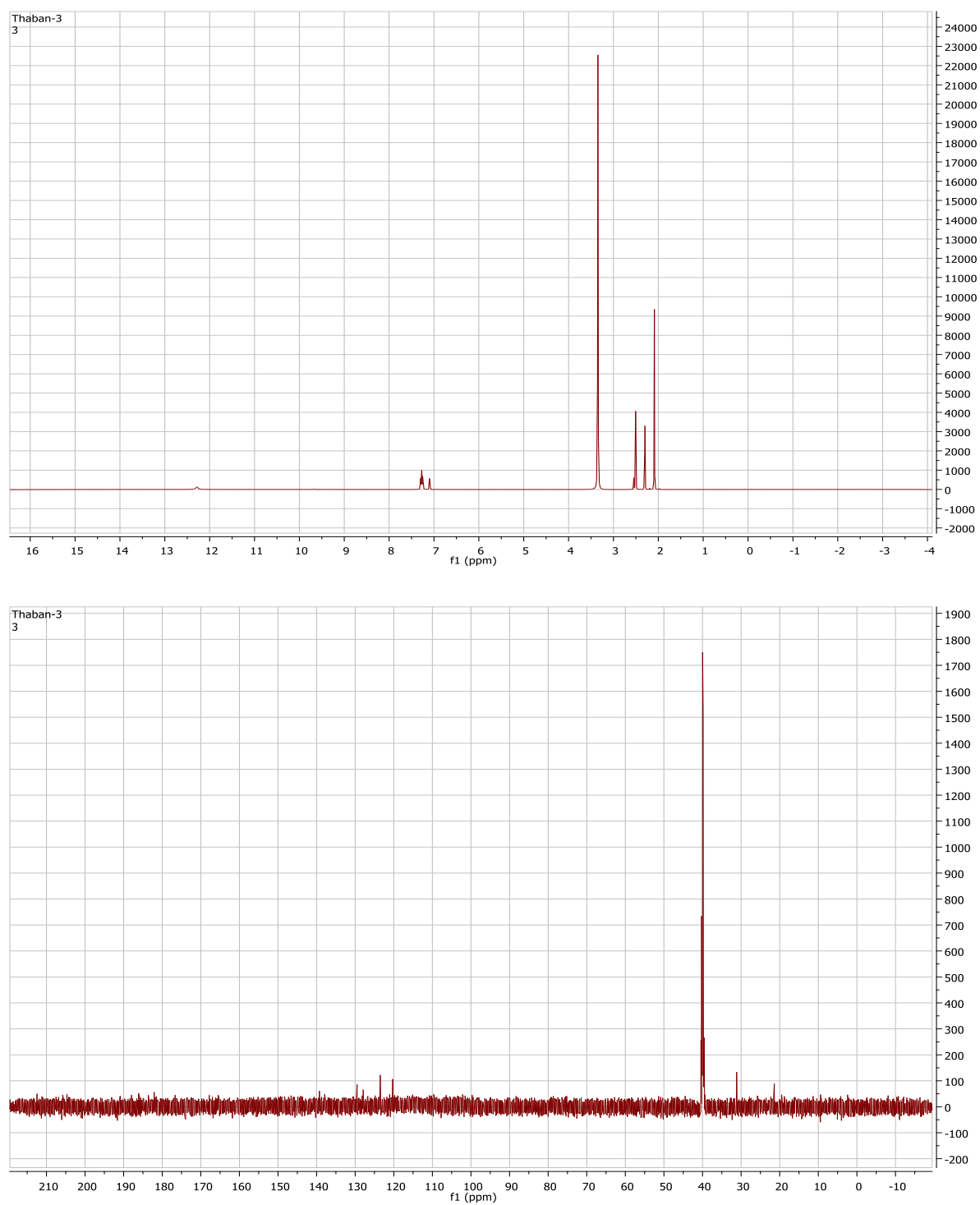
Figure 5.16: ^1\text{H} and ^{13}\text{C} -NMR spectra of Ni(II) bis(3-methyldithiocarbamate) complex
