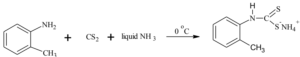
Scheme 2: Reaction equation for the synthesis of ammonium 2-methyl-N-phenyldithiocarbamate ligand \text{NH}_4 [(\text{CH}_3)\text{C}_6\text{H}_5\text{NHCS}_2] .
