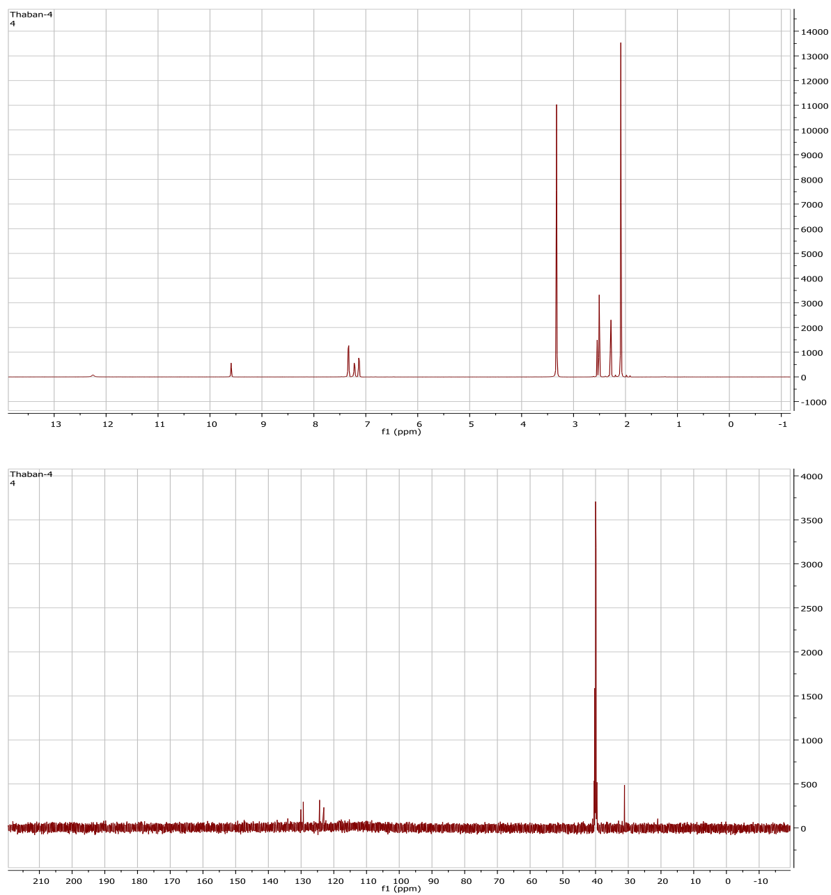
Figure 5.17: ^1\text{H} and ^{13}\text{C} -NMR spectra of Ni(II) bis(4-methyl-N-phenyldithiocarbamate) complex
