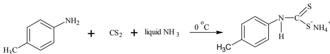
Scheme 4: Reaction equation for the synthesis of 4-methyl-N-phenyldithiocarbamate ligand NH 4 [(CH 3 )C 6 H 5 NHCS 2 ]
