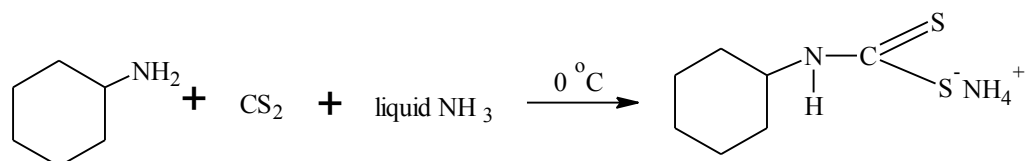
Scheme 6: Reaction equation for the synthesis of cyclohexyldithiocarbamate ligand ( \text{NH}_4 [\text{C}_6\text{H}_{11}\text{NHCS}_2] ).
