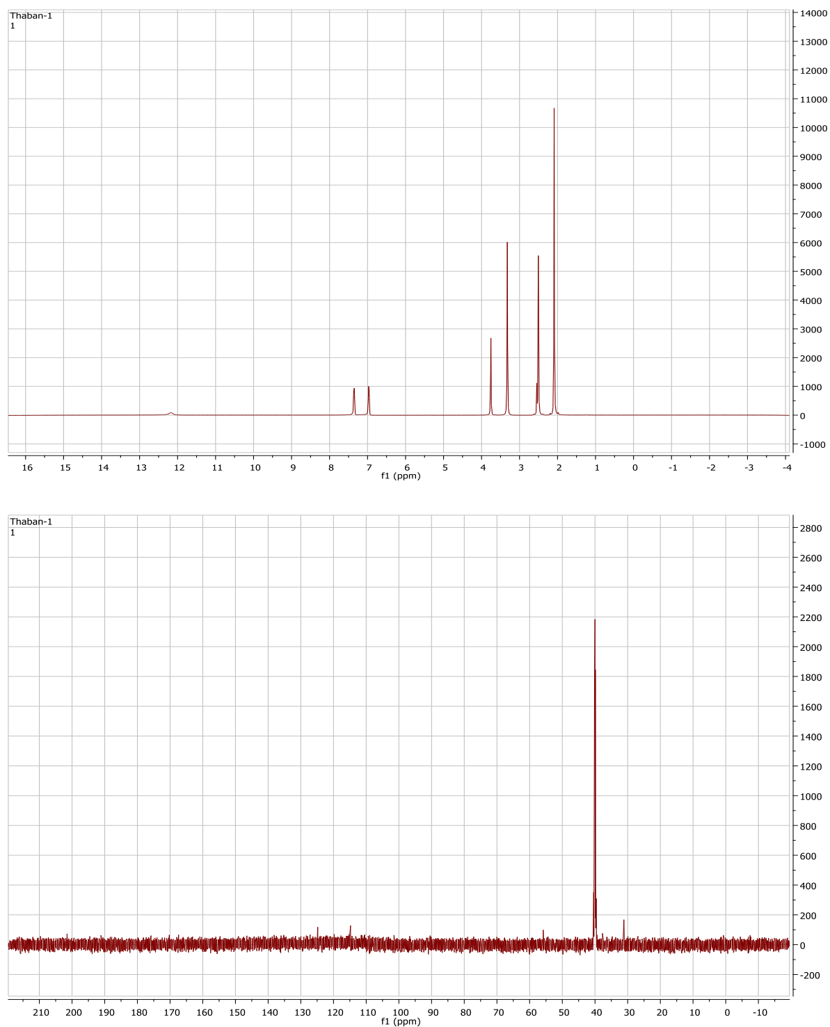
Figure 5.18: ^1\text{H} and ^{13}\text{C} -NMR spectra of Ni(II) bis(4-methoxy-N-phenyldithiocarbamate) complex
