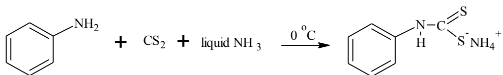
Scheme 1: Reaction equation for the synthesis of ammonium N-phenyldithiocarbamate ligand \text{NH}_4 [\text{C}_6\text{H}_5\text{NHCS}_2] .
