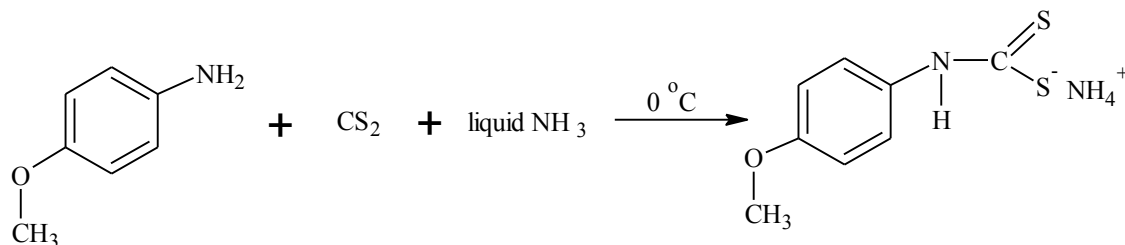
Scheme 5: Reaction equation for the synthesis of 4-methoxy-N-phenyldithiocarbamate ligand \text{NH}_4 [(\text{OCH}_3)\text{C}_6\text{H}_5\text{NHCS}_2] .
