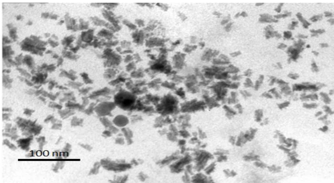
Figure 4.7: TEM image o HDA capped PbS1 nanoparticles prepared from \text{Pb}(\text{L}^4)_2
