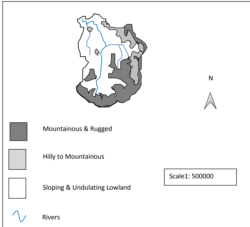
Figure 3.2 Sterkspruit catchment: relief features
