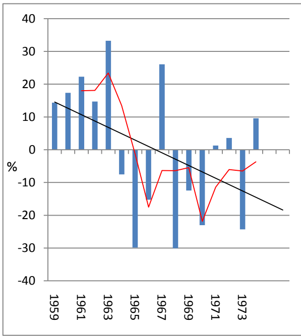
Figure 5.14 Deviations from mean annual rainfall, Sterkspruit: 1959-1974.
