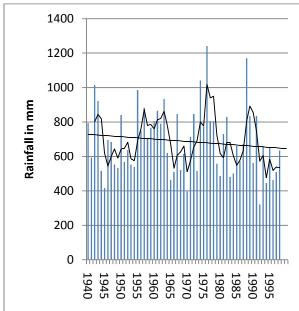
Figure 5.7a Mean annual rainfall at SterkspruitTNK: 1940-1998
