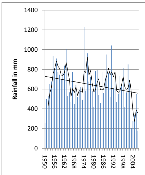
Figure 5.11a Mean annual rainfall, Lady Grey: 1950-2006
