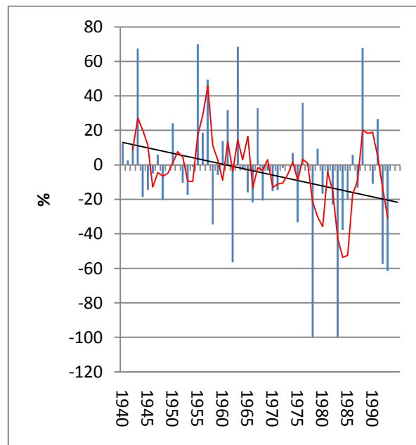
Figure 5.16 Deviations from mean annual rainfall, Bensonvale: 1940-1993
