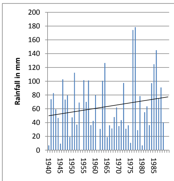
Figure 5.20 SterkspruitTNK, October rainfall: 1940-1989
