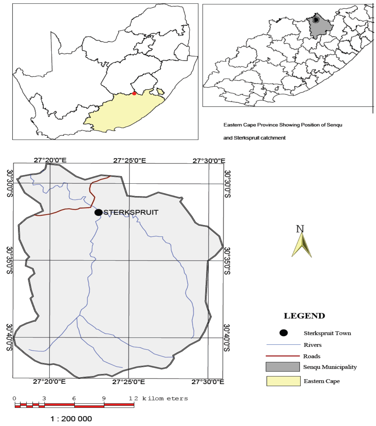
Figure 1 The study area: Sterkspruit catchment, showing its position in the Eastern Cape province and in South Africa
