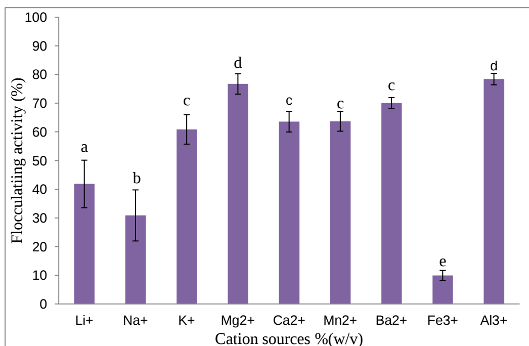
Figure 3.9: Effect of cations on the flocculating activity of purified bioflocculant produced by Halomonas sp. Okoh. Flocculating activities with different letters are significantly different ( P < 0.05 ) from each other.
