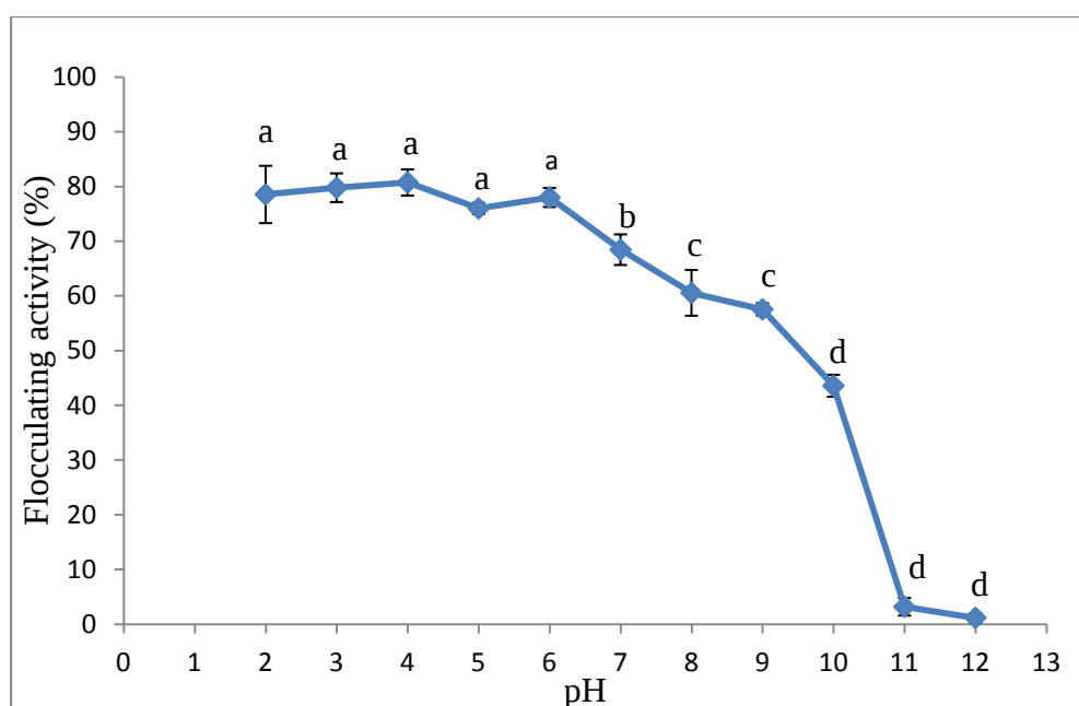
Figure 4.9: Effect of pH on the flocculating activity of the purified bioflocculant produced by Micrococcus sp. Leo. Flocculating activities with different letters are significantly different ( P < 0.05 ) from each other.
