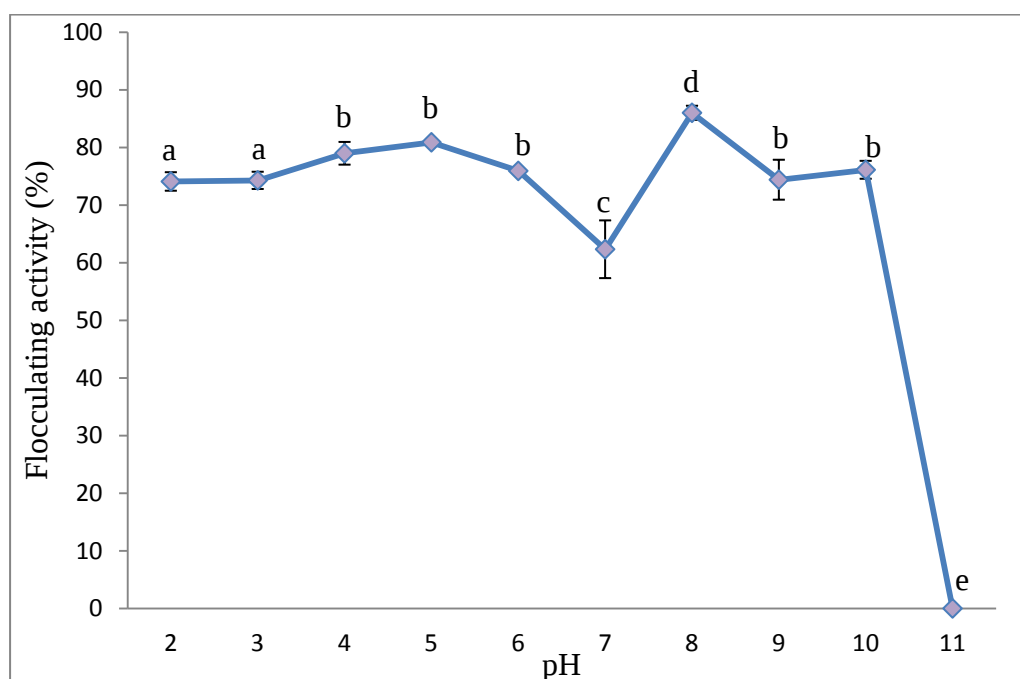
Figure 5.6: Effect of pH on the flocculating activity of the biofloculant produced by a consortium ( Halomonas sp. Okoh and Micrococcus sp. Leo). Flocculating activities with different letters are significantly different ( P < 0.05 ) from each other.
