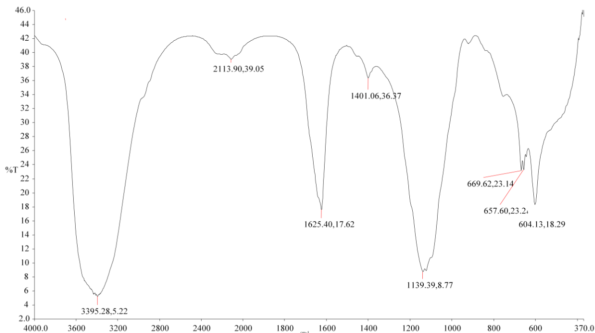
Figure 5.8: Fourier transform intrared (FTIR) spectroscopy of the purified biofloculant
