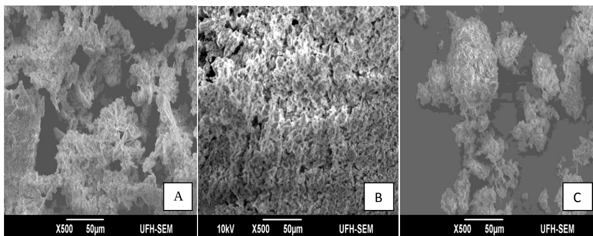
Figure 5.9: SEM images of purified bioflocculant A, Kaolin particles B and Kaolin particles flocculated with bioflocculant.
