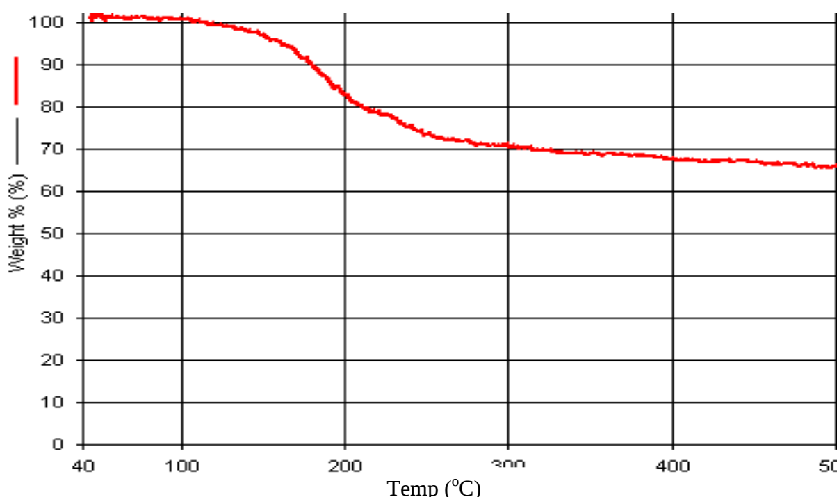
Figure 3.13: Thermo gravimetric analyses of purified bioflocculant produced by Halonomas sp. Okoh.
