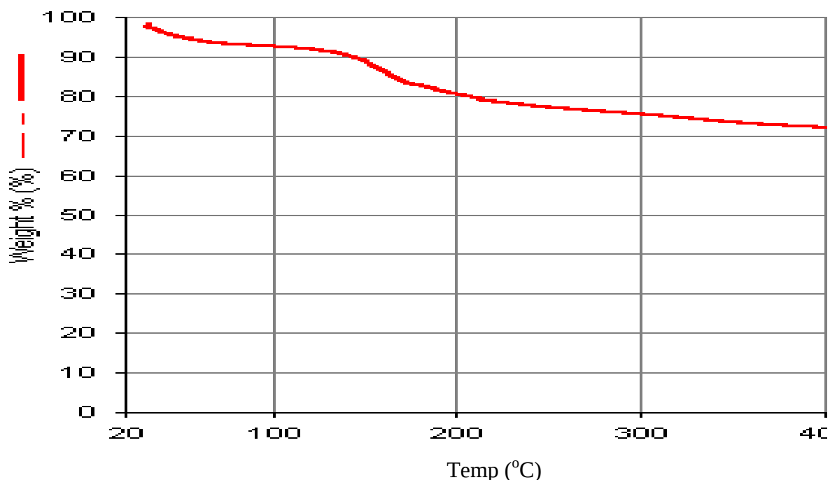
Figure 5.7: Thermogravimetric analyses of the purified biofloculant
