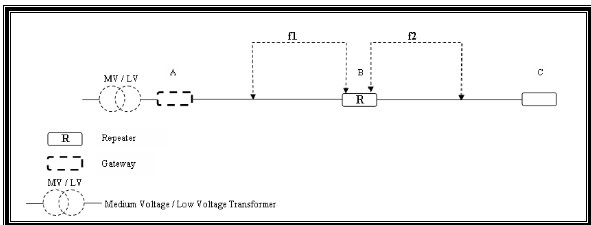
Figure 3.7: Frequency Division (FD) Repeater
