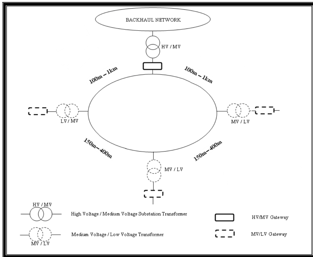
Figure 3.10: Proposed Medium PLC Ring Network Topology
