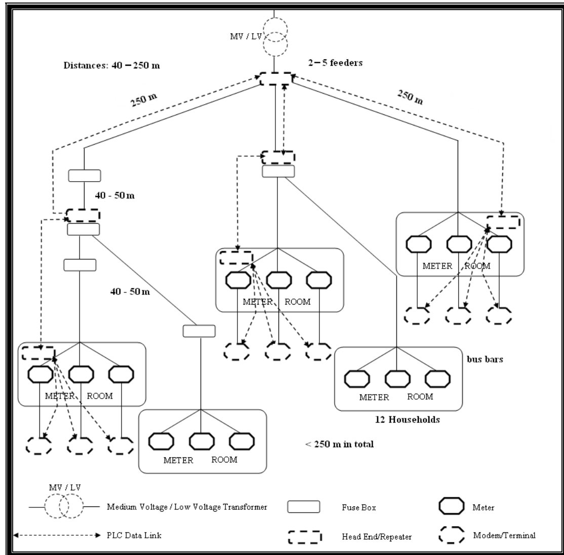
Figure 3.14: Proposed Local PLC Topology Architecture Third Model
