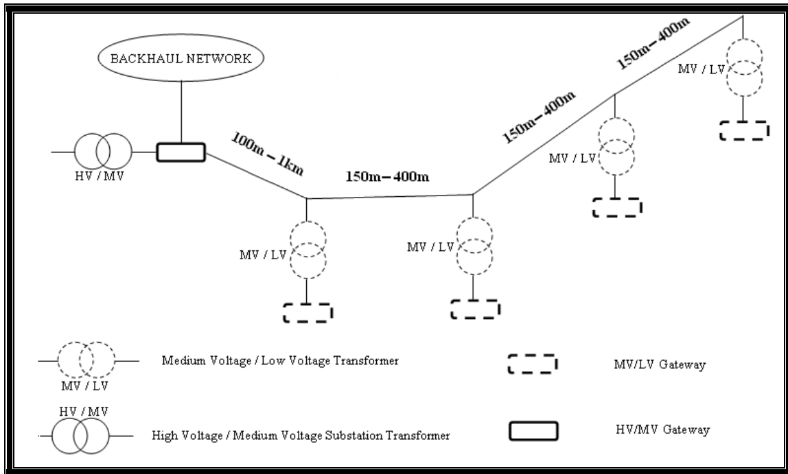
Figure 3.8: Proposed Medium PLC Bus Network Topology
