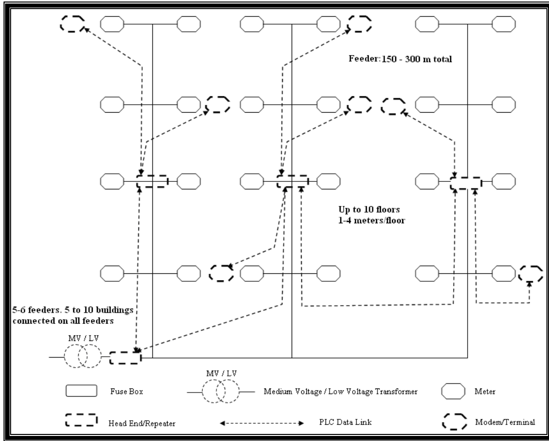
Figure 3.15: Proposed Local PLC Topology Architecture Fourth Model
