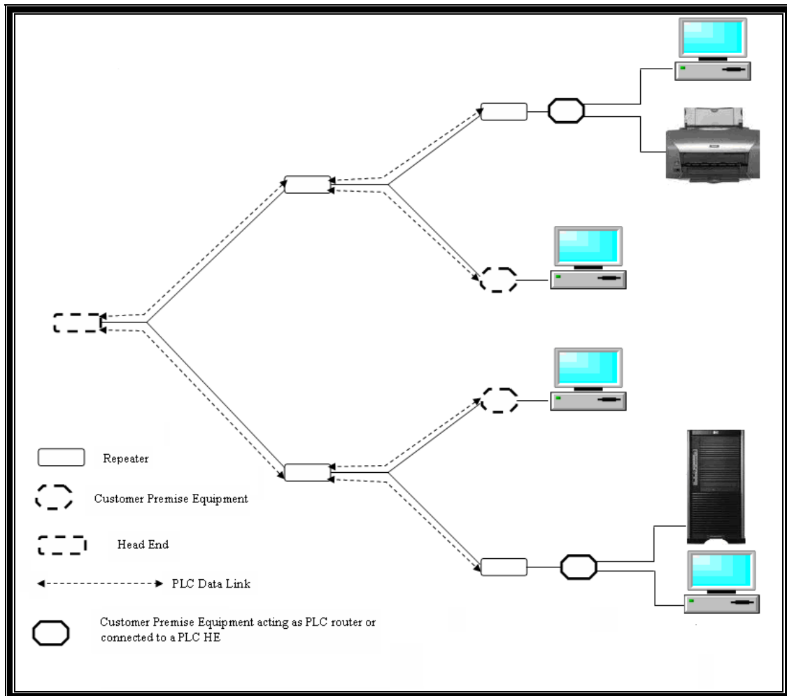
Figure 3.18: Proposed PLC Topology Model for a Hybrid Set-Up
