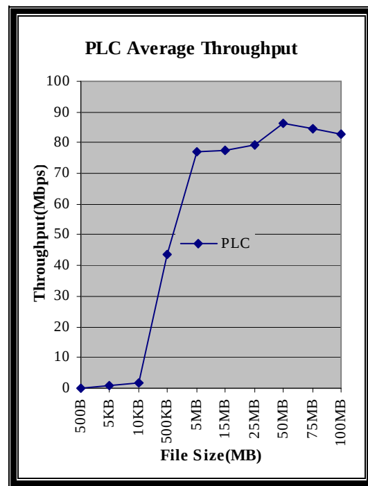
Figure 5.4: PLC Average Throughput
