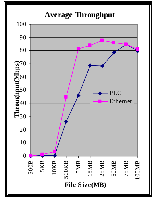
Figure 5.11: PLC and Ethernet Average Throughput
