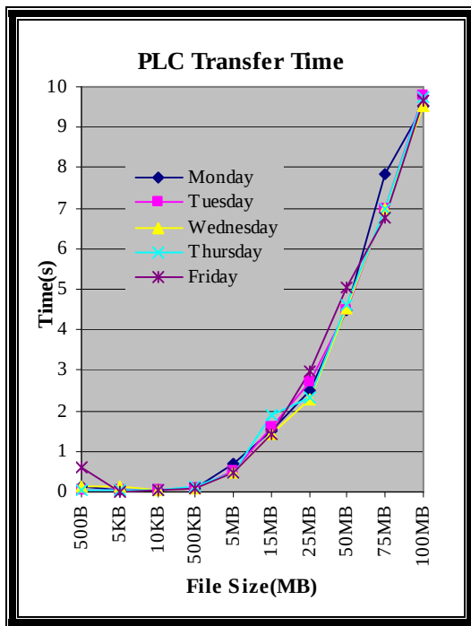
Figure 5.1: Broadband PLC Transfer Time
