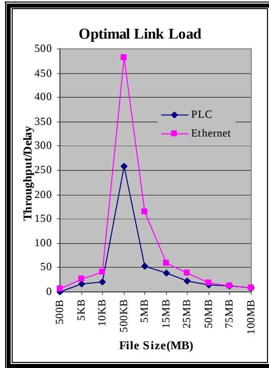
Figure 5.12: PLC and Ethernet Optimal Load
