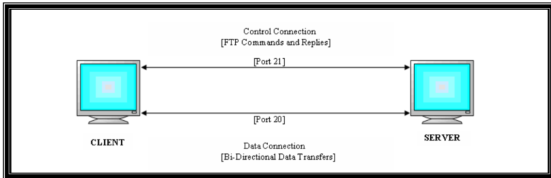
Figure 4.2: A typical FTP Client/Server Scenario.
