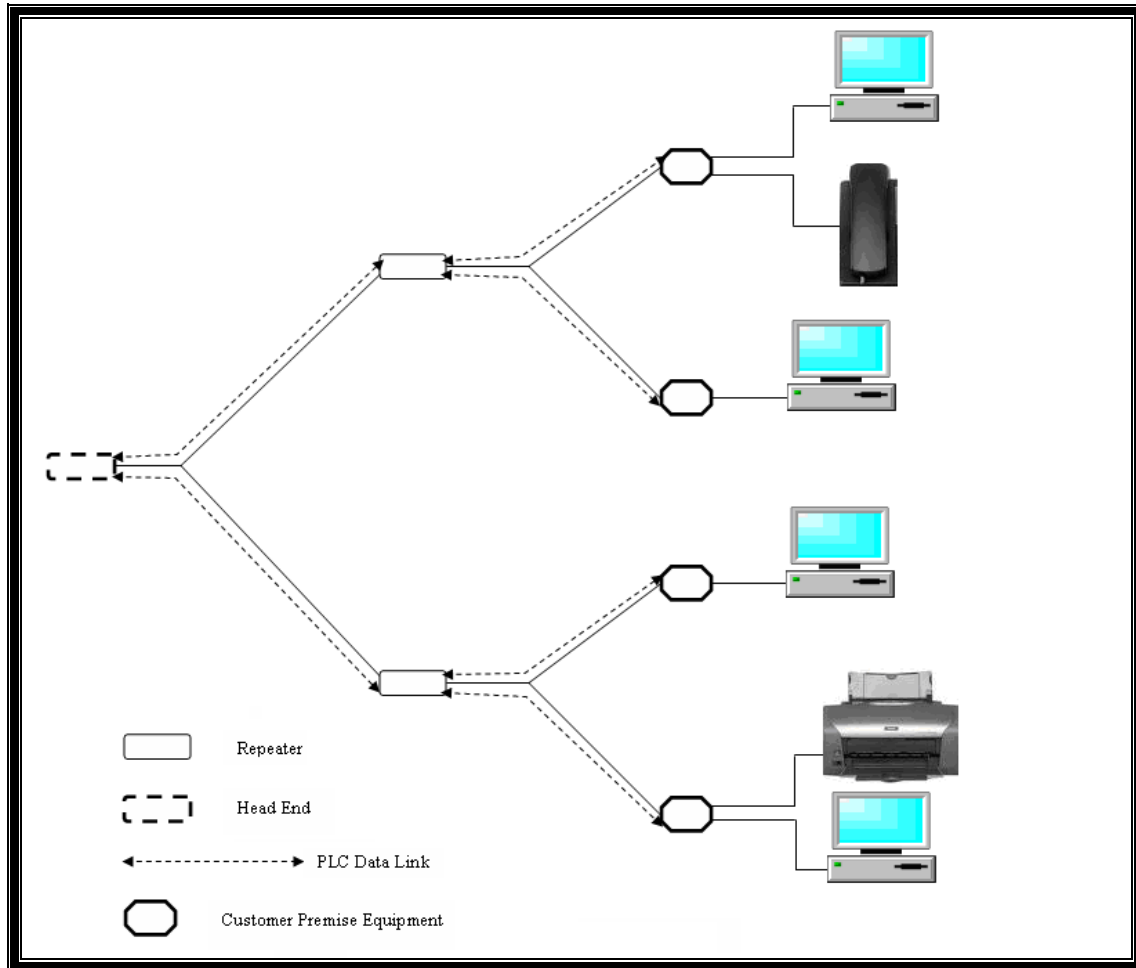
Figure 3.16: Proposed PLC Topology Model for Home End Users
