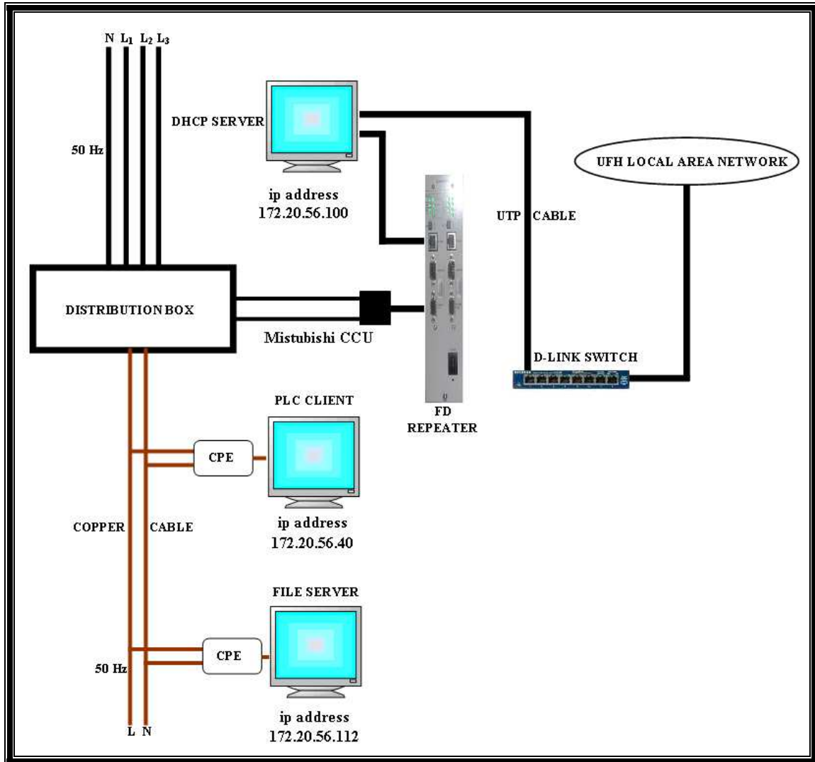
Figure 4. 8: Experiment One: Laboratory Data Transfer Configuration.
