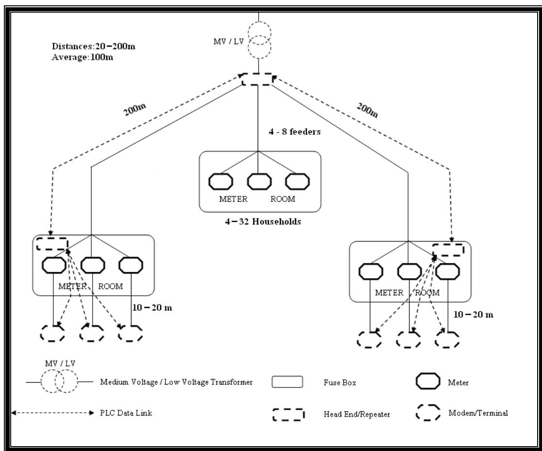
Figure 3.13: Proposed Local PLC Topology Architecture Second Model
