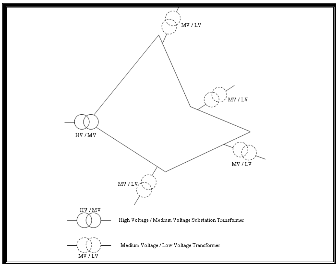
Figure 3.4: Ring Topology
