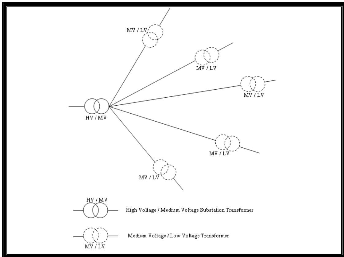
Figure 3.1: Radial Topology with Exclusive MV lines
