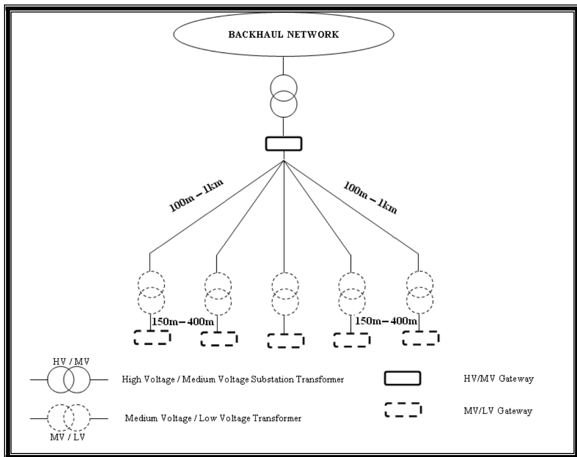
Figure 3.9: Proposed Medium PLC Star Network Topology
