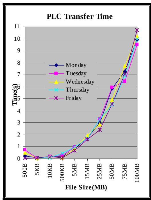
Figure 5.6: PLC Node Transfer Time
