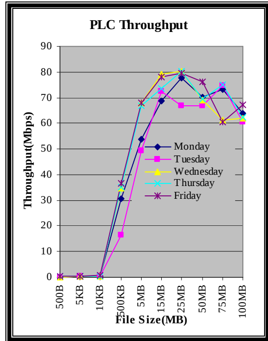
Figure 5.14: Broadband PLC Throughput
