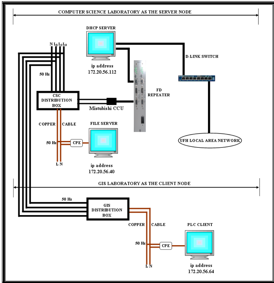
Figure 4.10: Experiment Three: Multibuilding Data Transfer Configuration.
