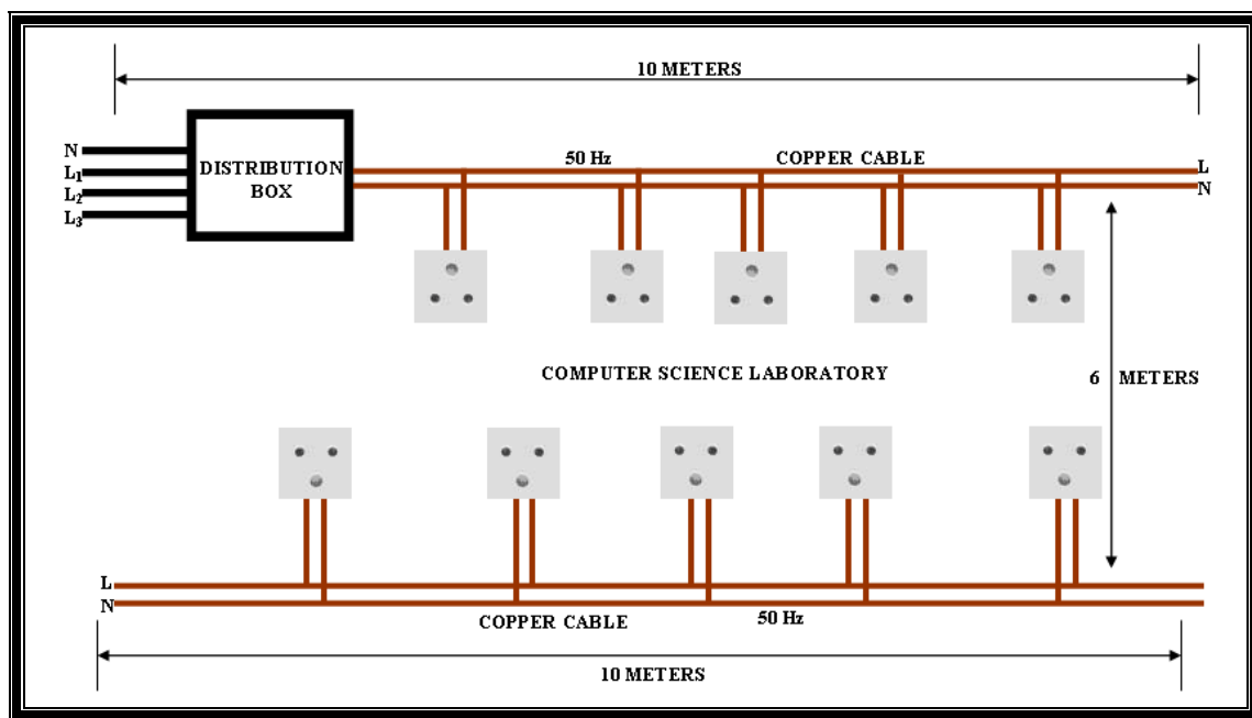
Figure 4.1: Diagram showing CSC Laboratory Layout.
