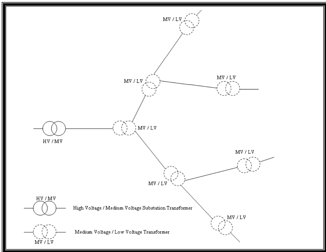
Figure 3.3: Radial Topology with Tree-shaped line
