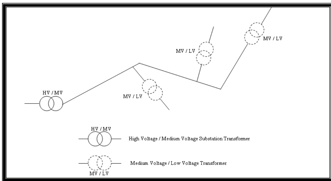
Figure 3.2: Radial Topology with Single MV line
