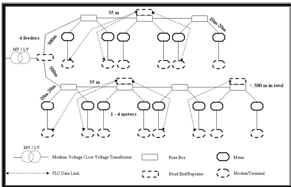
Figure 3.12: Proposed Local PLC Topology Architecture First Model
