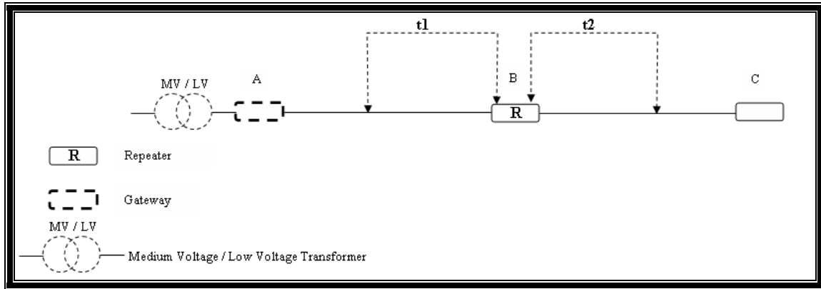
Figure 3.6: Time Division (TD) Repeater [Hrasnica et al 04]
