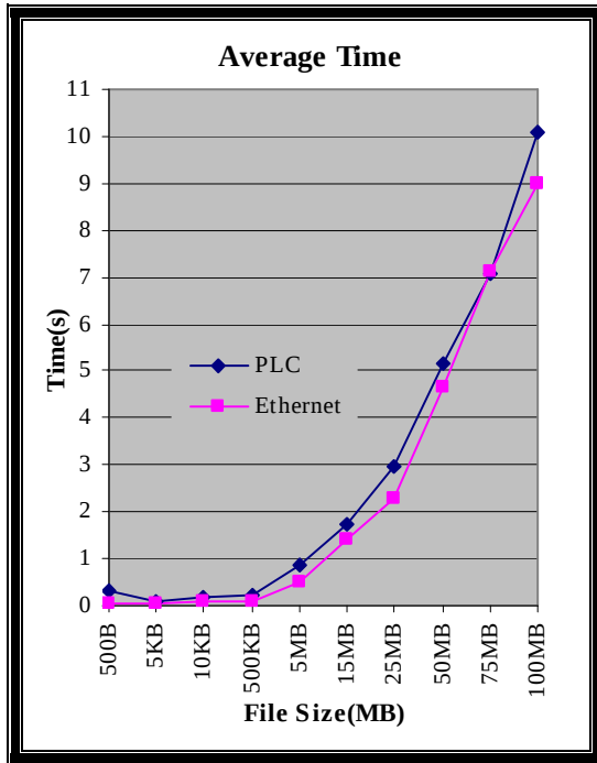
Figure 5.10: Broadband PLC and Ethernet Average Transfer Time
