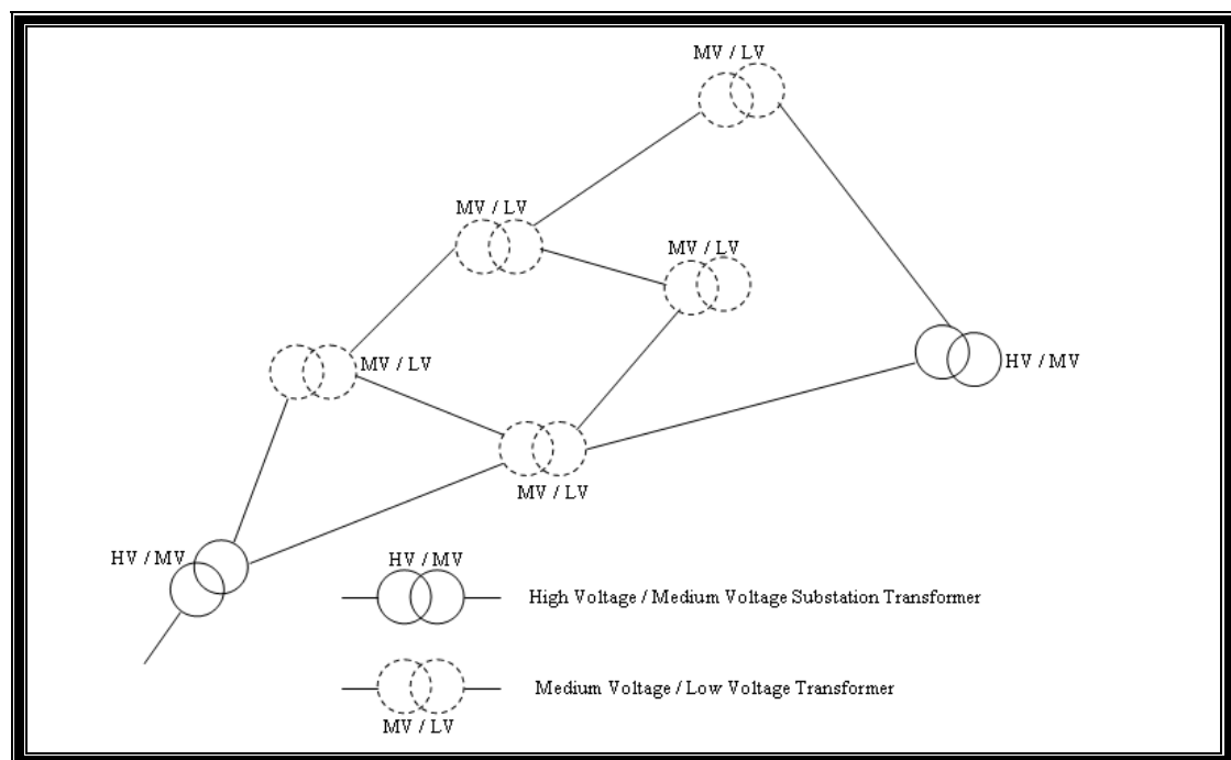
Figure 3.5: Networked Topology
