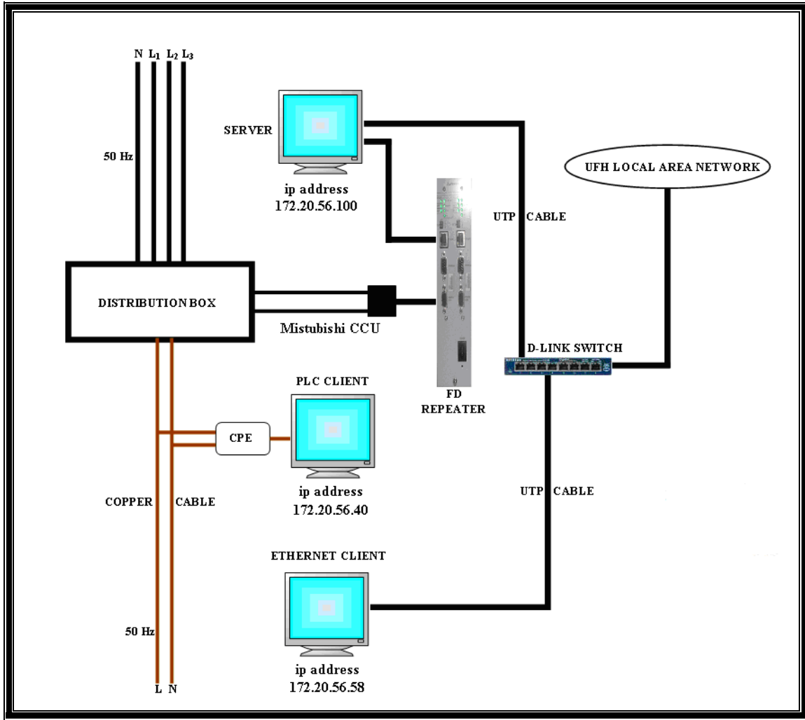
Figure 4. 9: Experiment Two: Laboratory Data Transfer Configuration.
