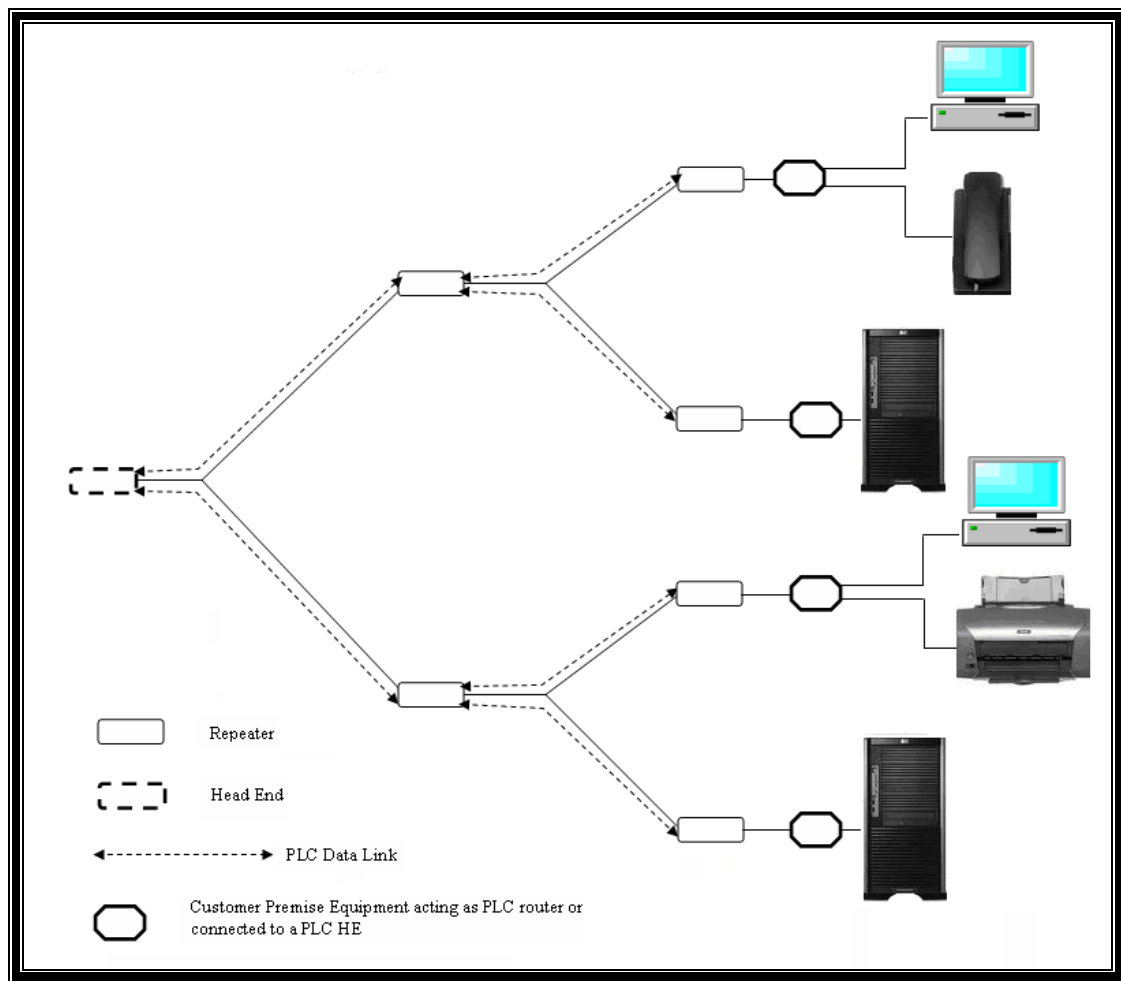
Figure 3.17: Proposed PLC Topology Model for Office End Users
