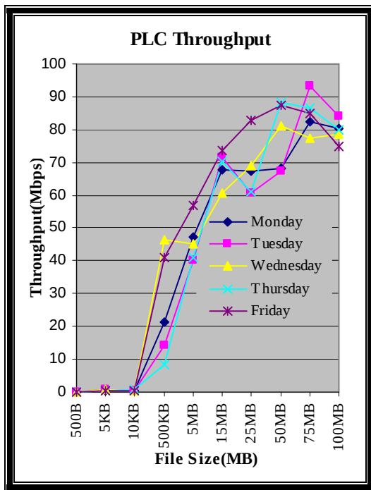
Figure 5.8: Broadband PLC Throughput
