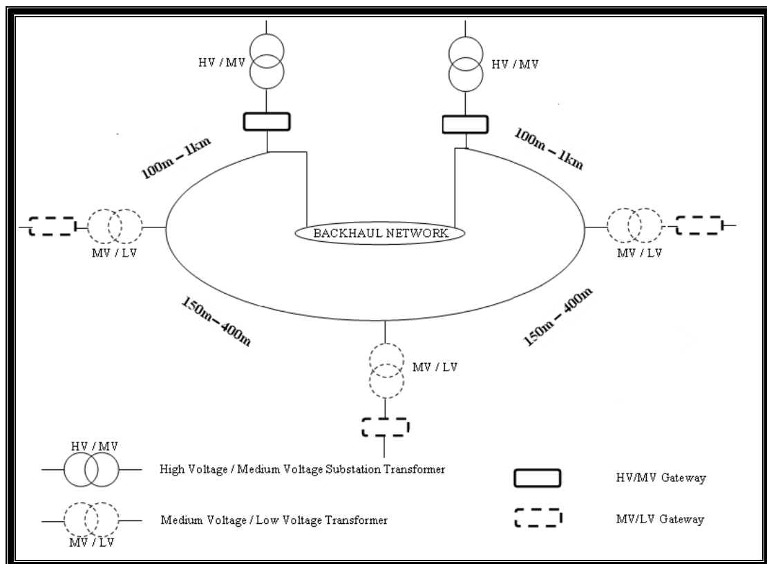
Figure 3.11: Proposed Medium PLC Partial Ring Network Topology
