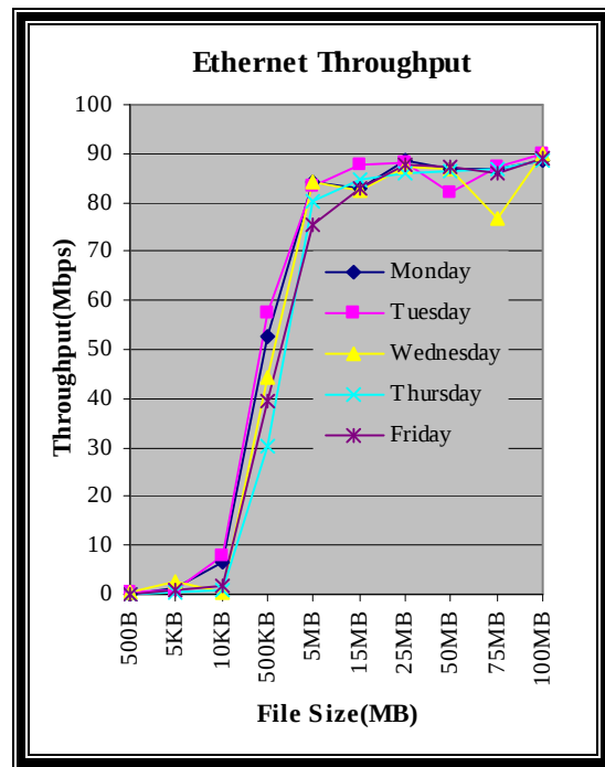
Figure 5.9: Ethernet Throughput
