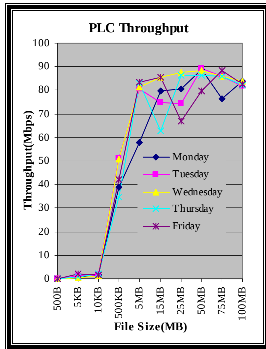
Figure 5.2: Broadband PLC Throughput.
